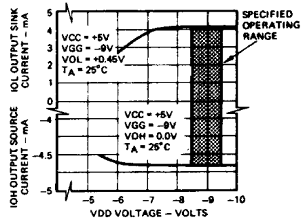
Output Current Versus VDD Supply Voltage
