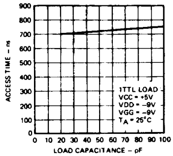
Access Time Versus Load Capacitance
