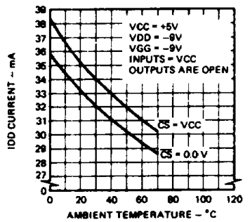
IDD Current Versus Temperature
