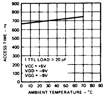
Access Time Versus Temperature
