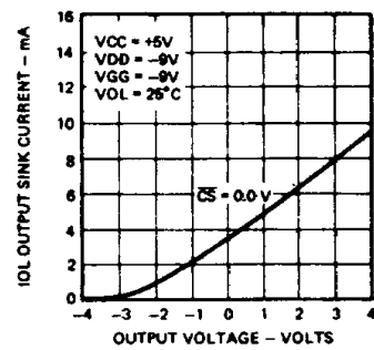
Output Sink Current Versus Output Voltage
