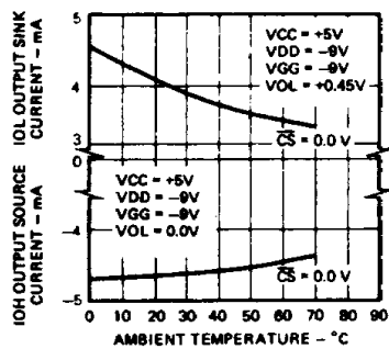
Output Current Versus Temperature
