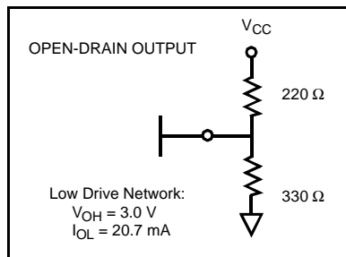
Figure 5. Connection Recommendations for Low Current Drive Network
