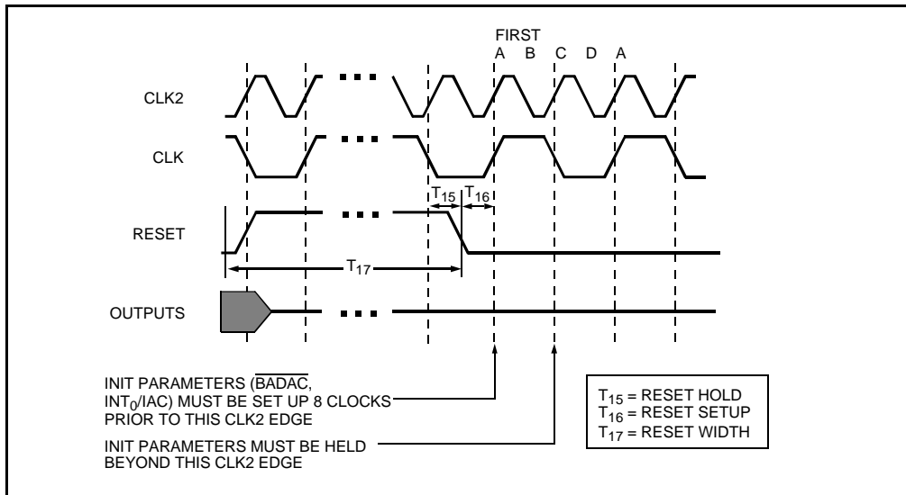
Figure 16. RESET Signal Timing
