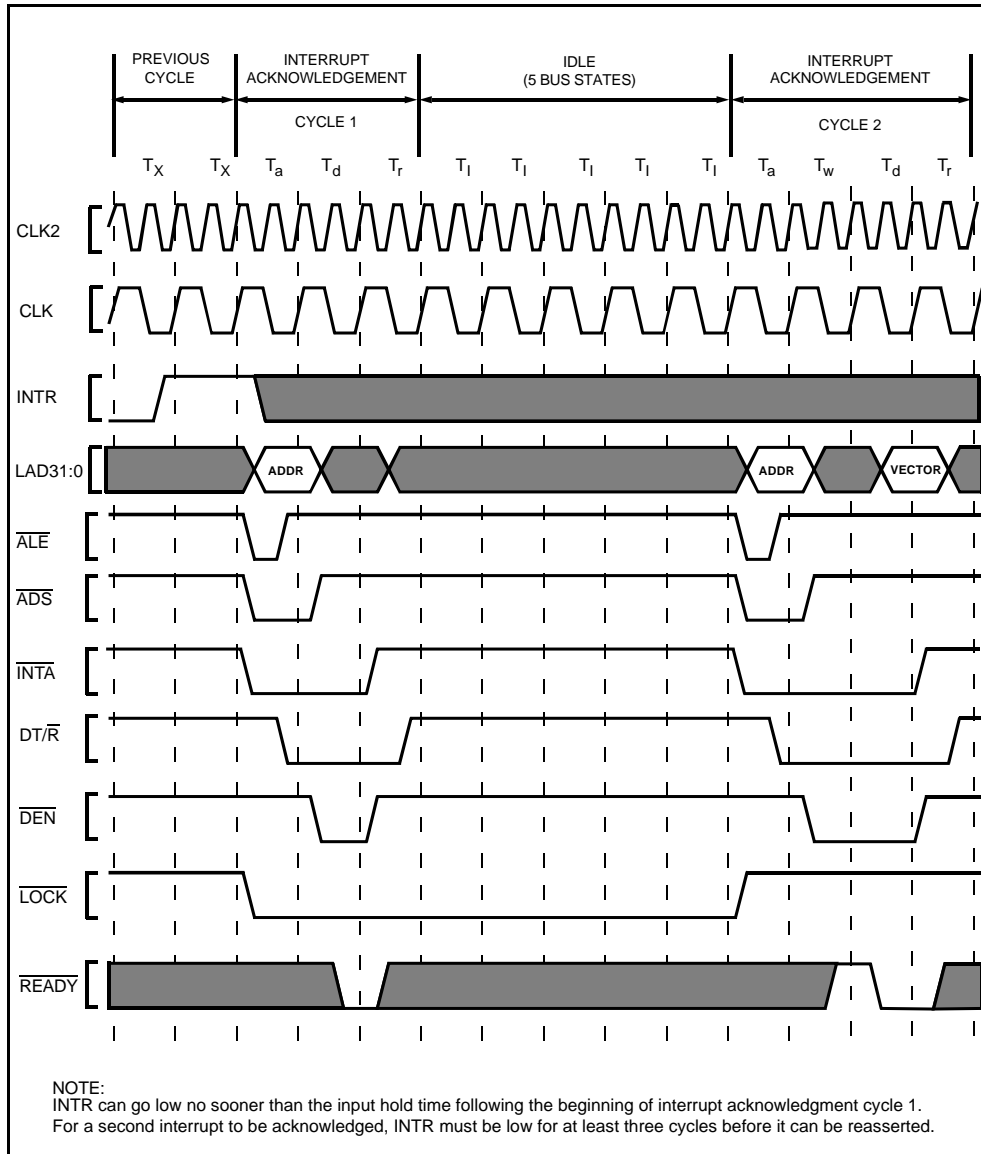
Figure 31. Interrupt Acknowledge Transaction
