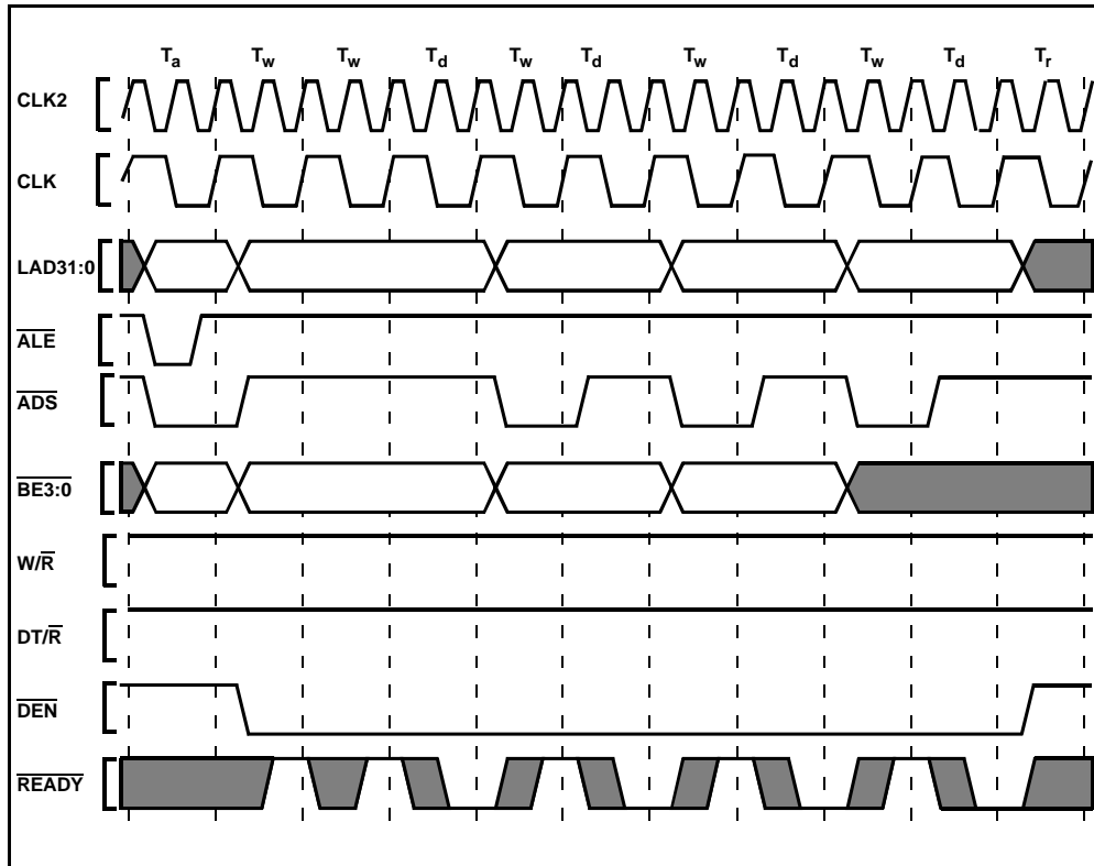
Figure 29. Burst Write Transaction with 2, 1, 1, 1 Wait States
