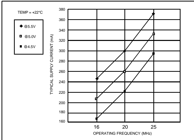
Figure 9. Typical Current vs. Frequency (Hot Temp)
