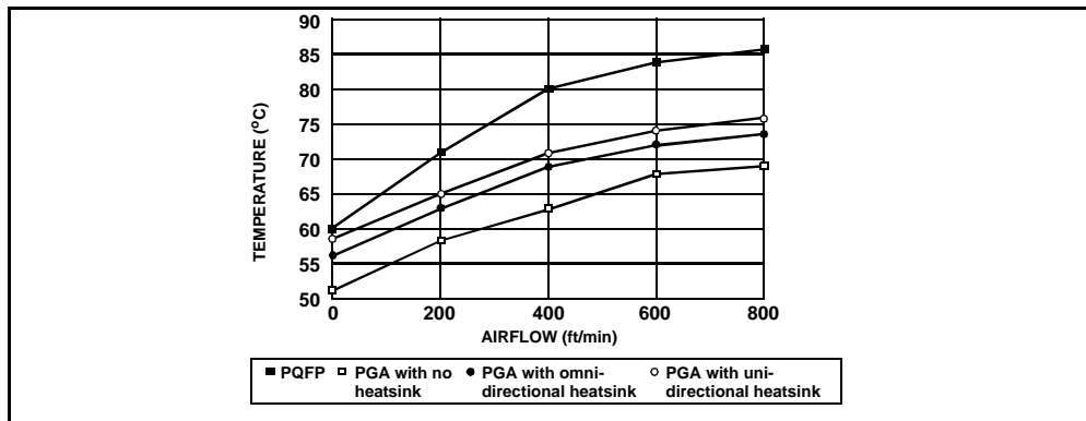
Figure 24. 20 MHz Maximum Allowable Ambient Temperature
