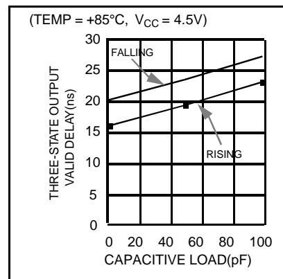
Figure 11. Capacitive Derating Curve
