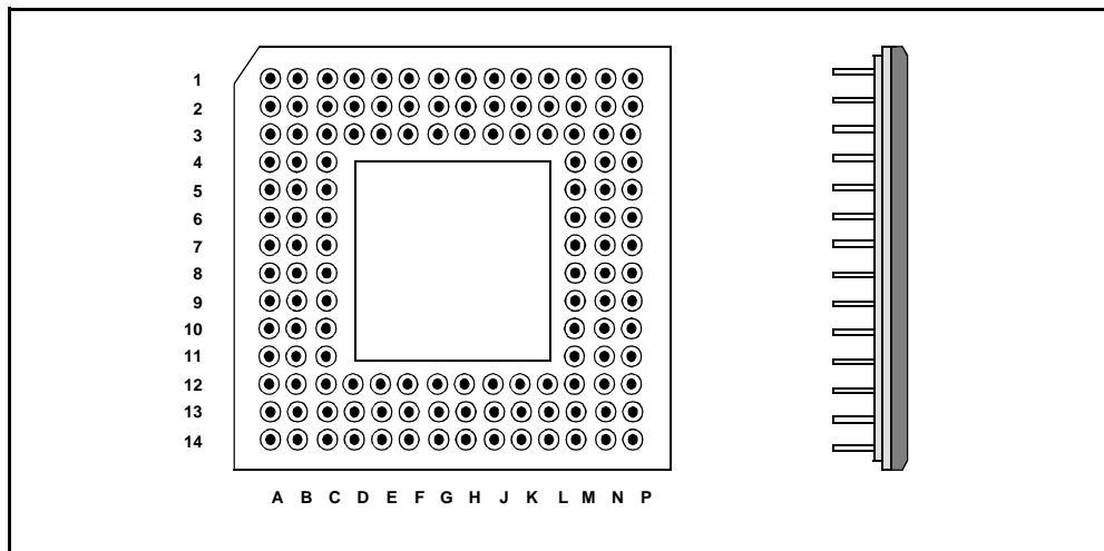
Figure 17. 132-Lead Pin-Grid Array (PGA) Package
