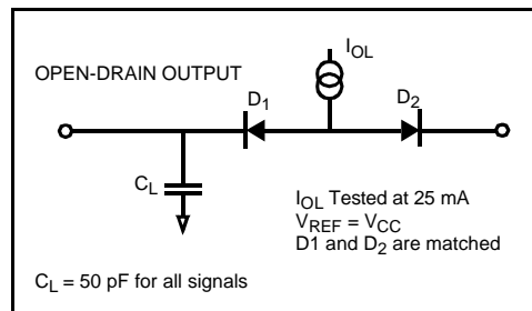
Figure 13. Test Load Circuit for Open-Drain Output Pins
