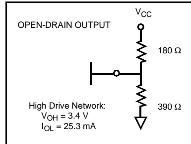
Figure 6. Connection Recommendations for High Current Drive Network
