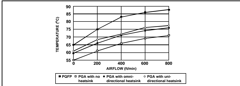
Figure 23. 16 MHz Maximum Allowable Ambient Temperature
