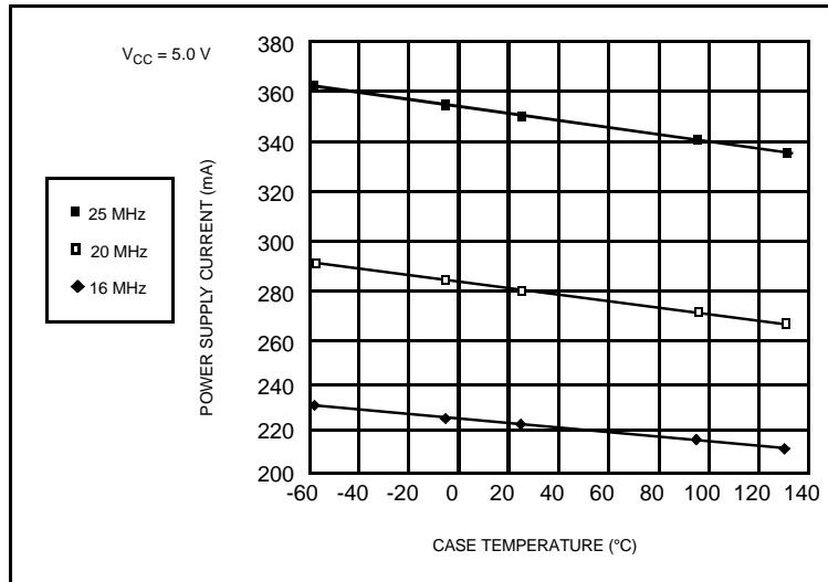
Figure 7. Typical Supply Current vs. Case Temperature
