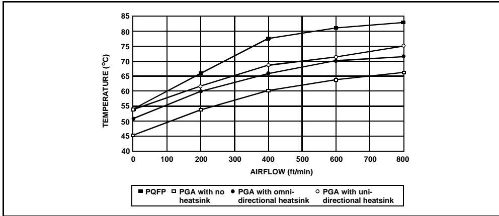
Figure 25. 25 MHz Maximum Allowable Ambient Temperature
