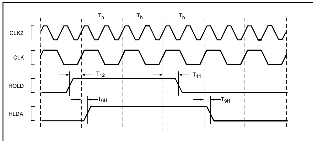
Figure 22. HOLD Timing
