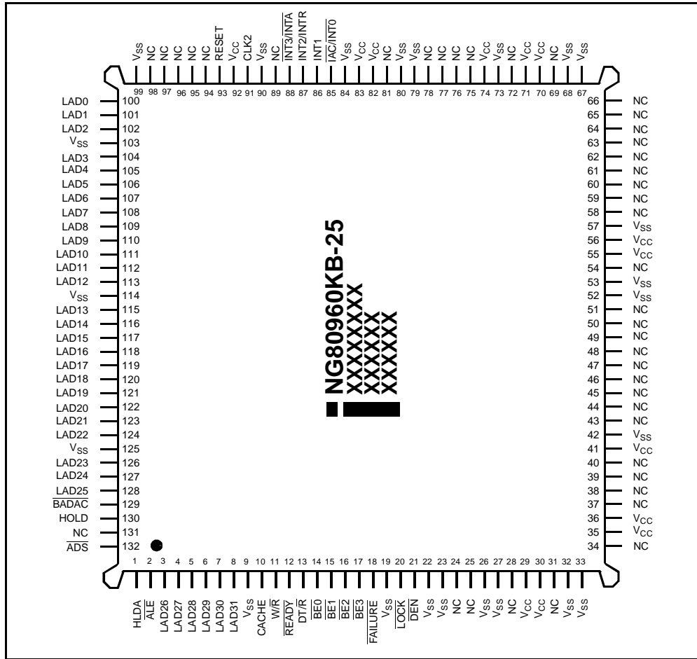
Figure 21. PQFP Pinout - View From Top
