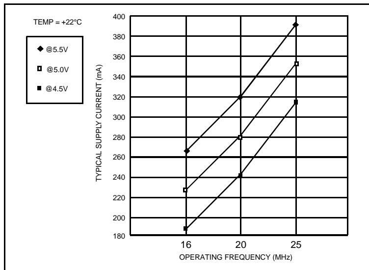
Figure 8. Typical Current vs. Frequency (Room Temp)
