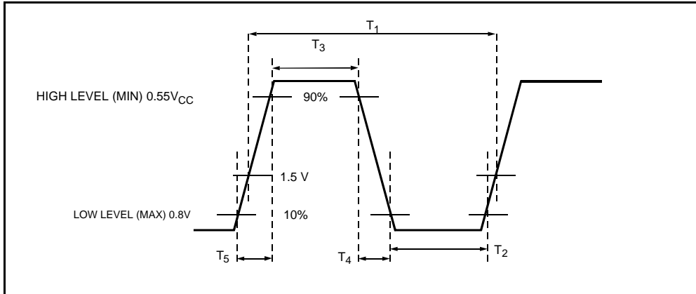
Figure 15. Processor Clock Pulse (CLK2)
