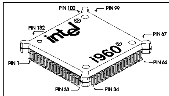
Figure 20. 80960KB 132-Lead Plastic Quad Flat-Pack (PQFP) Package
