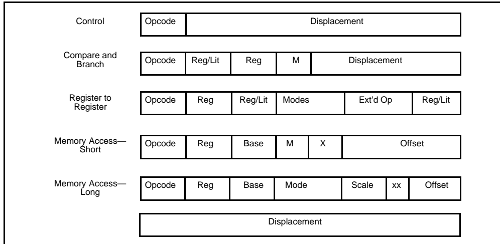
Figure 3. Instruction Formats
