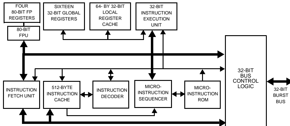
Figure 1. The 80960KB Processor's Highly Parallel Architecture
