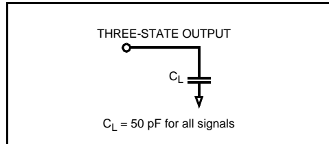
Figure 12. Test Load Circuit for Three-State Output Pins
