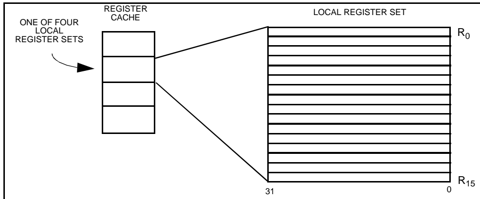
Figure 4. Multiple Register Sets Are Stored On-Chip
