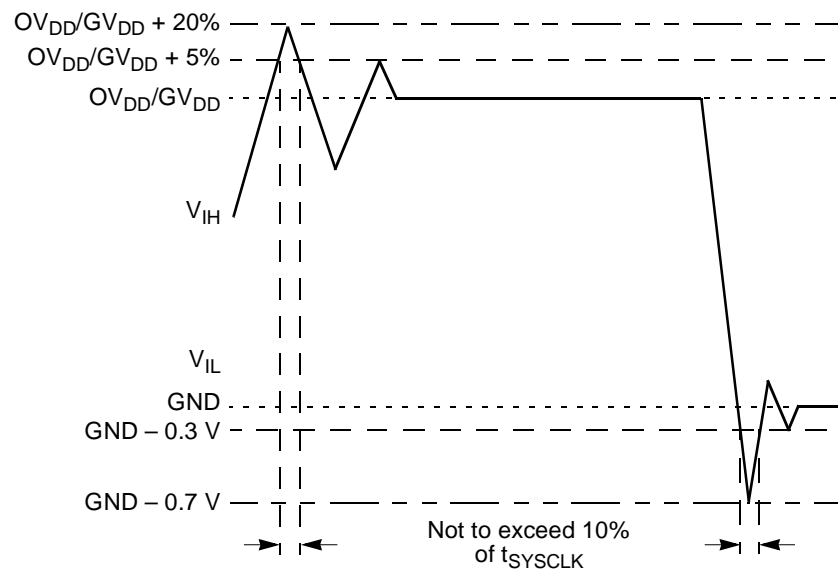
Figure 2. Overshoot/Undershoot Voltage
