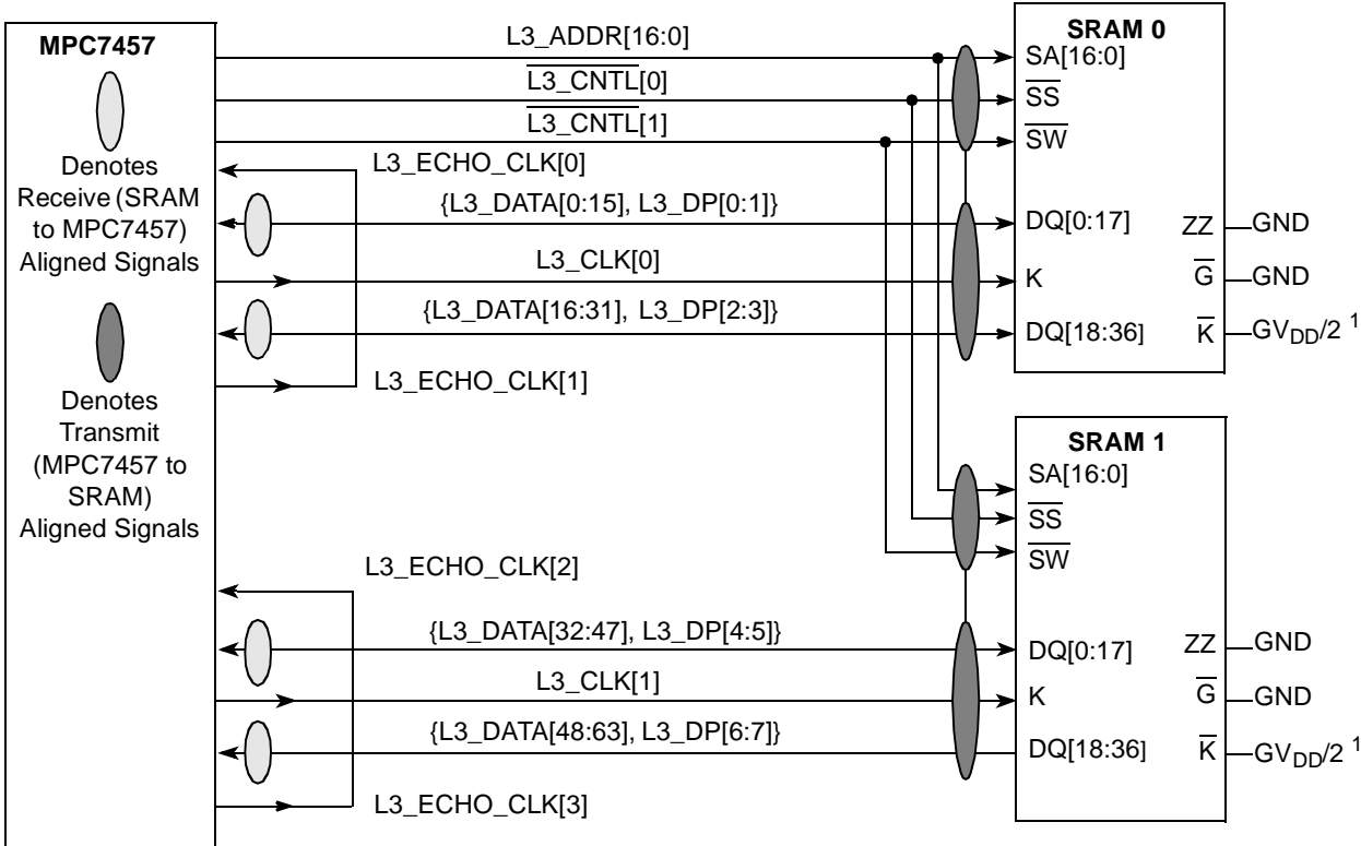
Figure 11 shows the typical connection diagram for the MPC7457 interfaced to PB2 SRAMs or Late Write SRAMs.
