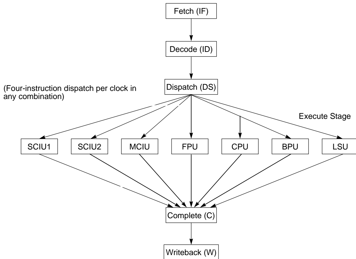
Figure 7. Pipeline Diagram
