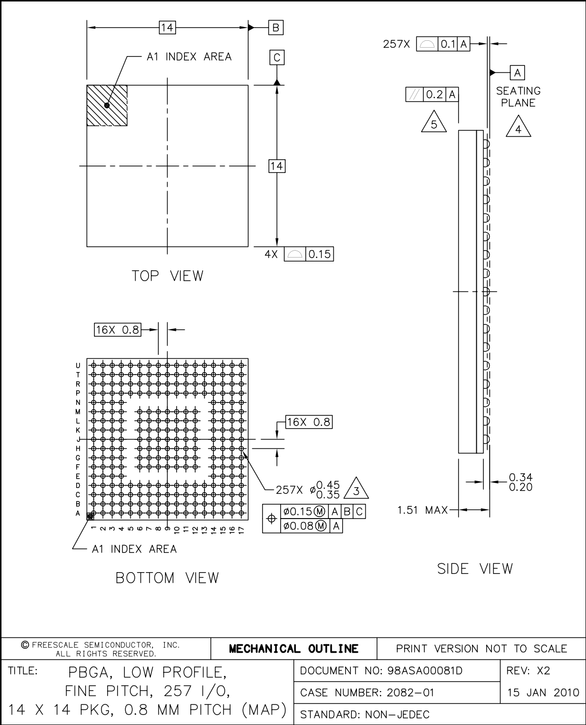
Figure 60. 257 MAPBGA mechanical data (1 of 2)
