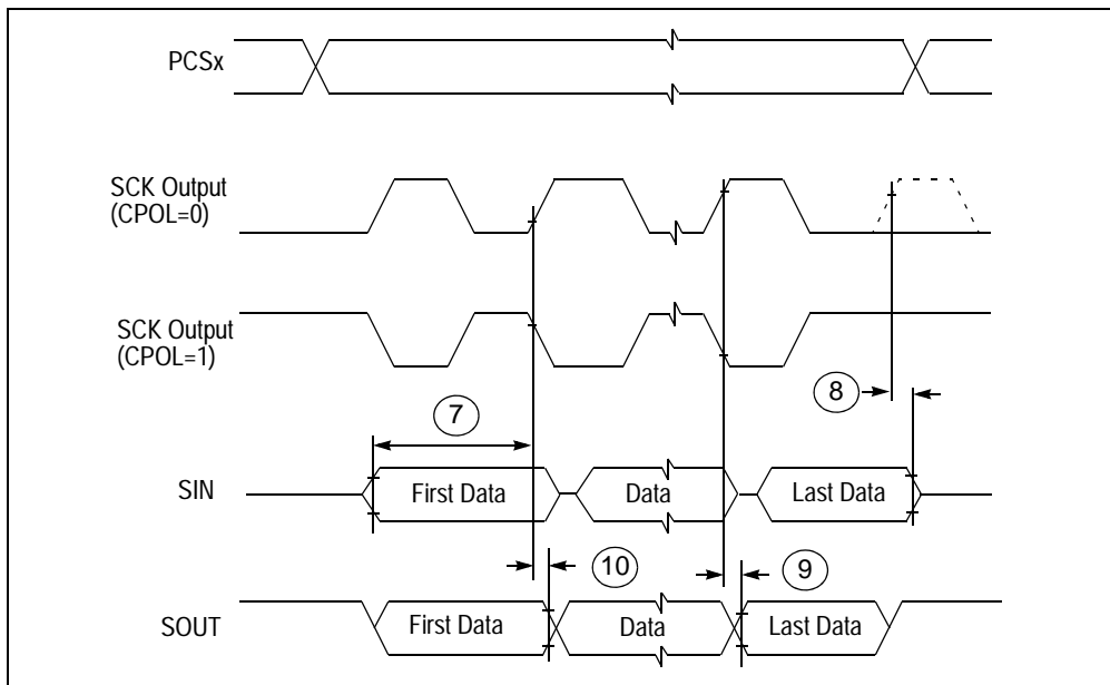
Figure 37. DSPI modified transfer format timing—master, CPHA = 1
