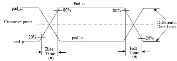
Figure 44. Rise/fall transition, part 1
