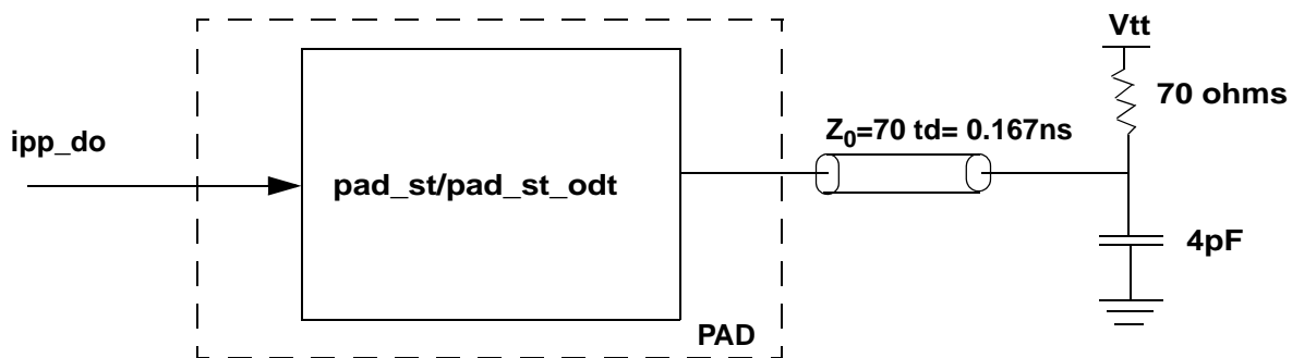
Figure 28. SSTL_2 Class II Test Load
