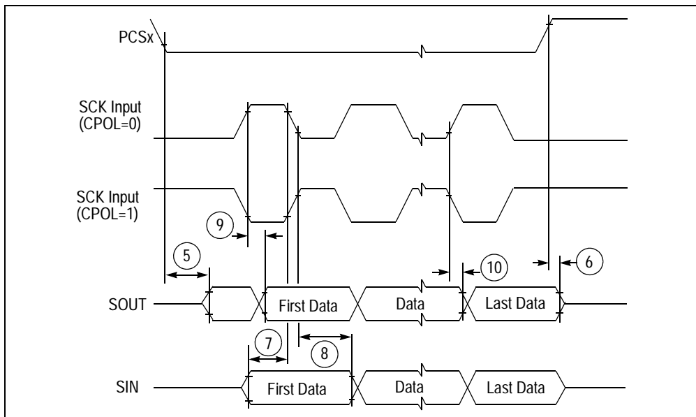
Figure 35. DSPI classic SPI timing—slave, CPHA = 1
