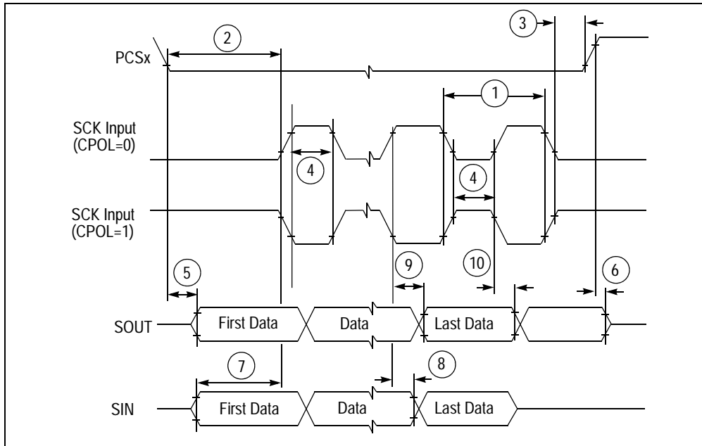
Figure 38. DSPI modified transfer format timing—slave, CPHA = 0
