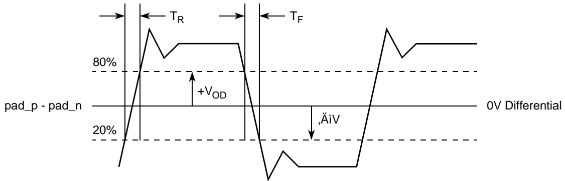
Figure 46. Illustration of t_r , t_f , and V_{OD}
