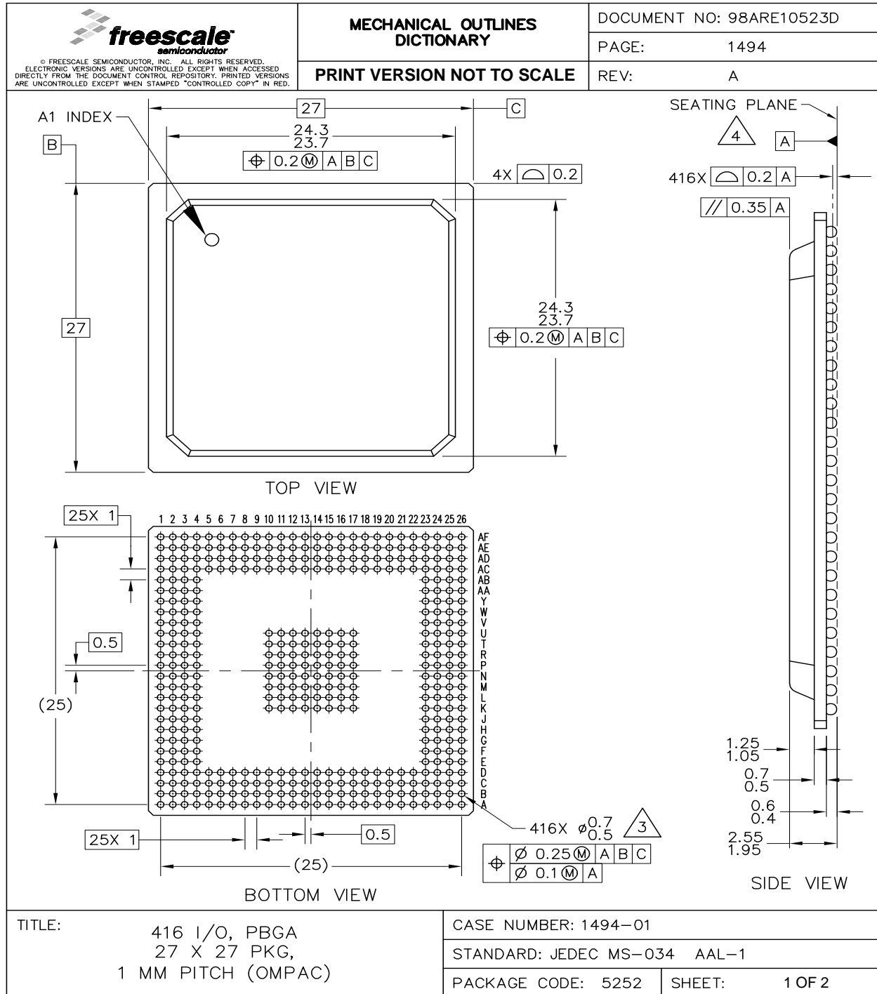
Figure 53. 416 TEPBGA mechanical drawing (part 1 of 2)
