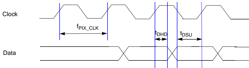
Figure 30. VIU2 timing diagram
