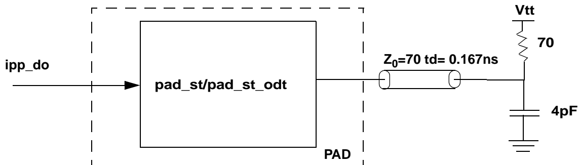
Figure 29. SSTL_18 CLass II Test Load
