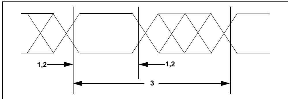
Figure 31. IRQ and NMI Timing
