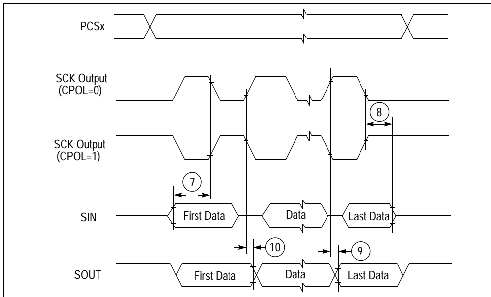
Figure 33. DSPI classic SPI timing—master, CPHA = 1
