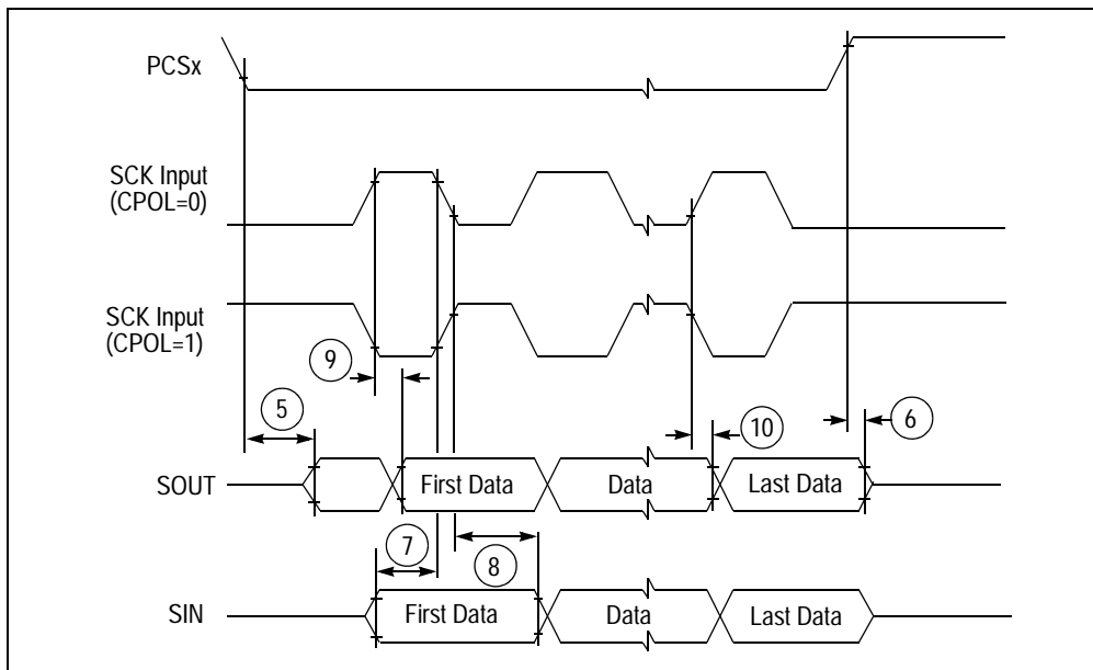
Figure 39. DSPI modified transfer format timing—slave, CPHA = 1
