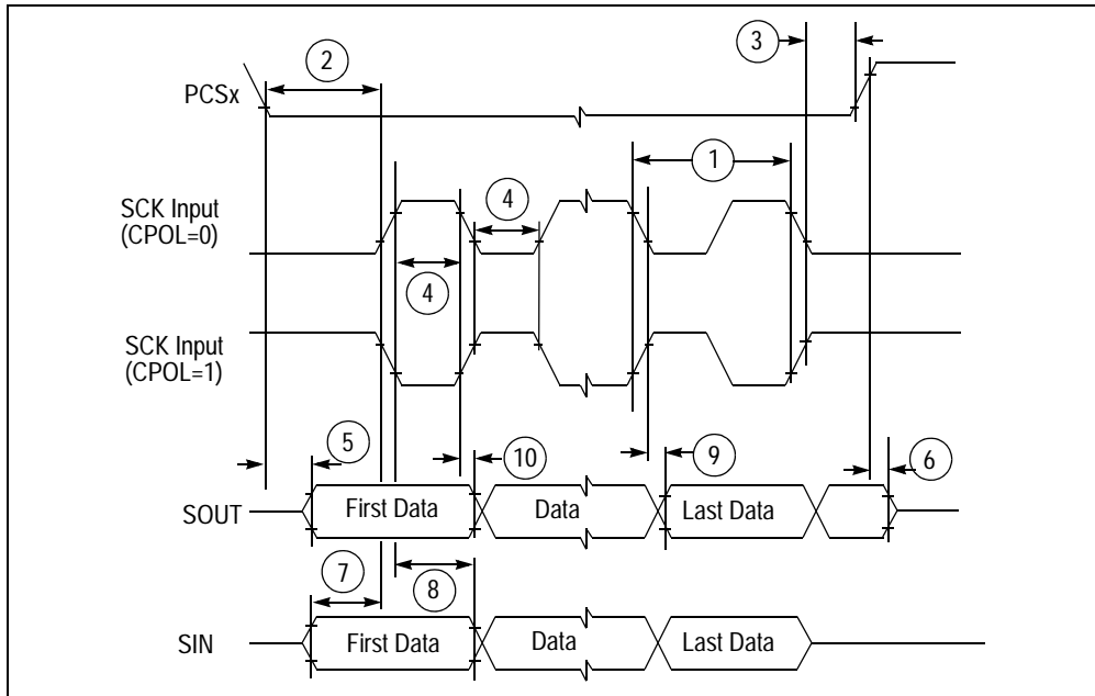
Figure 34. DSPI classic SPI timing—slave, CPHA = 0
