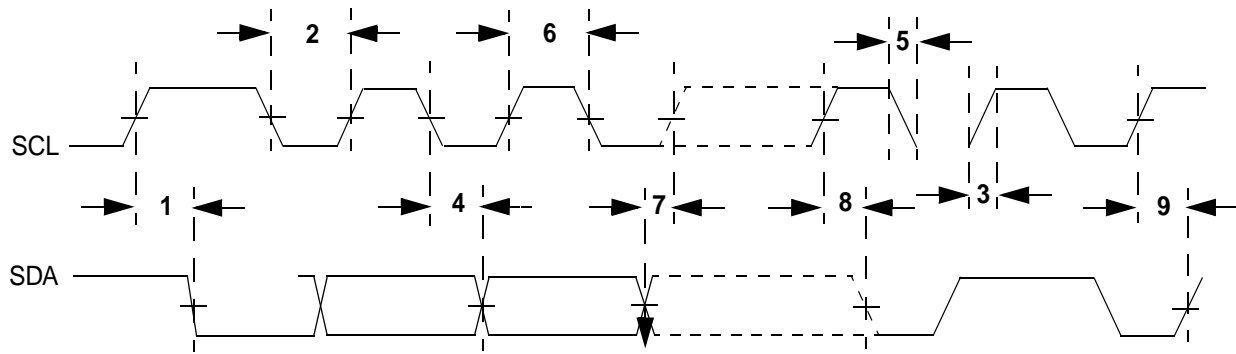
Figure 40. I 2 C input/output timing
