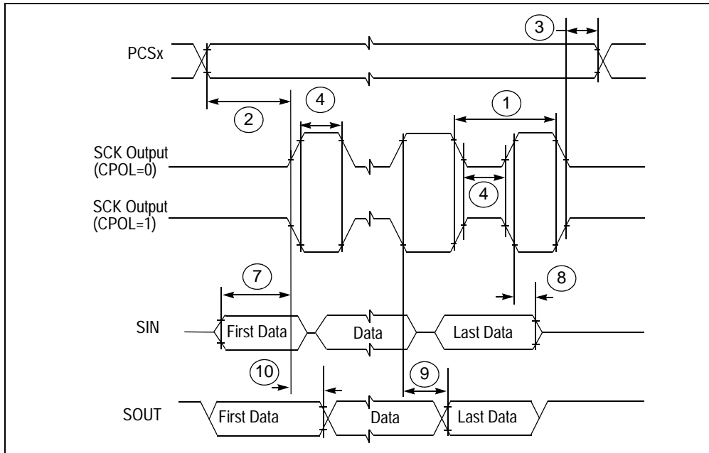
Figure 36. DSPI modified transfer format timing—master, CPHA = 0
