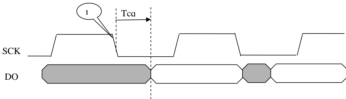
Figure 41. QuadSPI output timing
