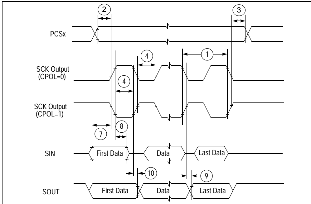
Figure 32. DSPI classic SPI timing—master, CPHA = 0
