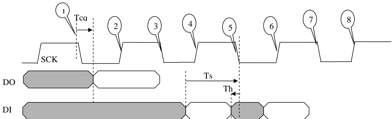
Figure 41. QuadSPI output timing
