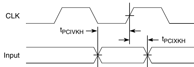
Figure 31. PCI Input AC Timing Measurement Conditions
