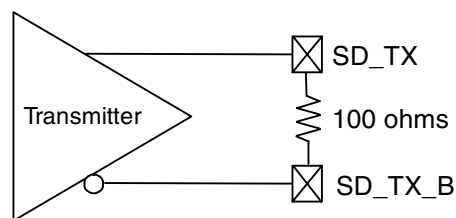
Figure 15. Transmitter Reference Circuit
