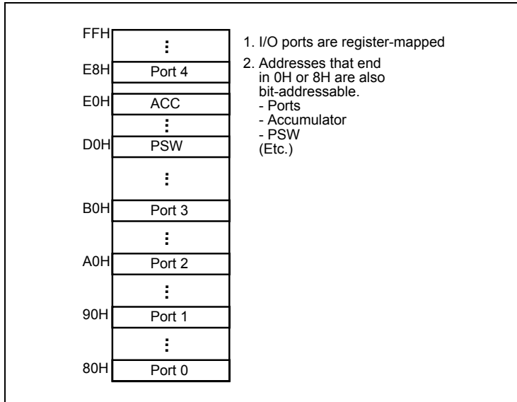
Figure 5-4. SFR Space
