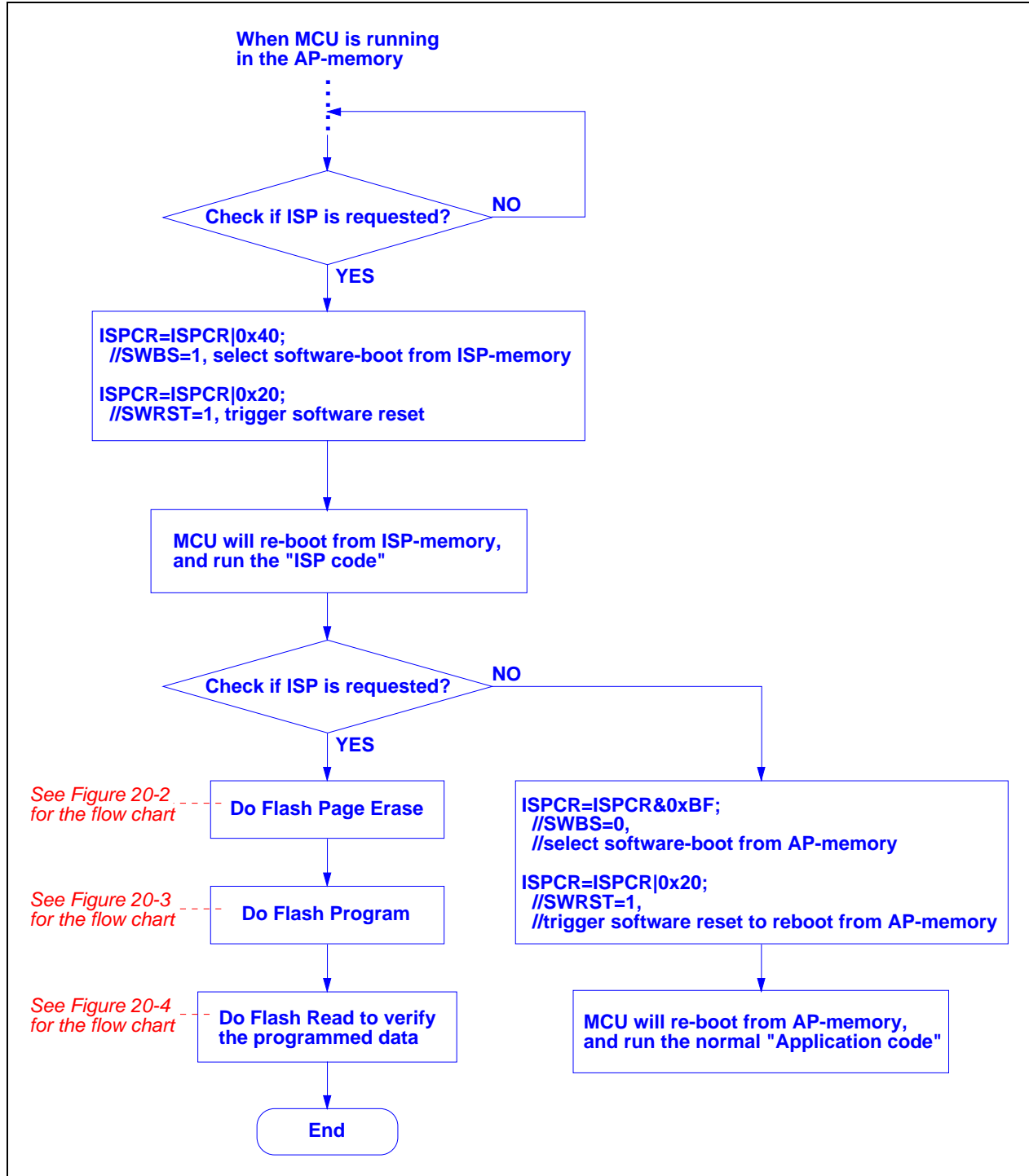
Figure 20-6. Re-boot from ISP-memory through AP-memory
