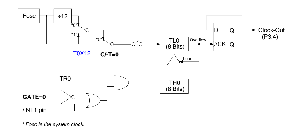
Figure 11-5. Programmable Clock-Out from Timer 0
