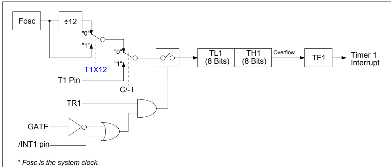
Figure 11-2. Timer 1 in Mode 1: 16-Bit Timer/Counter
