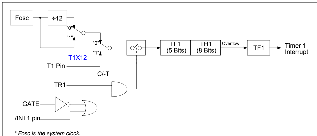
Figure 11-1. Timer 1 in Mode 0: 13-Bit Timer/Counter
