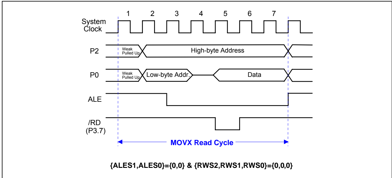
Figure 8-3. "MOVX A,@DPTR" without Stretch
