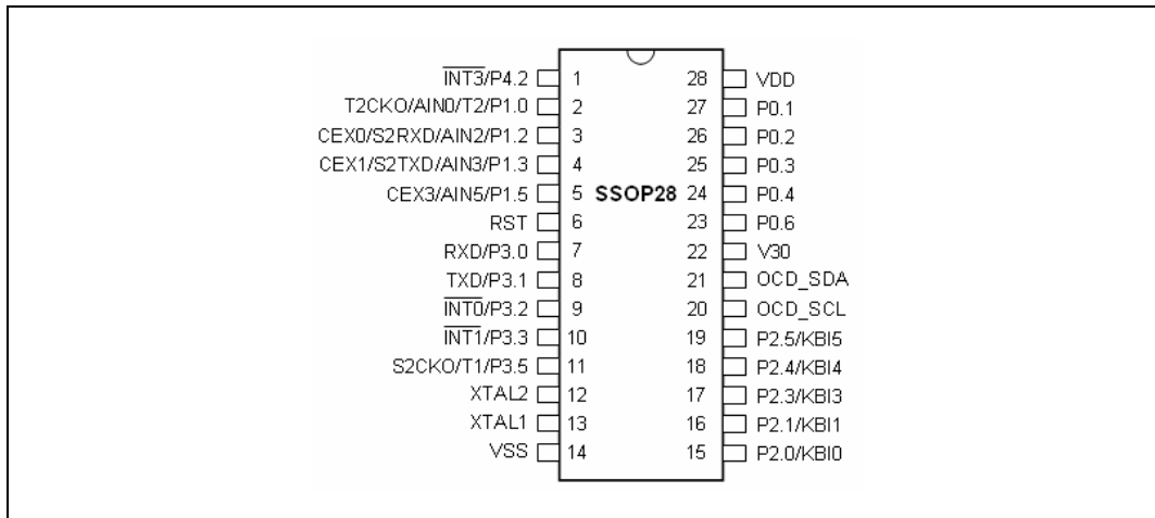
Figure 4-2. Pin Assignment: 28-Pin SSOP
