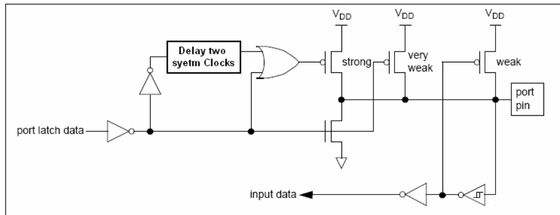
Figure 10-1. Quasi-Bidirectional I/O
