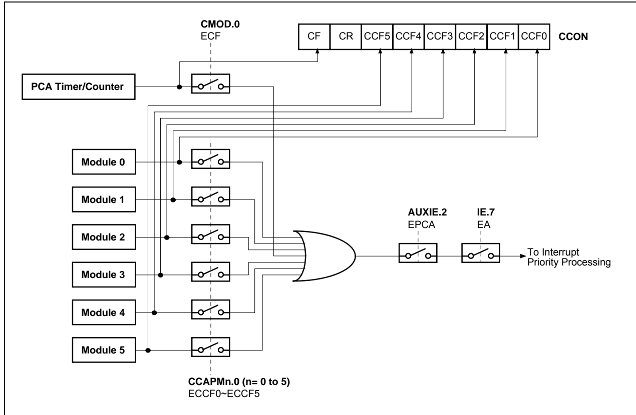
Figure 14-3. PCA Interrupt System
