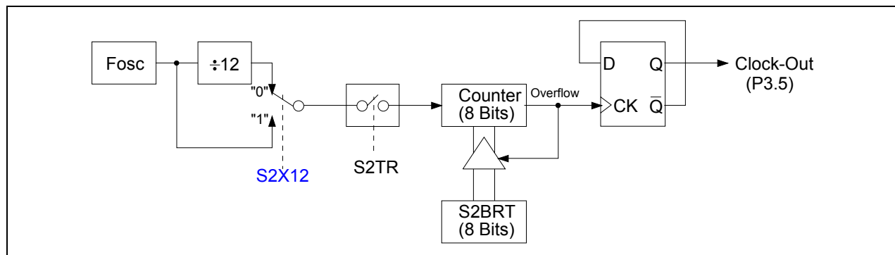
Figure 13-2. Programmable Clock-Out from UART2 Baud Rate Timer
