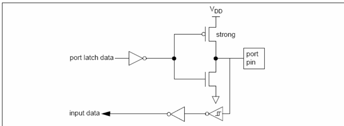
Figure 10-4. Push-Pull Output
