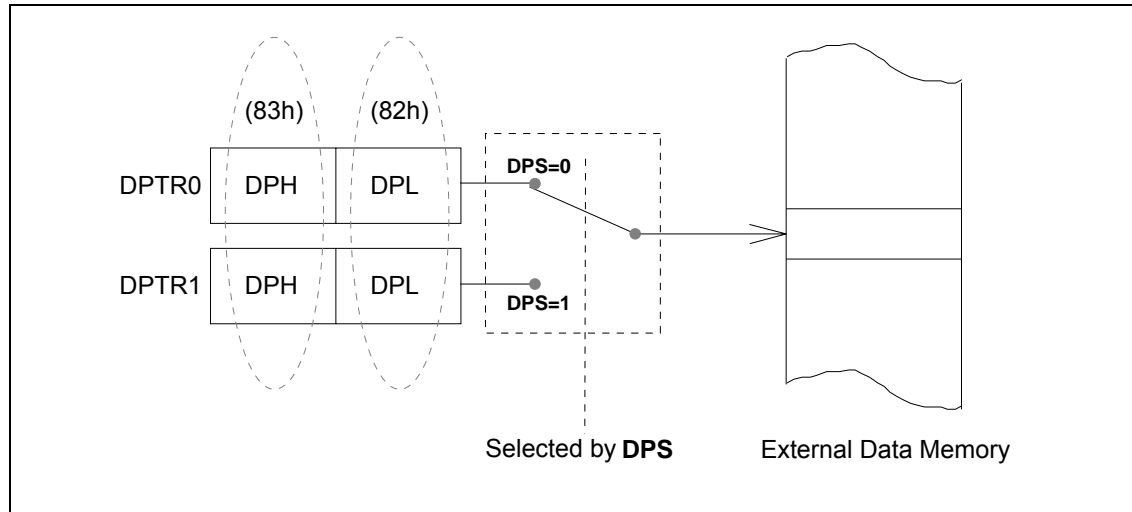
Figure 9-1. Use of Dual DPTR
