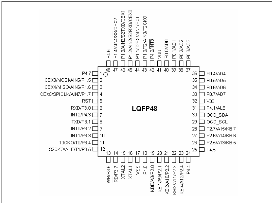
Figure 4-5. Pin Assignment: 48-Pin LQFP
