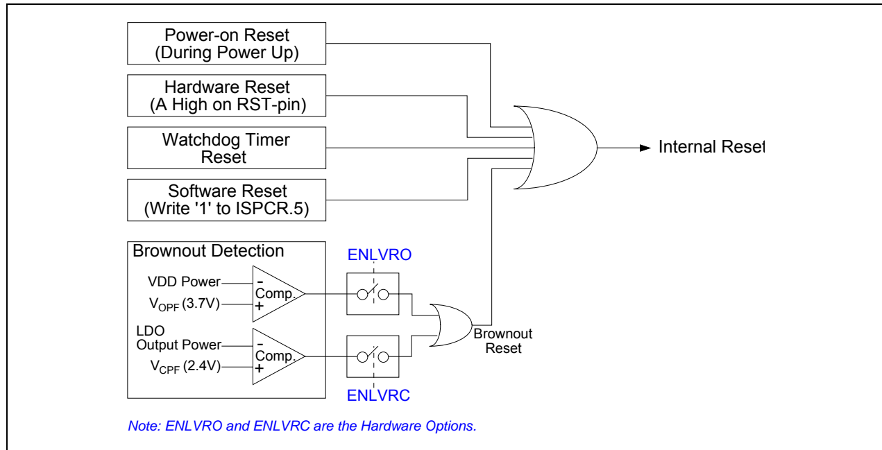
Figure 24-1. Block Diagram of Reset
