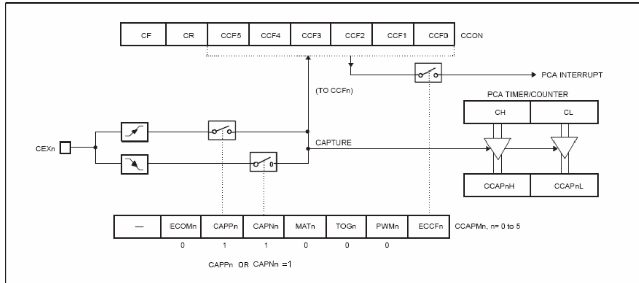
Figure 14-4. PCA Capture Mode
