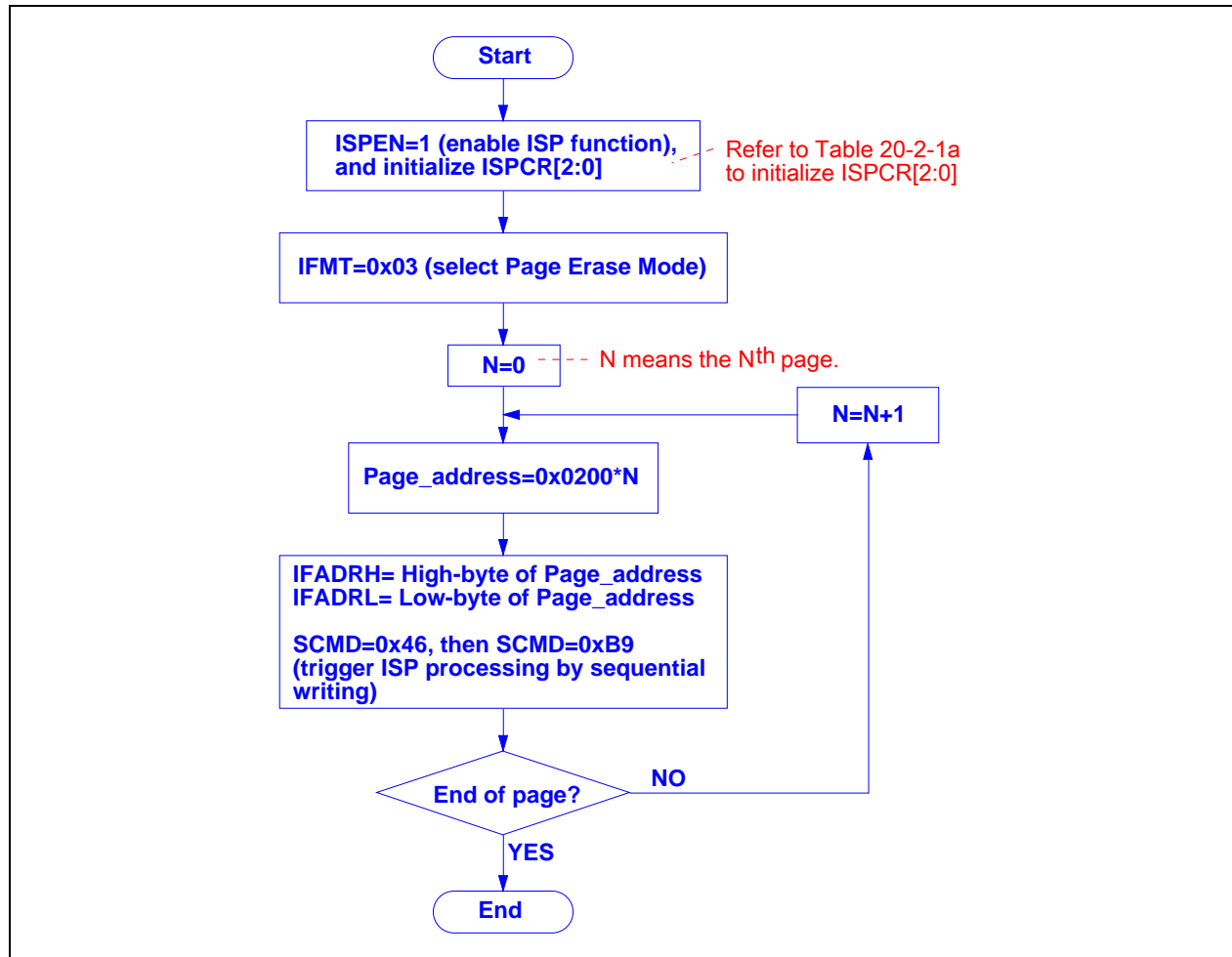
Figure 20-2. Flow Chart for “Flash Page Erase”
