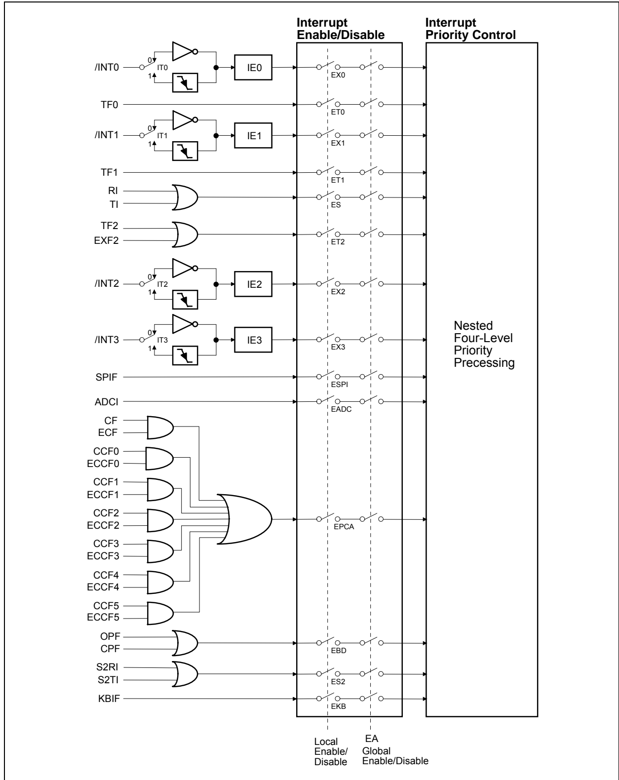
Figure 19-1. Interrupt System
