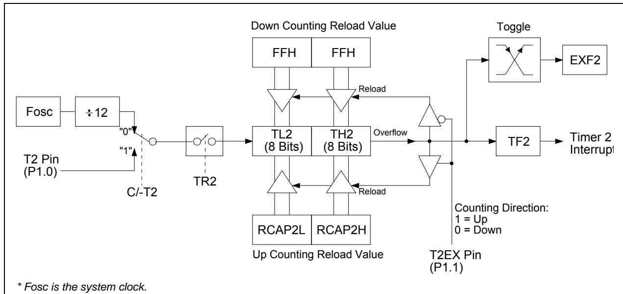
Figure 11-8. Timer 2 in Auto-Reload Mode (DCEN=1)
