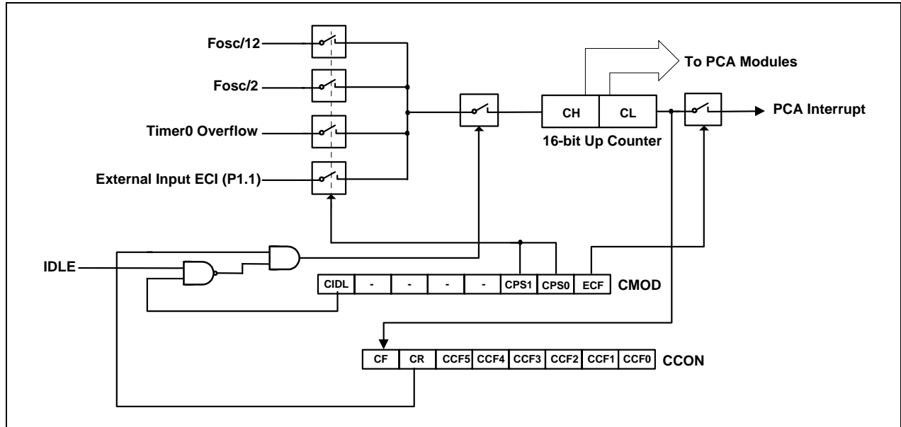
Figure 14-2. PCA Timer/Counter
