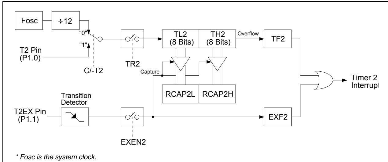
Figure 11-6. Timer 2 in Capture Mode
