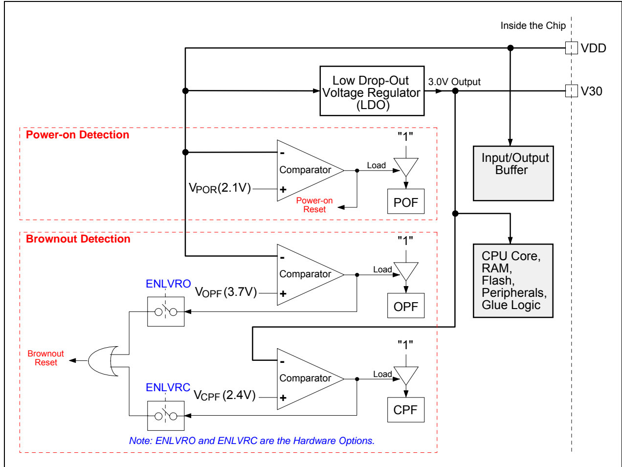
Figure 23-1. Power Monitor Block Diagram
