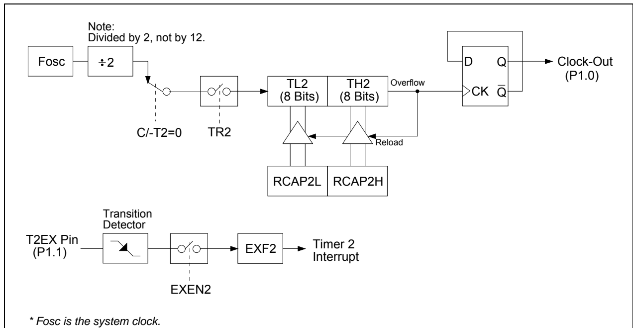
Figure 11-10. Programmable Clock-Out from Timer 2
