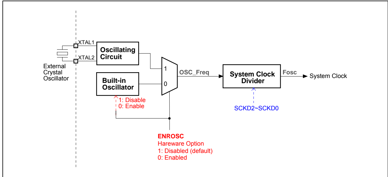
Figure 22-1. Block Diagram of System Clock
