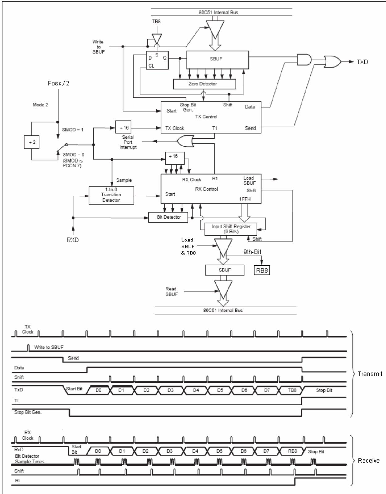
Figure 12-3. Serial Port Mode 2
