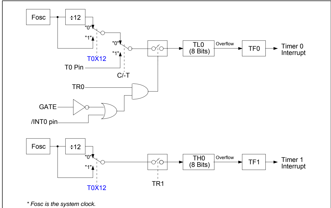
Figure 11-4. Timer 0 in Mode 3: Two 8-Bit Timer/Counters
