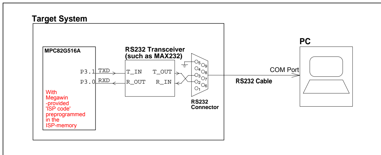
Figure 20-9. System Diagram for ISP via COM Port
