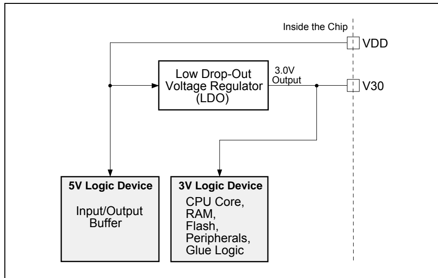
Figure 27-1. Power Scheme
