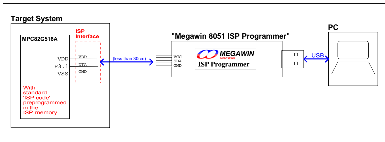
Figure 20-8. System Diagram for the ISP Function
