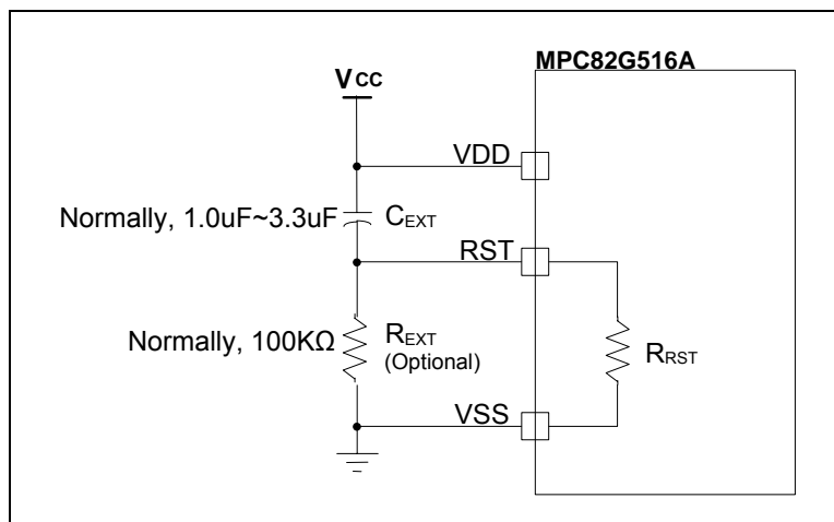
Figure 27-4. Reset Circuit
