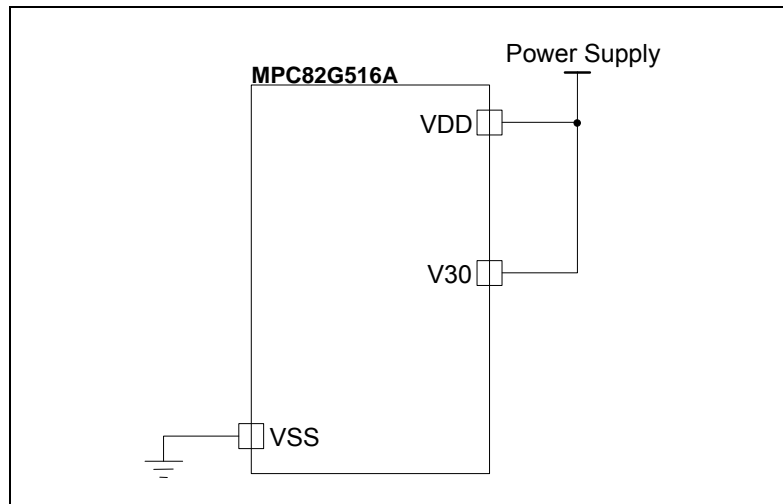
Figure 27-2. Power Supplied to a 3.3V System
