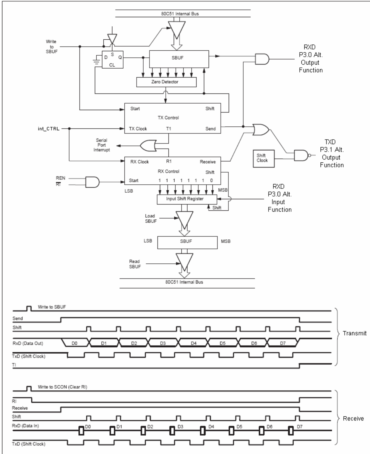
Figure 12-1. Serial Port Mode 0
