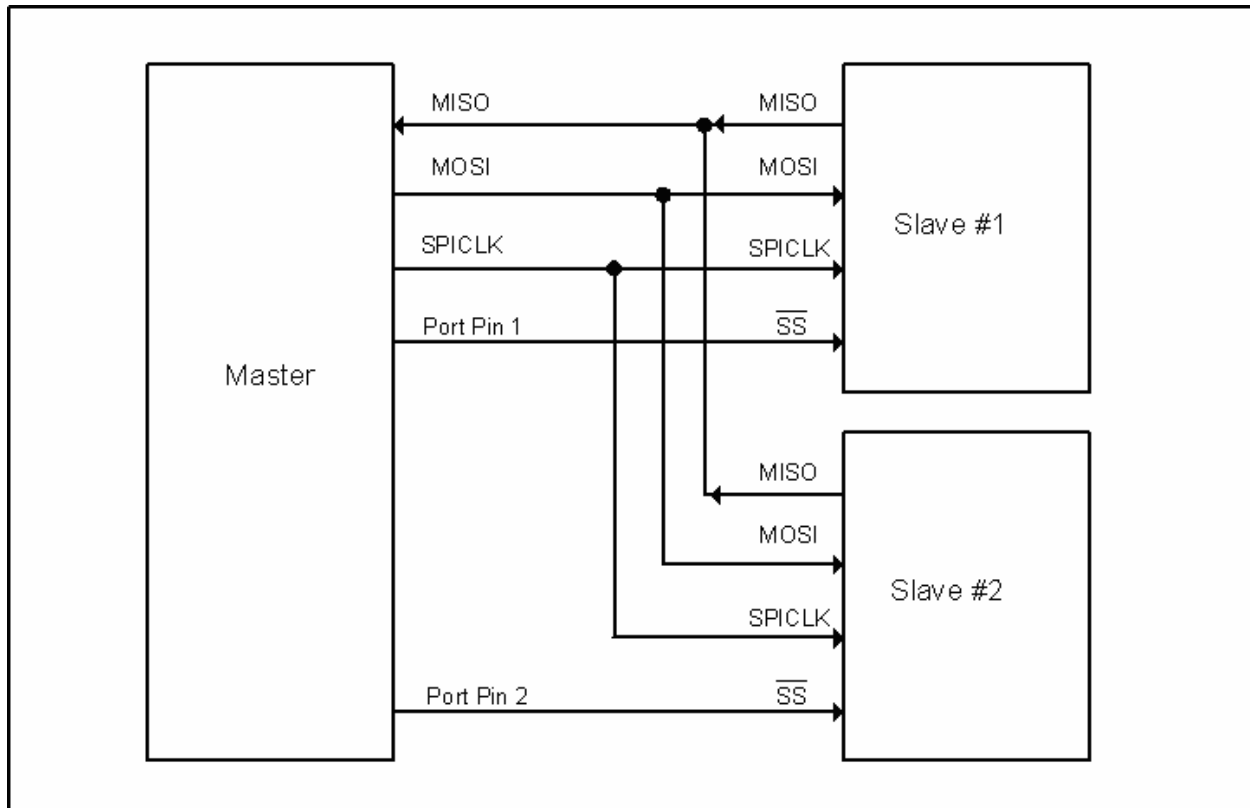
Figure 15-4. SPI single master multiple slaves configuration
