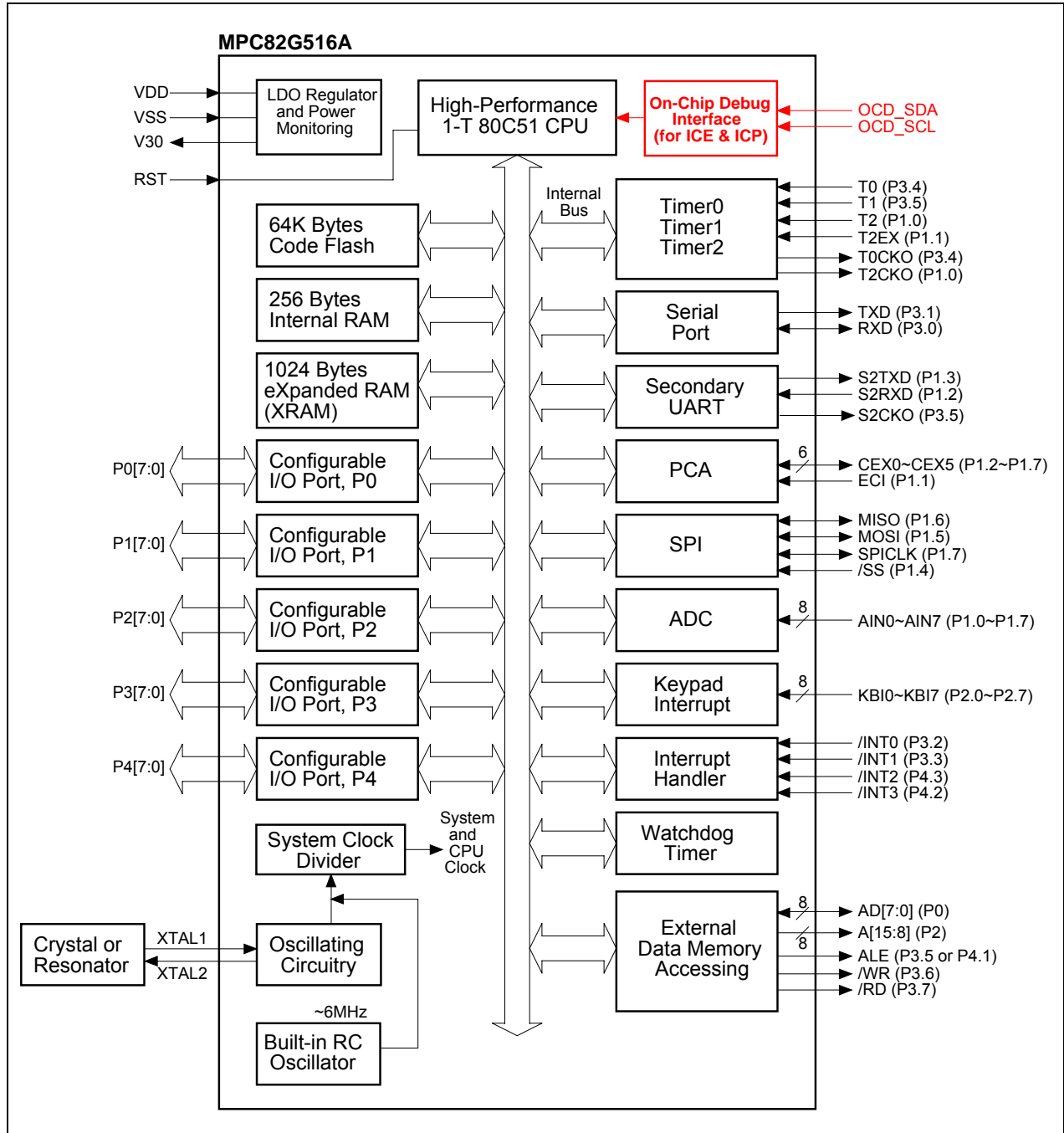
Figure 3-1. Block Diagram
