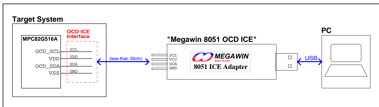
Figure 28-2. System Diagram for the ICE Function
