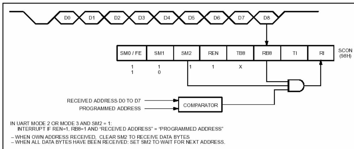
Figure 12-6. UART Multiprocessor Communication, Auto Address Recognition
