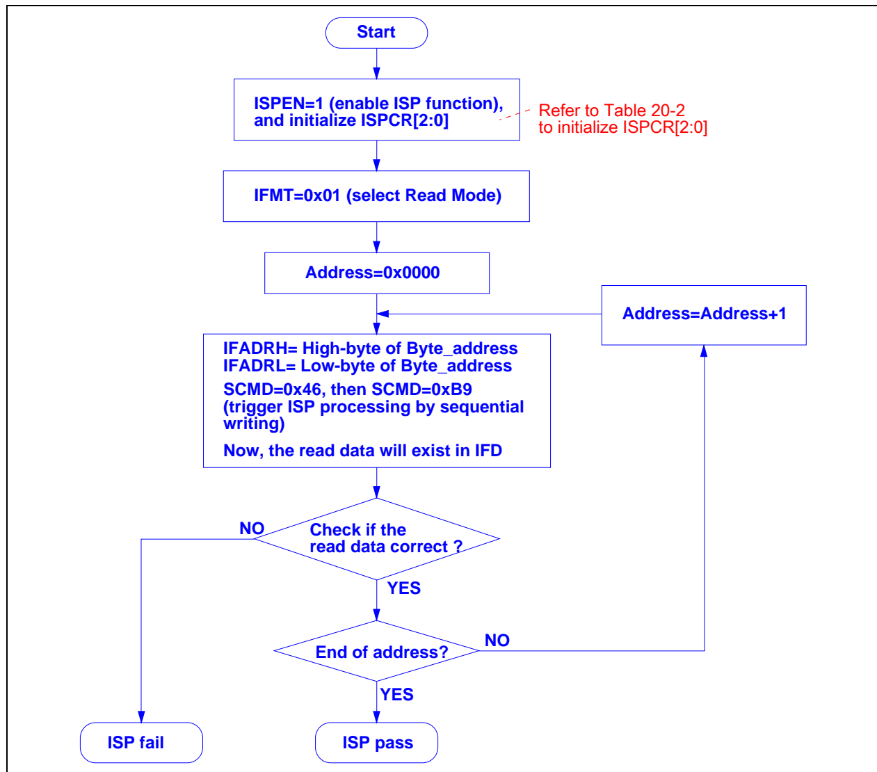
Figure 20-4. Flow Chart for “Flash Read”
