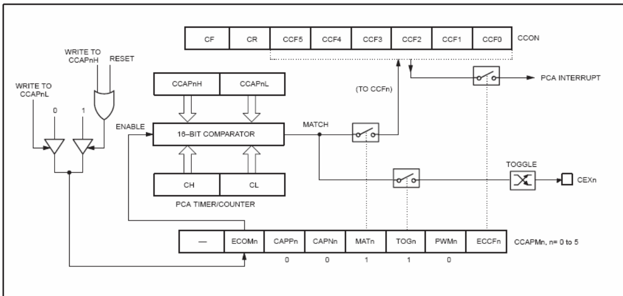
Figure 14-6. PCA High Speed Output Mode
