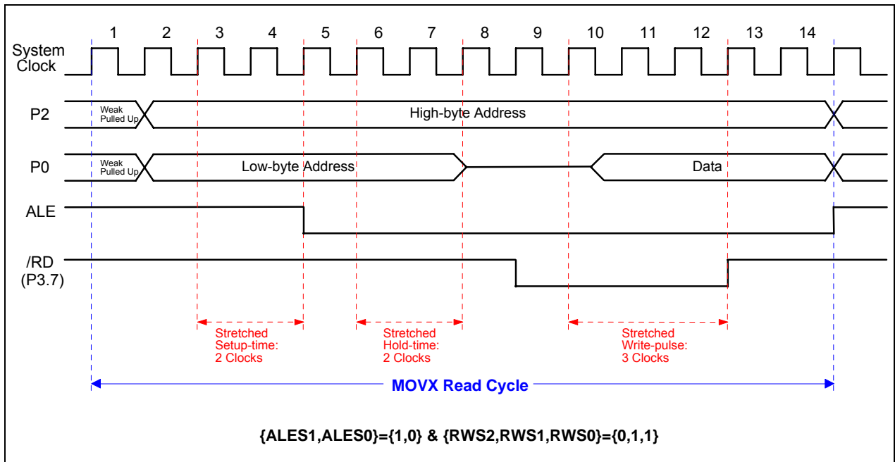
Figure 8-4. "MOVX A,@DPTR" with Stretch
