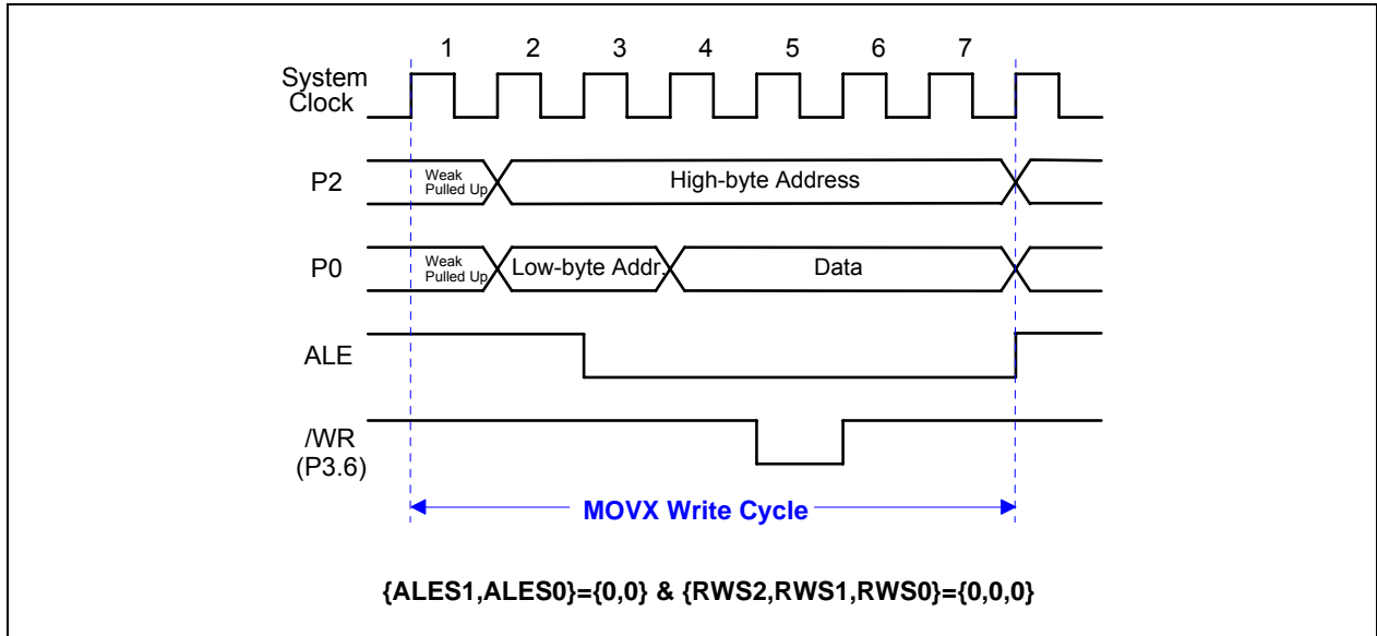
Figure 8-1. "MOVX @DPTR,A" without Stretch
