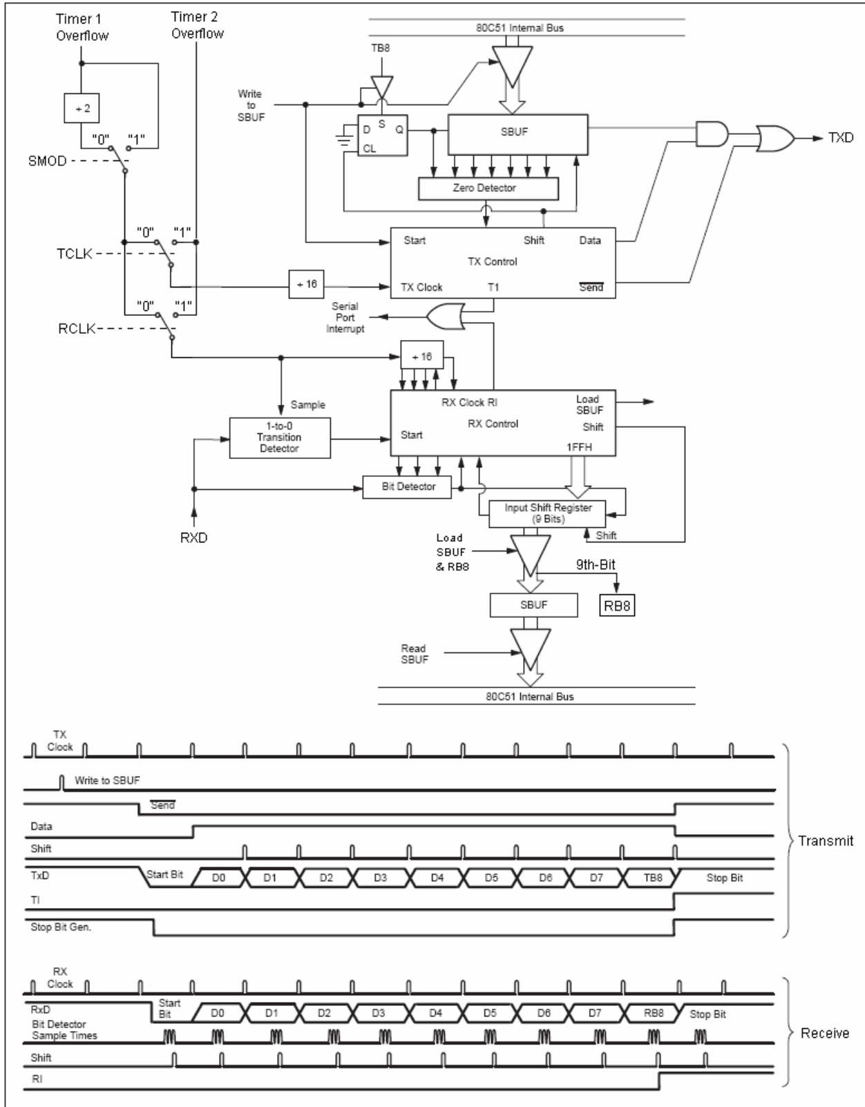
Figure 12-4. Serial Port Mode 3
