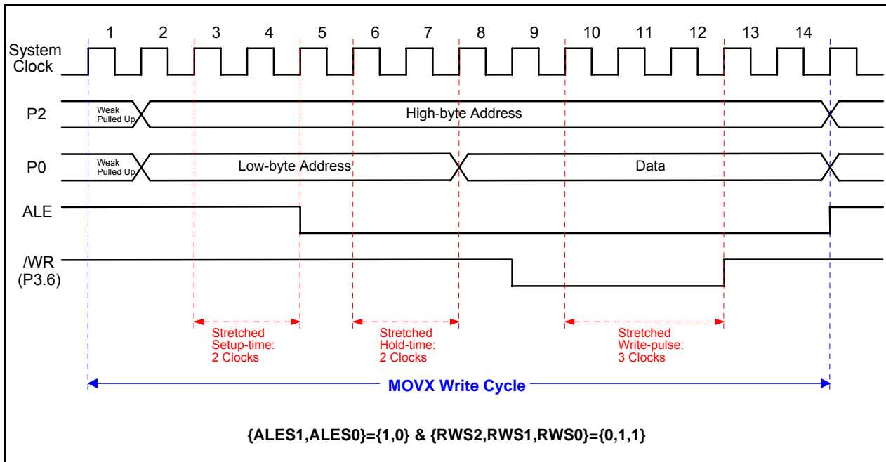
Figure 8-2. "MOVX @DPTR,A" with Stretch
