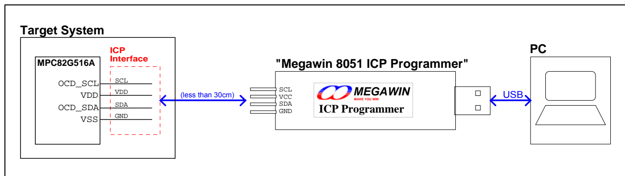
Figure 20-12. System Diagram for the ICP Function
