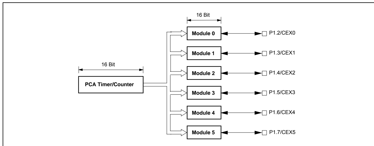
Figure 14-1. PCA Block Diagram
