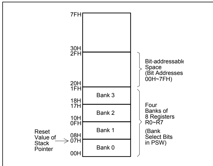
Figure 5-3. Lower 128 Bytes of Internal RAM
