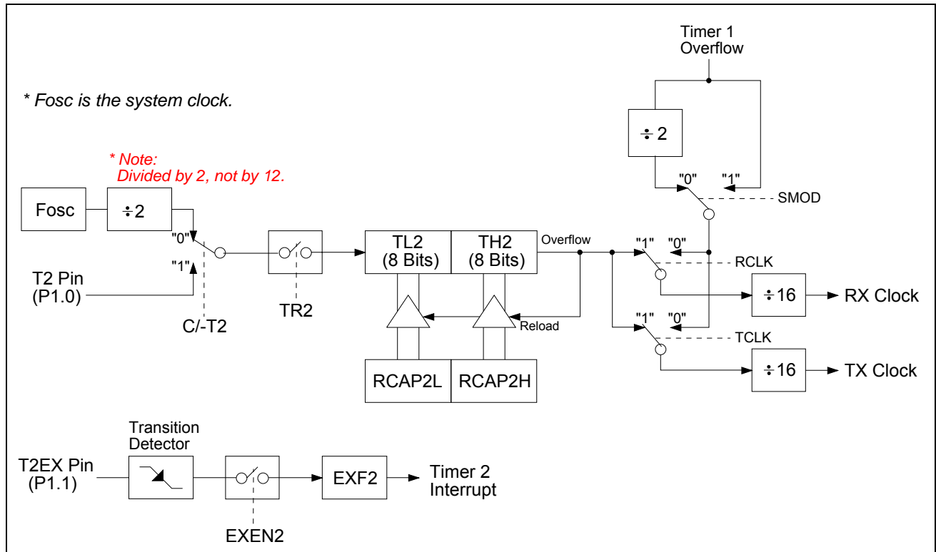
Figure 11-9. Timer 2 in Baud Rate Generator Mode
