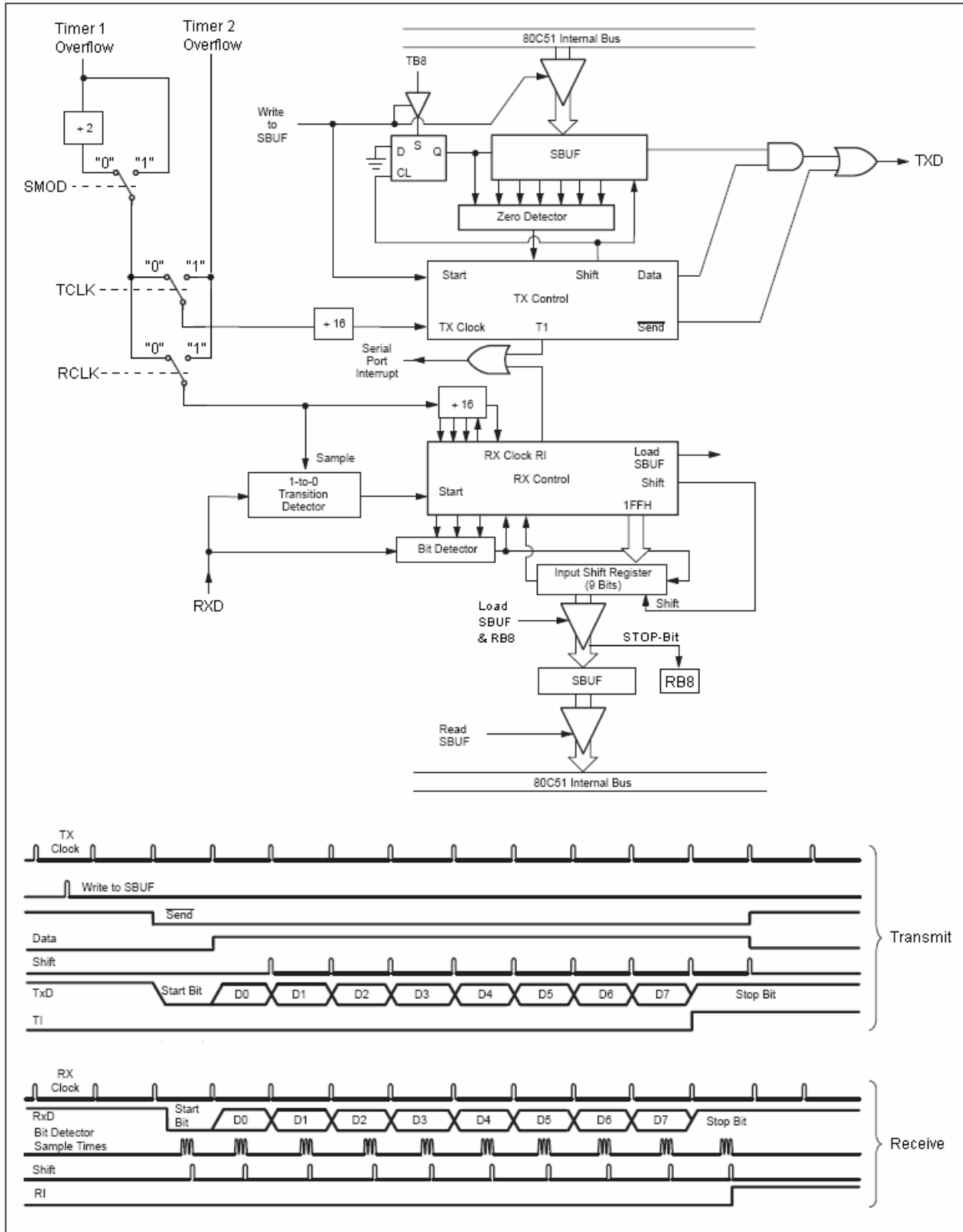
Figure 12-2. Serial Port Mode 1
