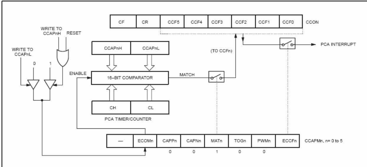
Figure 14-5. PCA Software Timer Mode
