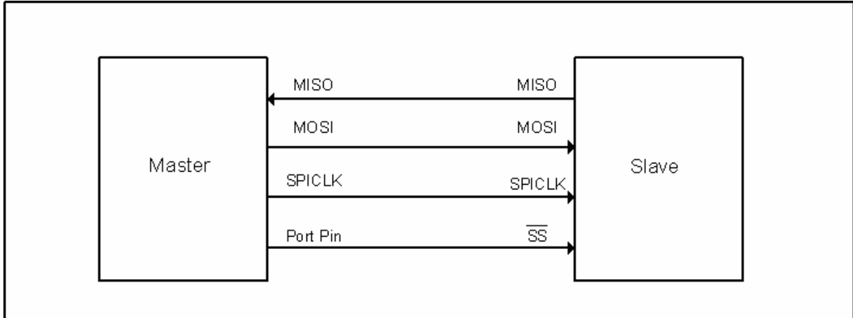
Figure 15-2. SPI single master single slave configuration
