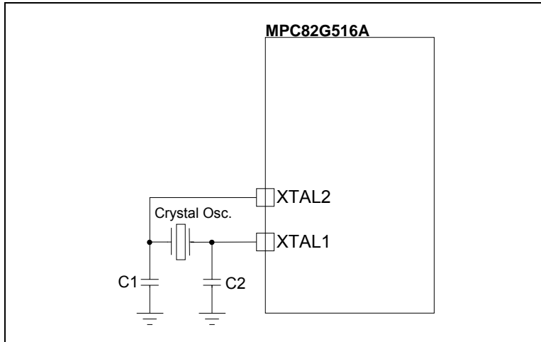
Figure 27-5. XTAL Oscillating Circuit
