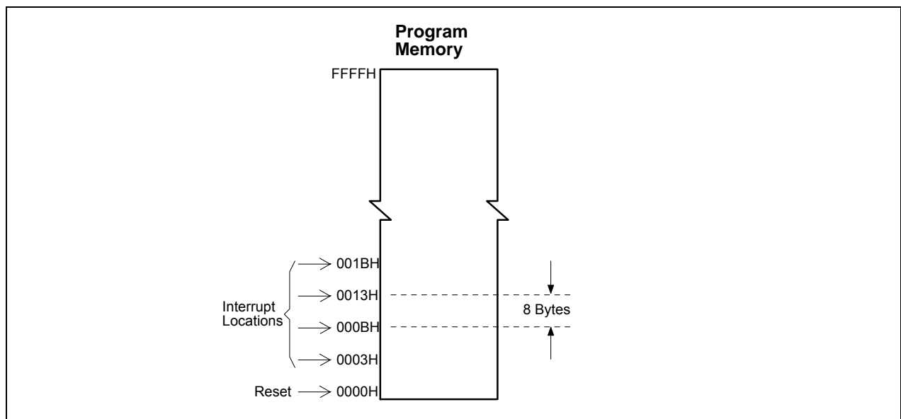
Figure 5-1. Program Memory
