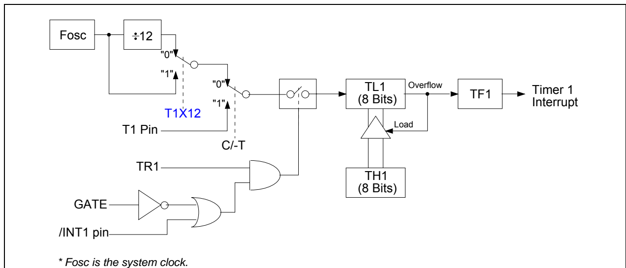
Figure 11-3. Timer 1 in Mode 2: 8-Bit Auto-Reload
