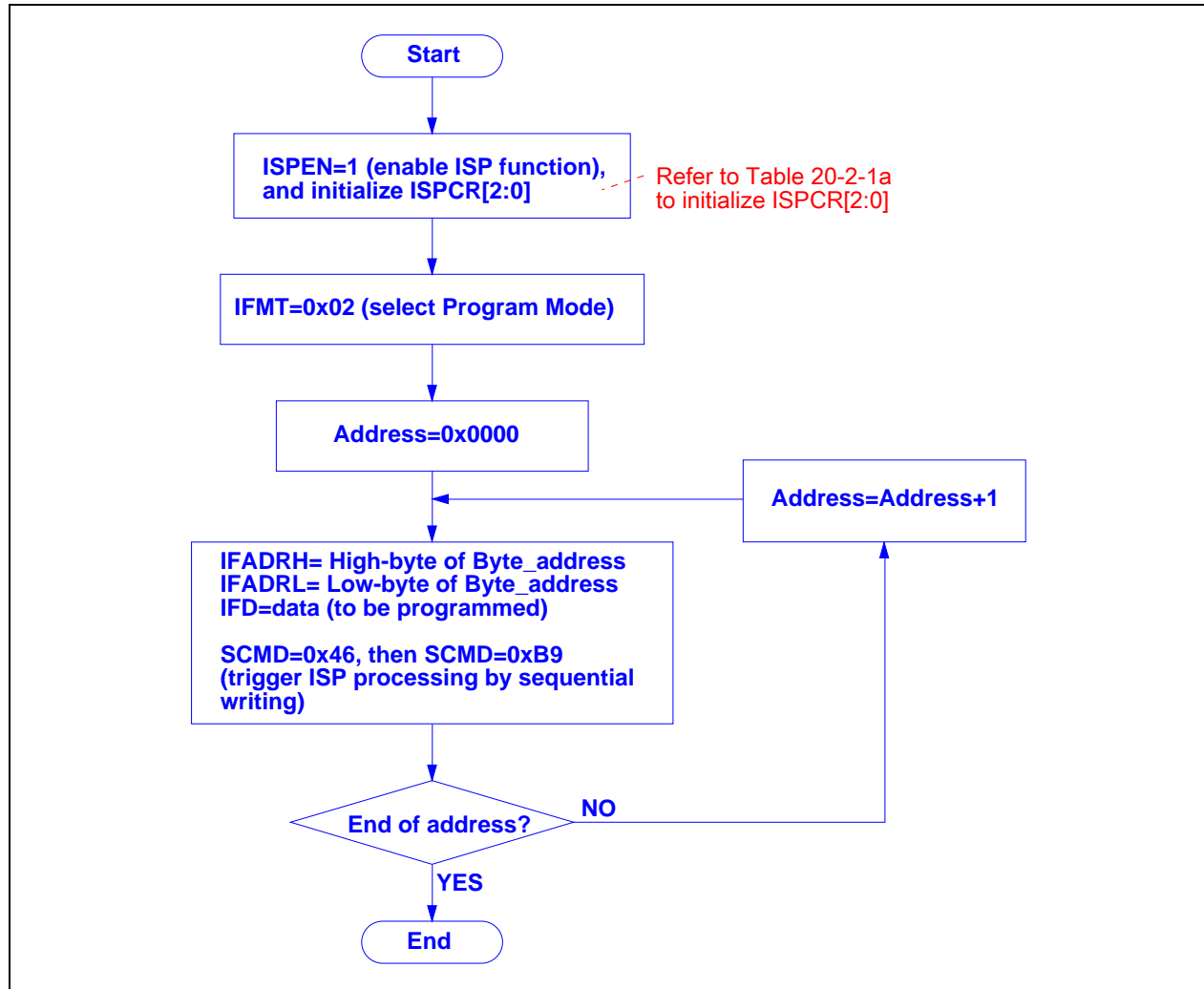
Figure 20-3. Flow Chart for “Flash Program”
