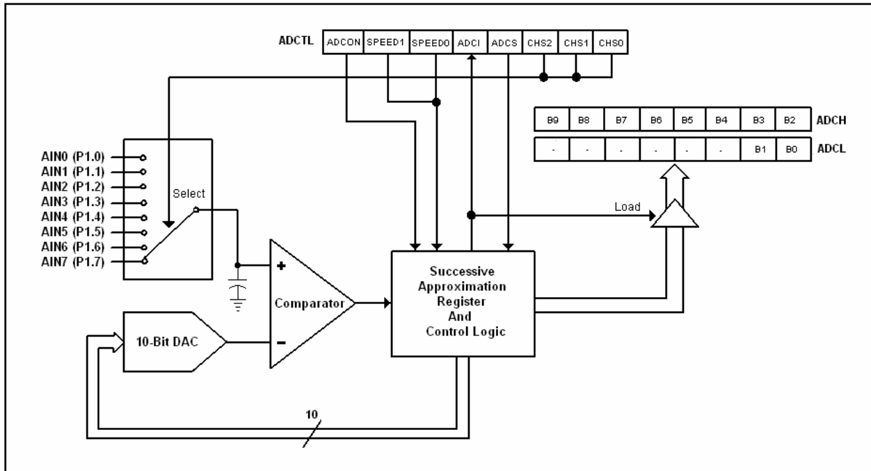
Figure 16-1. ADC Block Diagram
