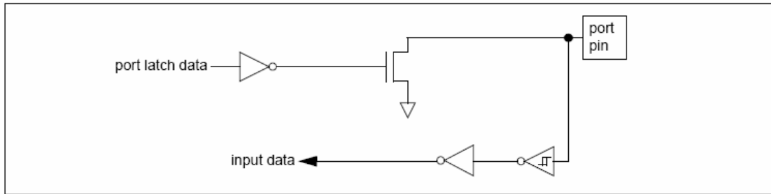
Figure 10-2. Open-Drain Output
