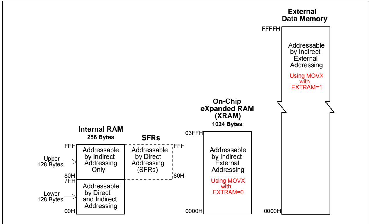
Figure 5-2. Data Memory
