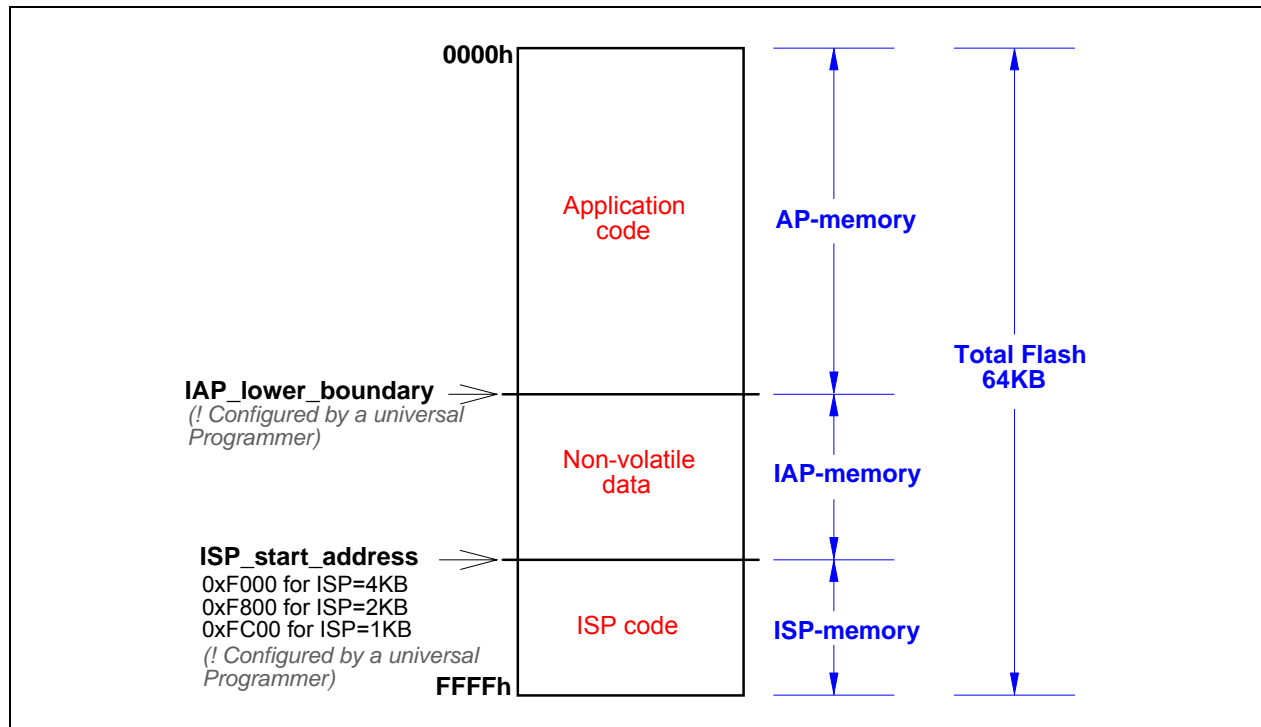
Figure 20-1. Flash Configuration
