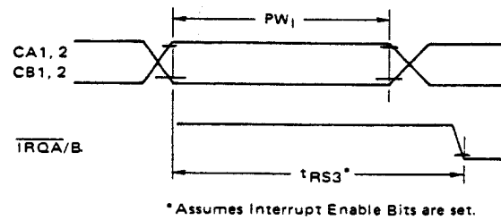
FIGURE 13 — INTERRUPT PULSE WIDTH AND \overline{\text{IRQ}} RESPONSE
