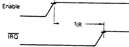
FIGURE 14 — \overline{\text{IRQ}} RELEASE TIME
