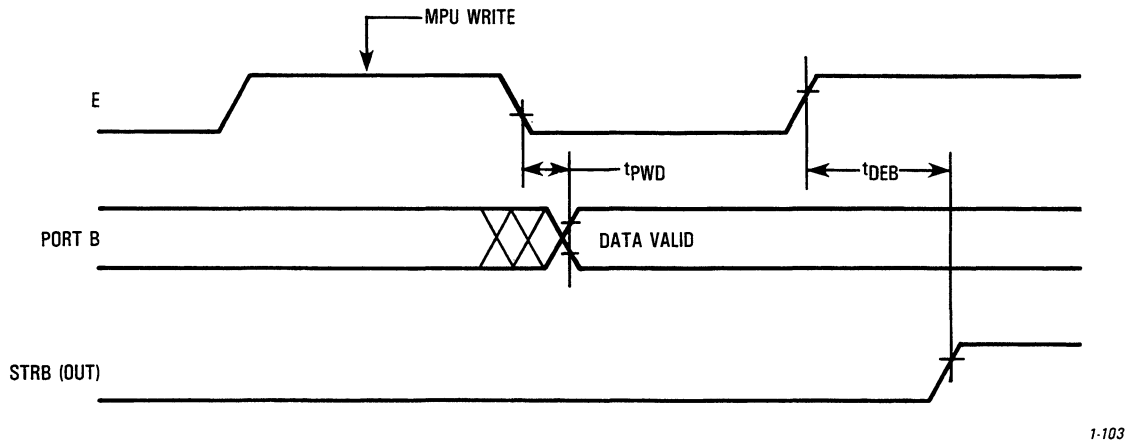
Figure 5. Simple Output Strobe Timing
