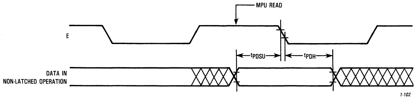
Figure 4. Port C Static Read Timing
