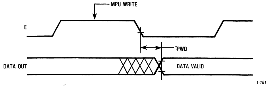
Figure 3. Port Write Timing
