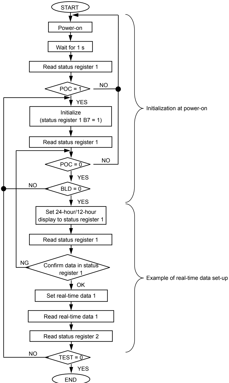
Figure 51 Example of Initialization Flowchart Seiko Instruments Inc.
