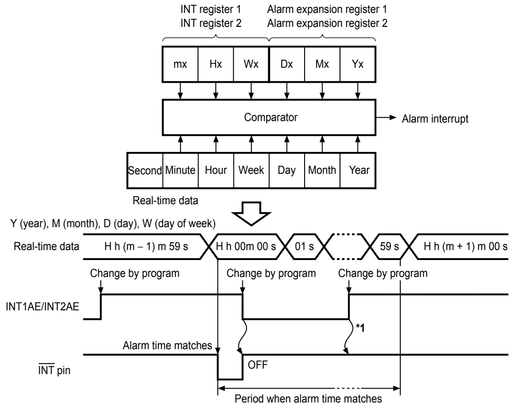
Figure 31 Alarm Interrupt Output Timing (1/2) Seiko Instruments Inc.
