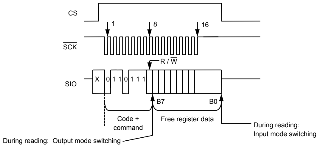
Figure 47 Free Register Access
