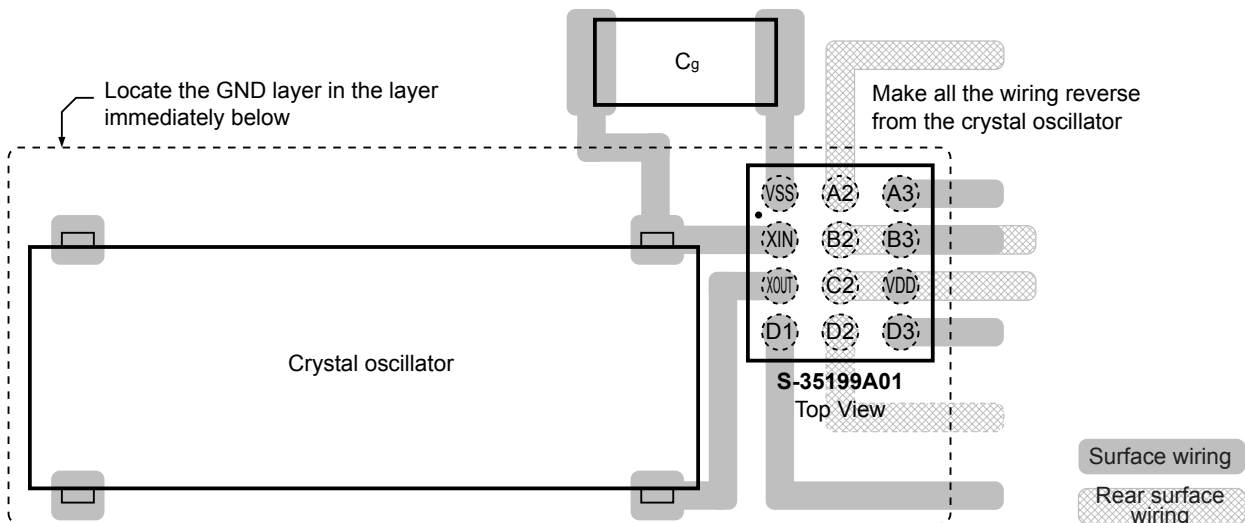
Figure 55 Connection Diagram 2
