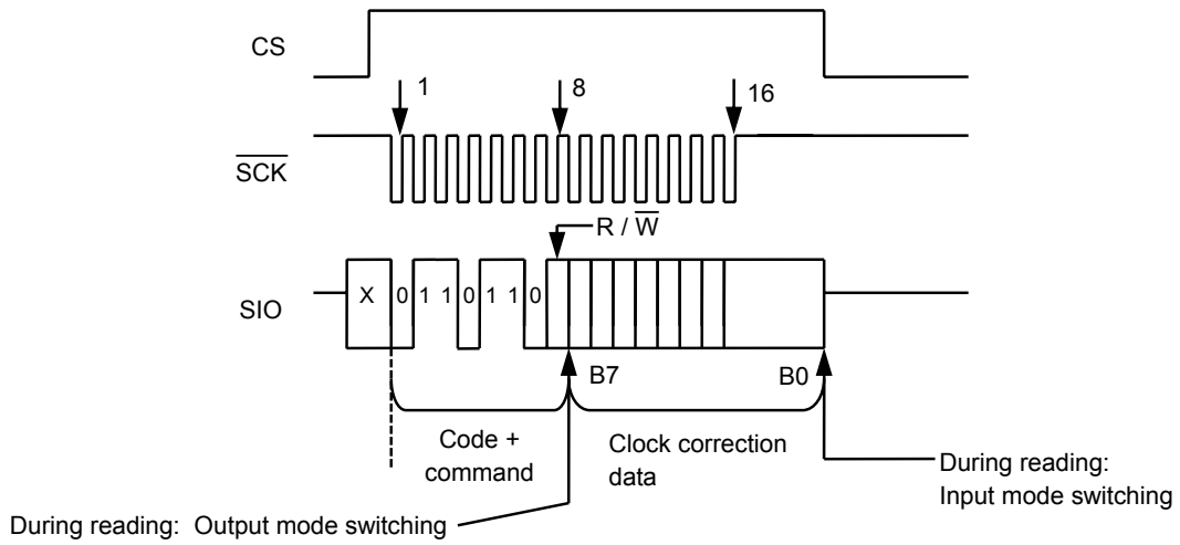
Figure 46 Clock Correction Register Access
