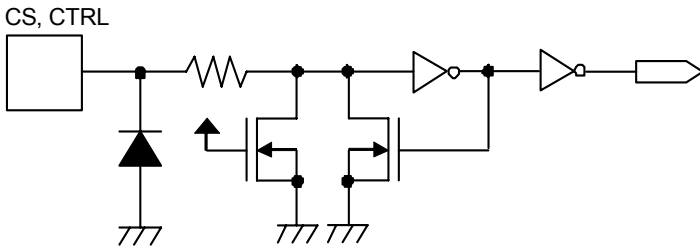
Figure 5 CS pin, CTRL pin
