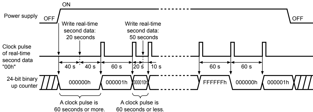
Figure 40 Timing Chart of 24-Bit Binary Up Counter
