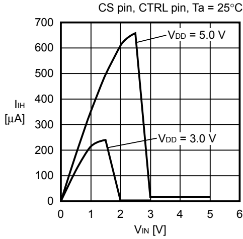
(13) Input current characteristics 3 ( V_{IN} vs. I_{IH} )
