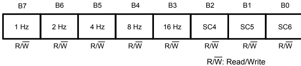
Figure 18 INT Register 1 (Data register for output frequency)
