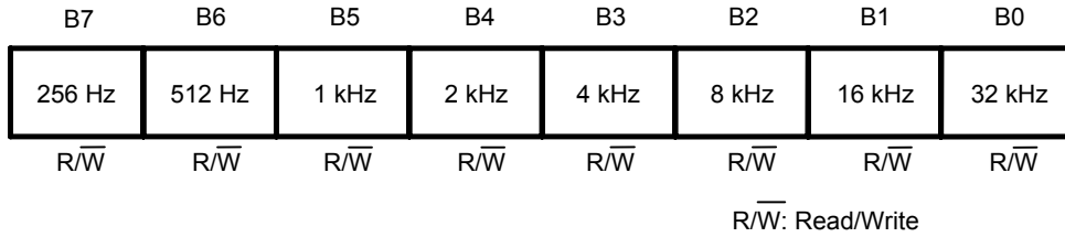
Figure 23 FOUT Setting Register 1
