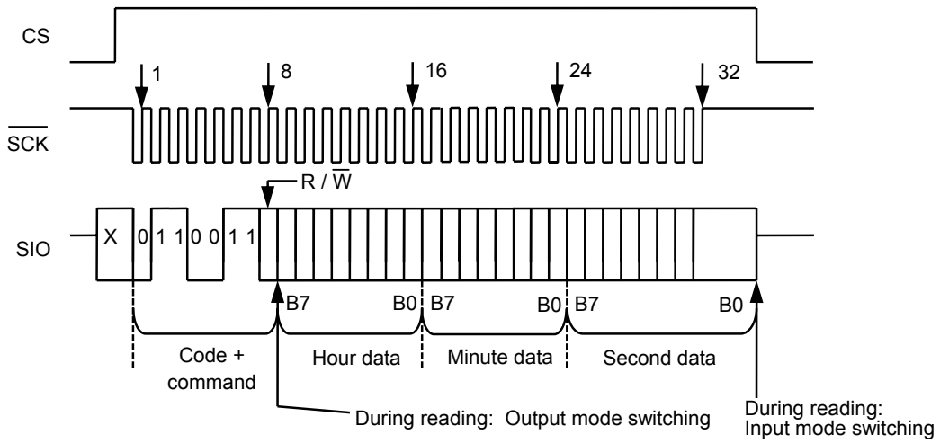
Figure 42 Real-Time Data Access 2
