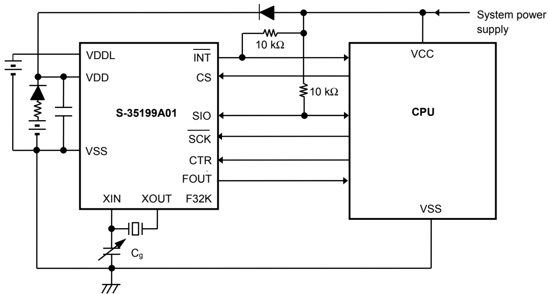
Figure 53 Application Circuit 2
