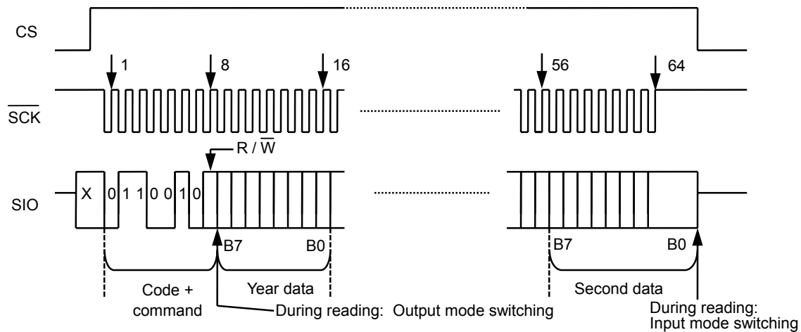
Figure 41 Real-Time Data Access 1
