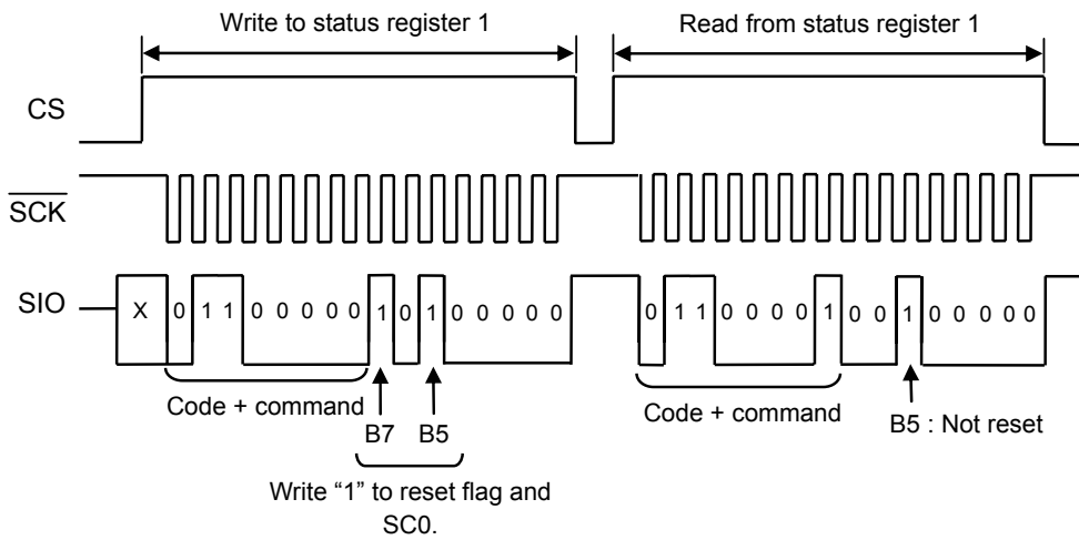
Figure 28 Data of Status Register 1 at Initialization
