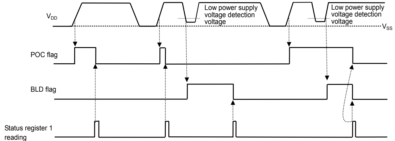
Figure 30 POC Flag and BLD Flag
