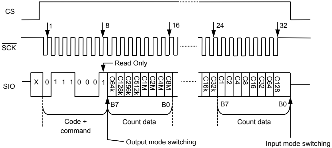
Figure 48 Up Counter Access
