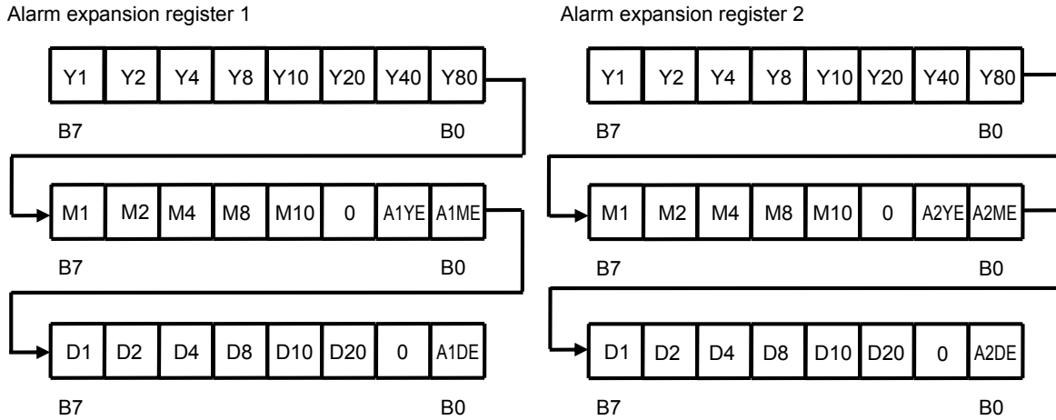
Figure 26 Alarm Expansion Register 1, Alarm Expansion Register 2
