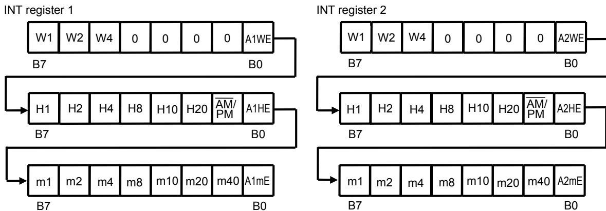
Figure 17 INT Register 1 and 2 (Alarm-Time Data)
