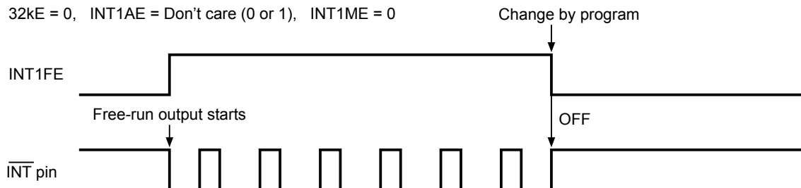
Figure 33 Output Timing of User-set Frequency
