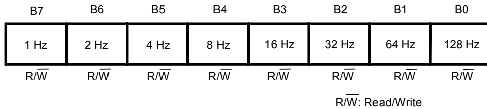
Figure 24 FOUT Setting Register 2
