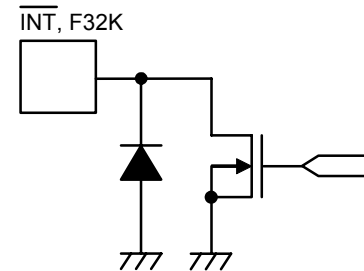
Figure 6 \overline{\text{INT}} pin, F32K pin
