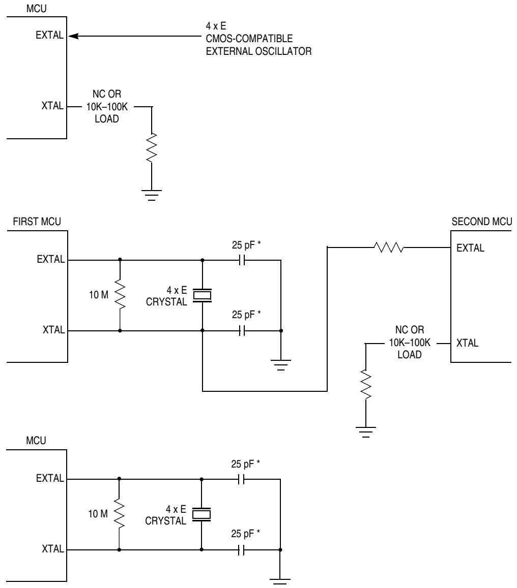
Figure 1-5. Oscillator Connections
