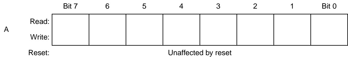
Figure 7-2. Accumulator (A)
