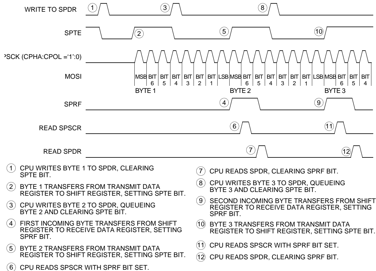
Figure 17-10. SPFR/SPTe CPU Interrupt Timing
