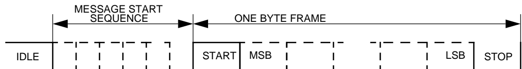
Figure 28 Byteflight™ Message Start Sequence
