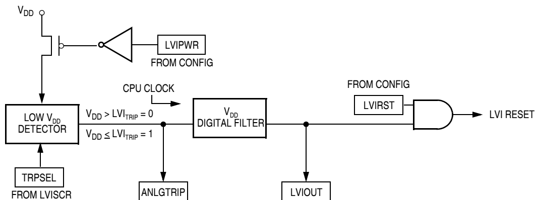
Figure 18-1. LVI Module Block Diagram
