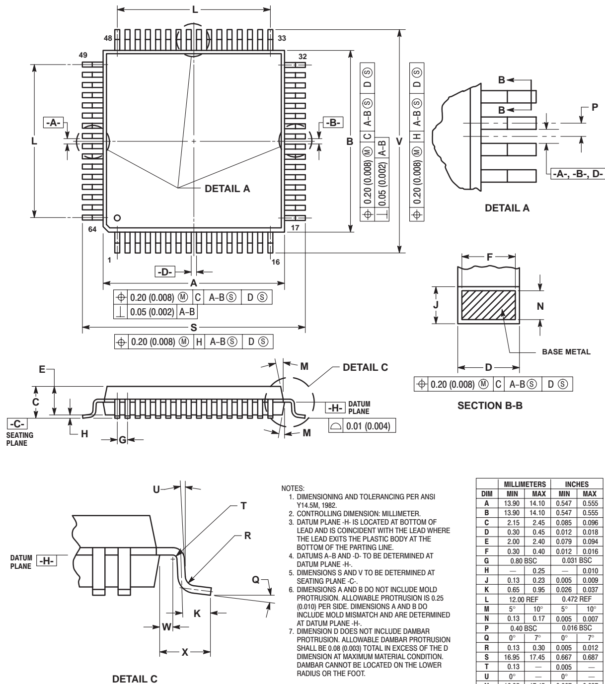
Figure 22-1. MC68HC908MR24FU
