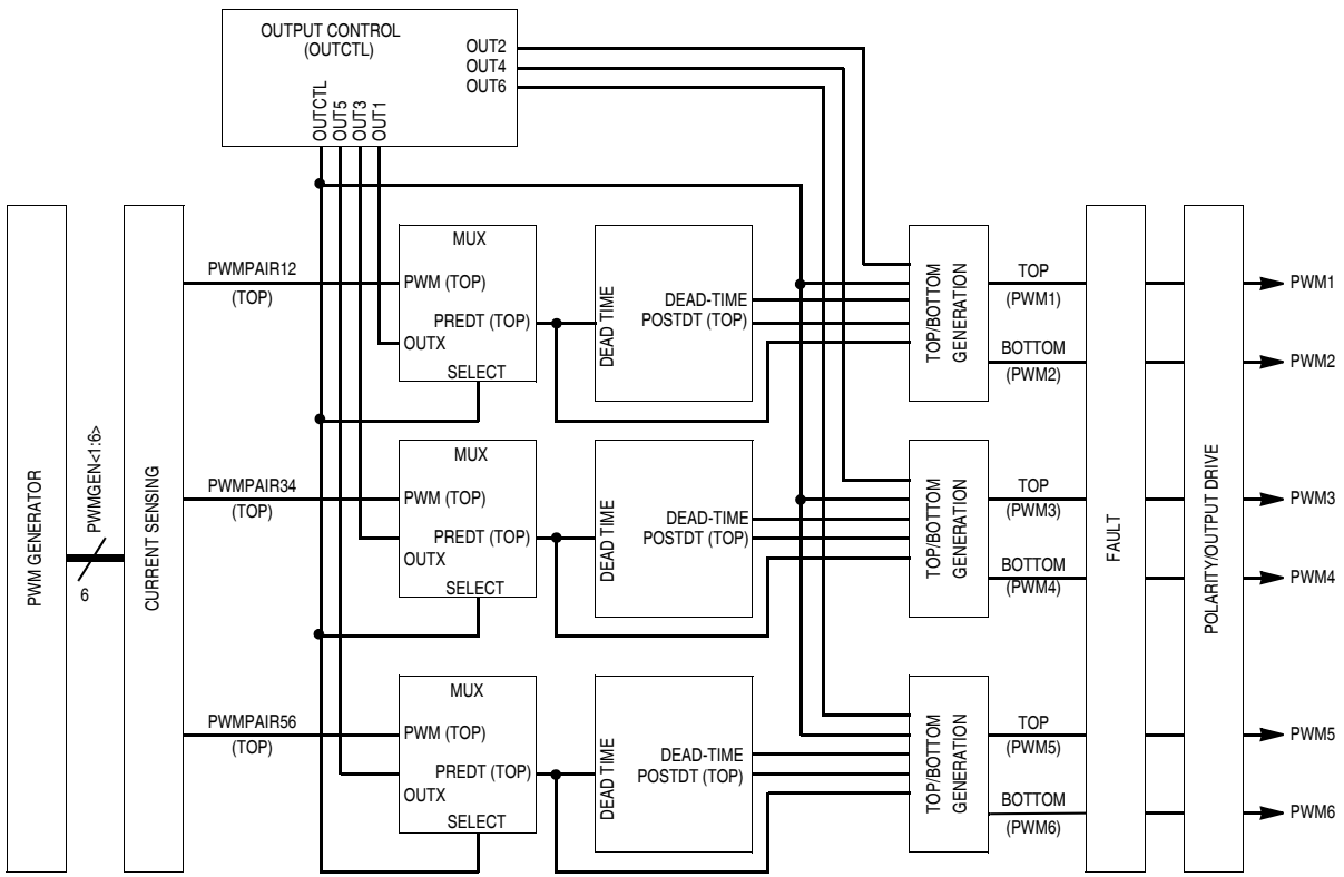
Figure 9-13. Dead-Time Generators
