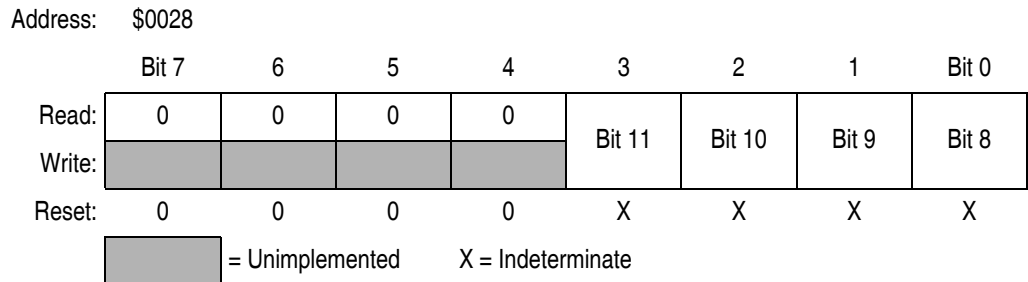
Figure 9-34. PWM Counter Modulo Register High (PMDH)
