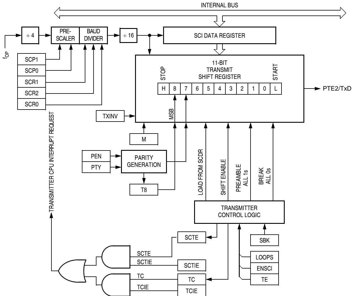
Figure 14-4. SCI Transmitter
