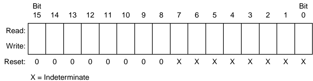
Figure 6-3. Index Register (H:X)
