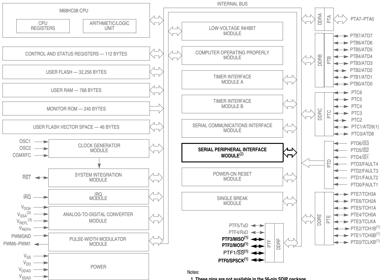
Figure 15-1. Block Diagram Highlighting SPI Block and Pins
