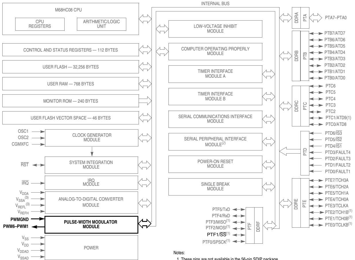
Figure 12-1. Block Diagram Highlighting PWM Module and Pins
