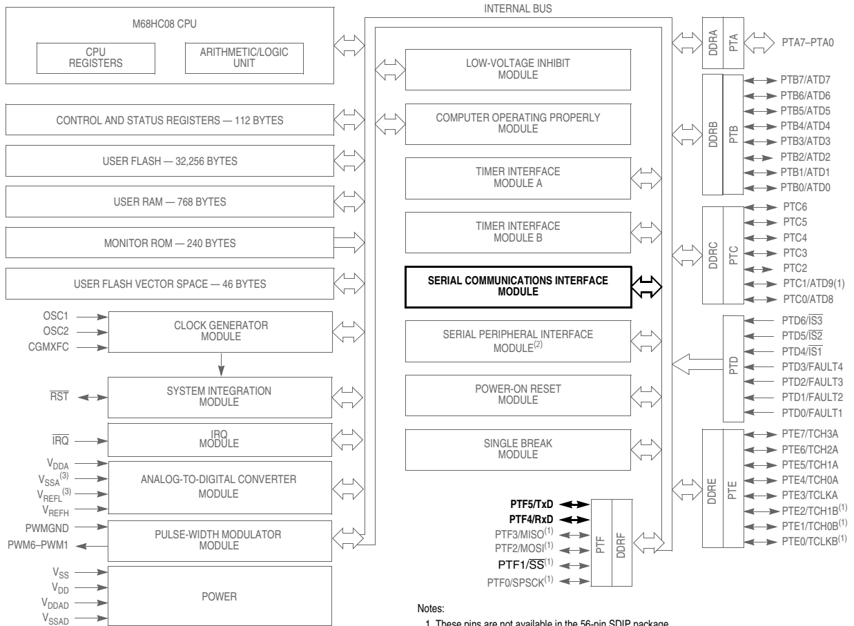
Figure 13-1. Block Diagram Highlighting SCI Block and Pins
