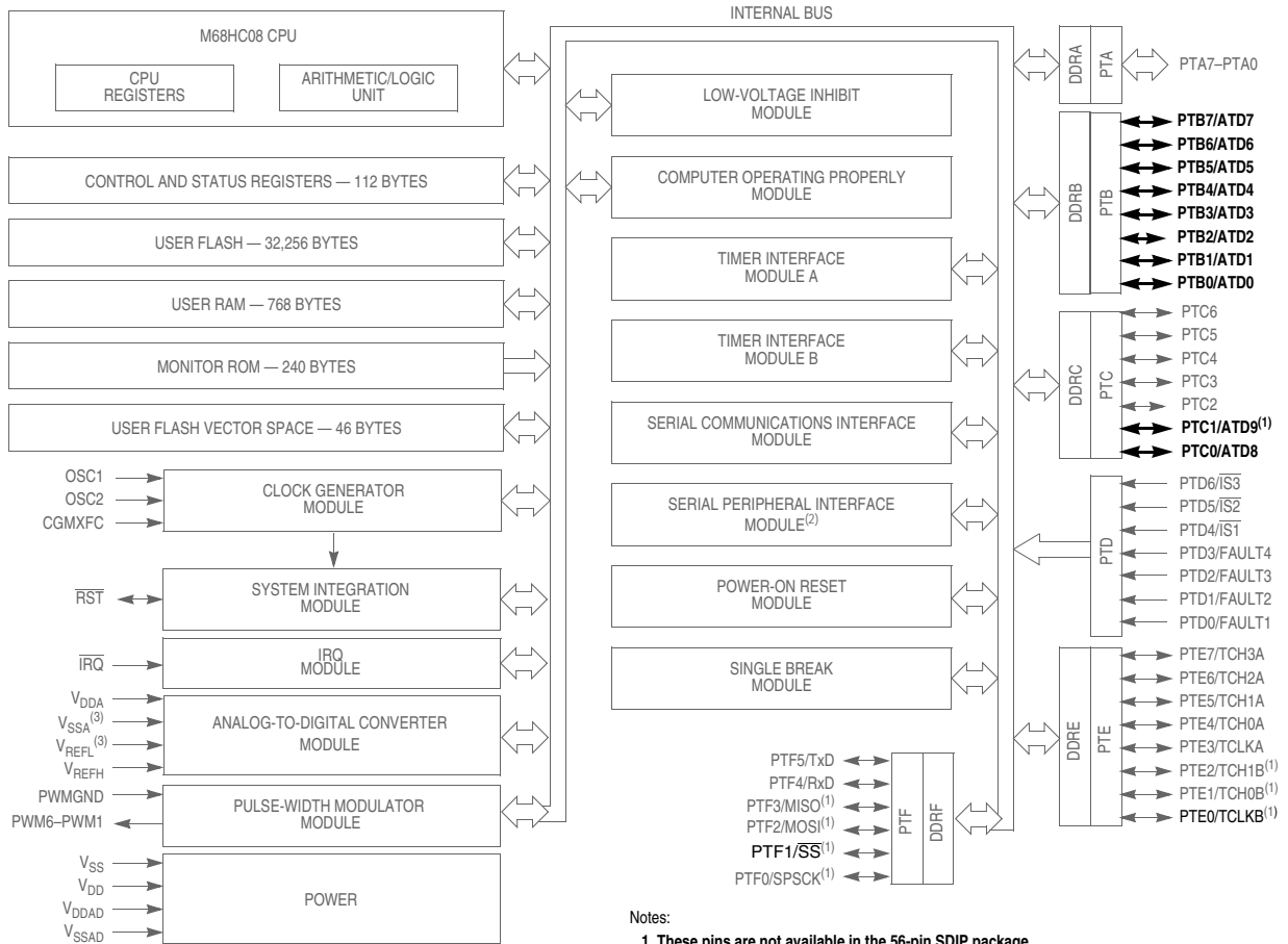
Figure 3-1. Block Diagram Highlighting ADC Block and Pins
