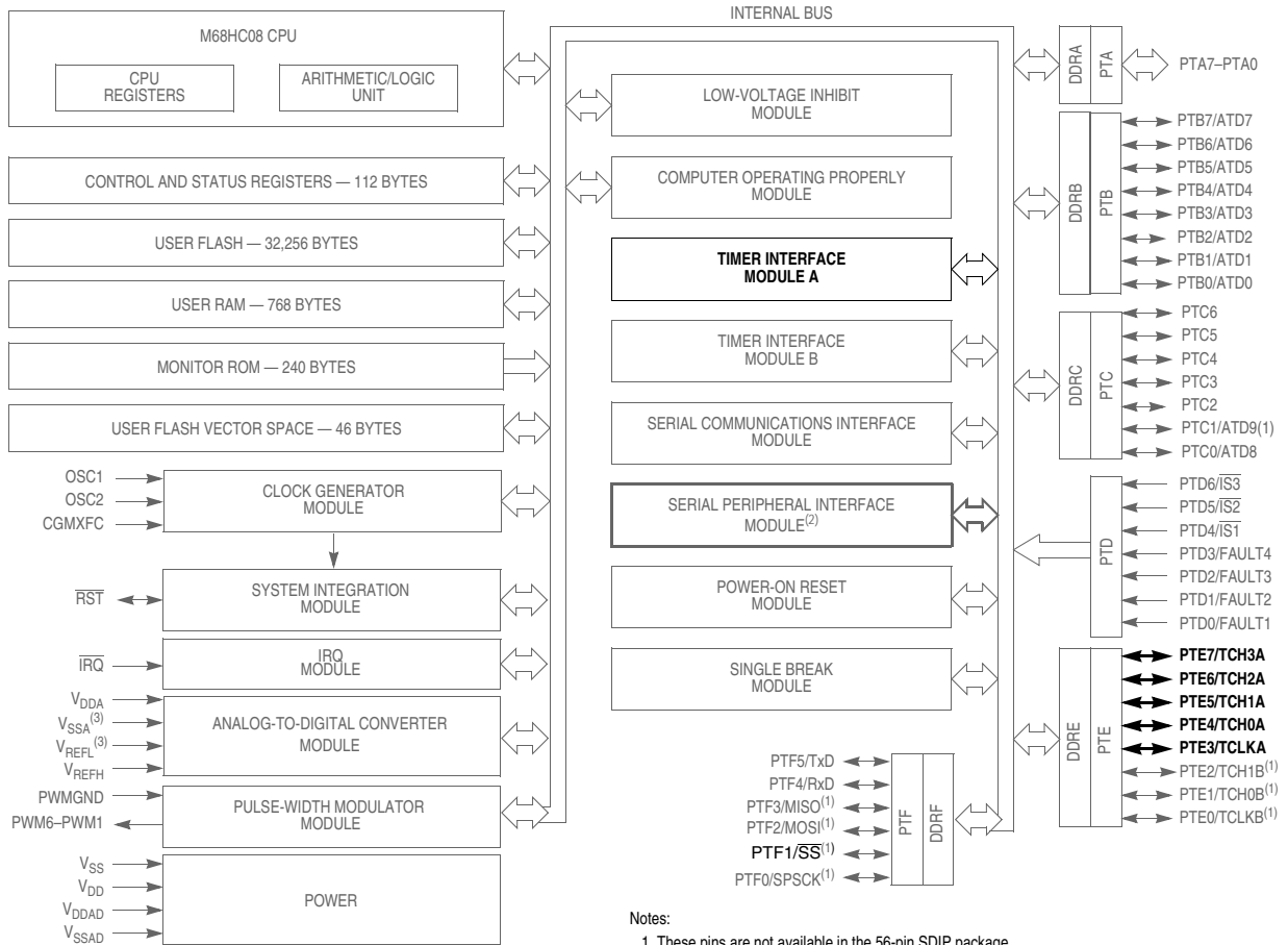
Figure 16-1. Block Diagram Highlighting TIMA Block and Pins
