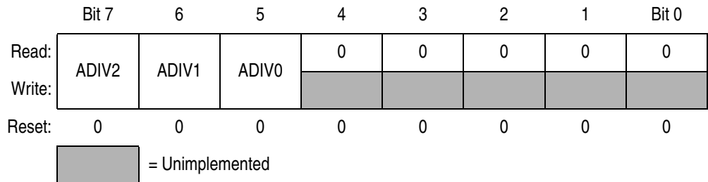
Figure 13-5. ADC Input Clock Register (ADICLK)
