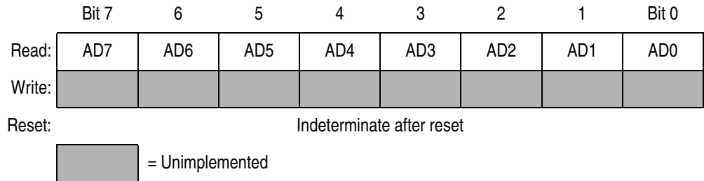
Figure 13-4. ADC Data Register (ADR)
