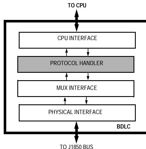
Figure 21-13. BDLC Block Diagram
