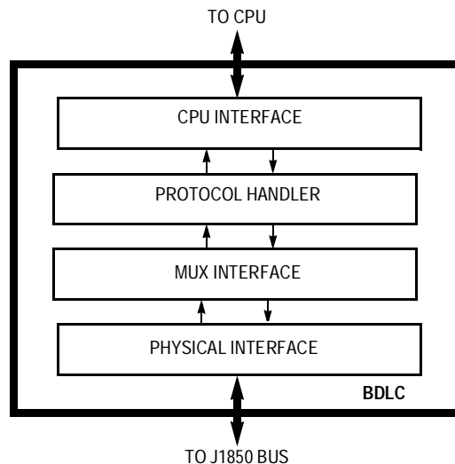
Figure 21-1. BDLC Block Diagram
