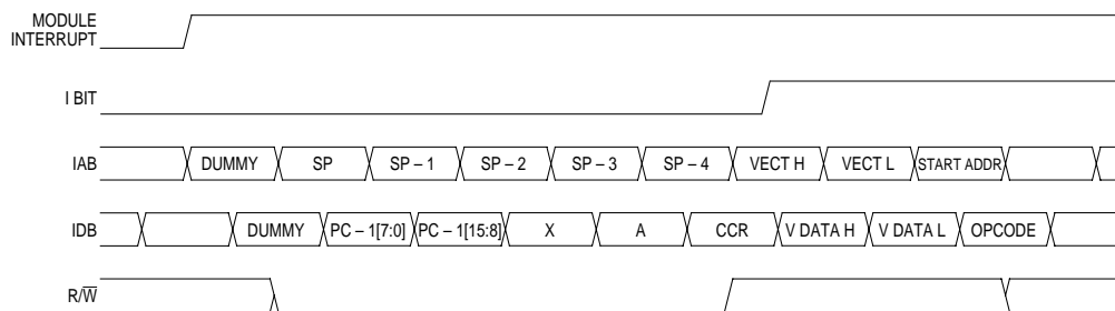
Figure 7-9. Interrupt Entry
