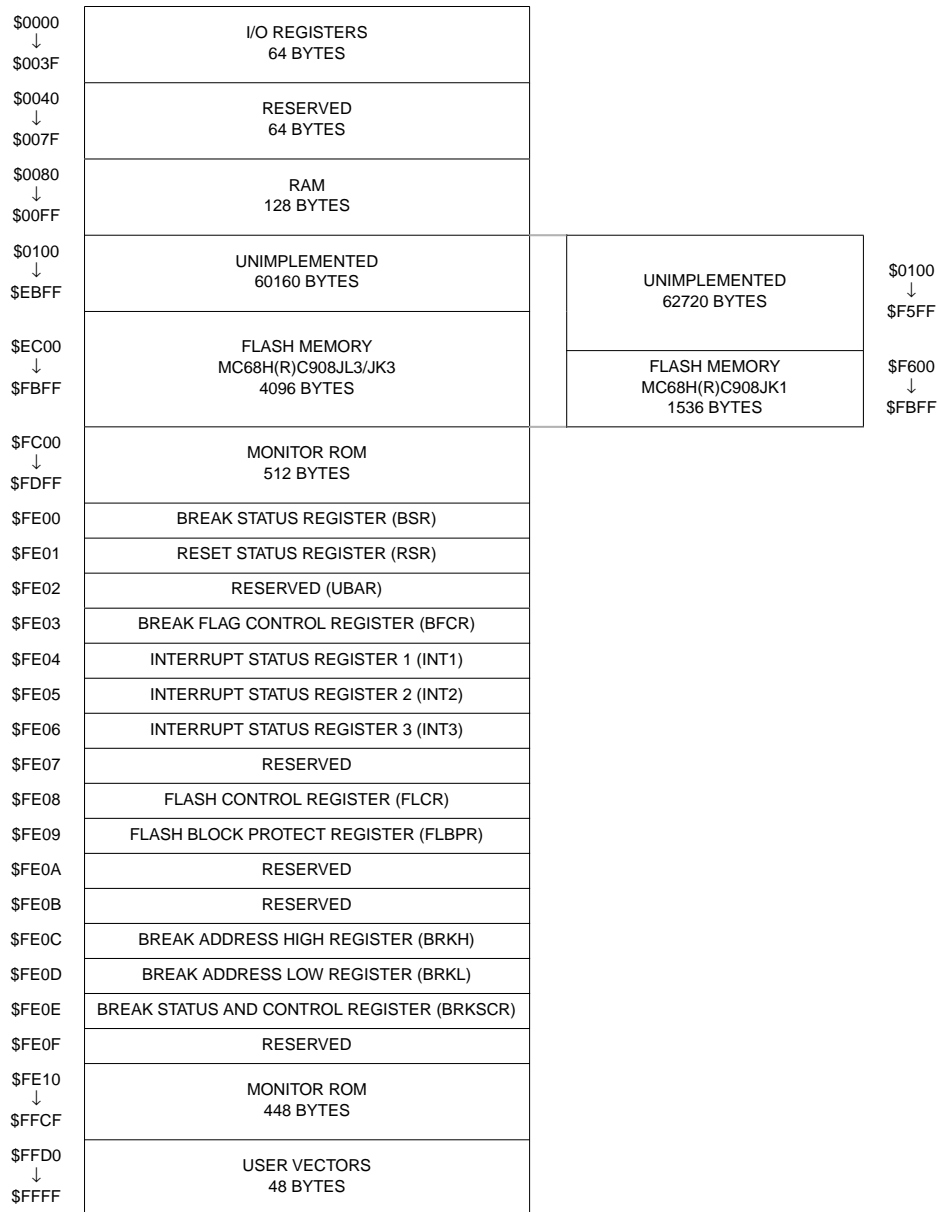
Figure 2-1. Memory Map
