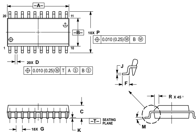
Figure 19-2. 20-Pin SOIC (Case #751D)
