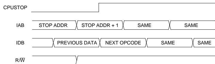
Figure 7-18. Stop Mode Entry Timing
