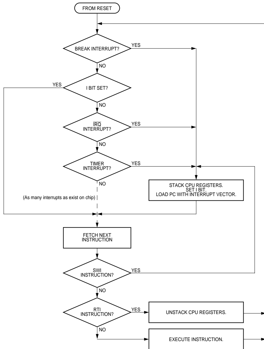
Figure 7-8. Interrupt Processing
