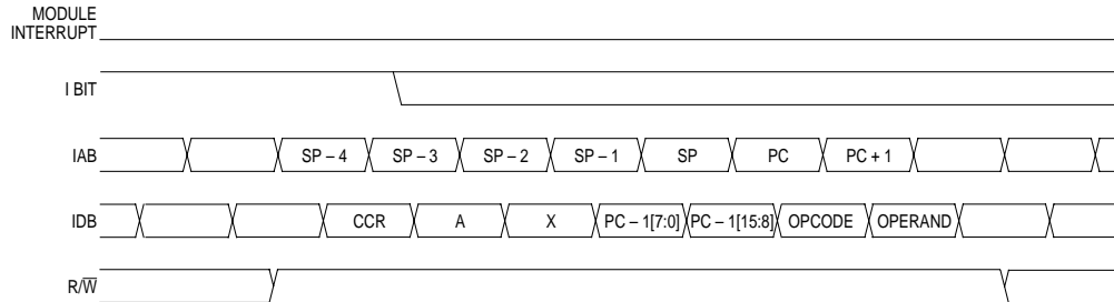
Figure 7-10. Interrupt Recovery
