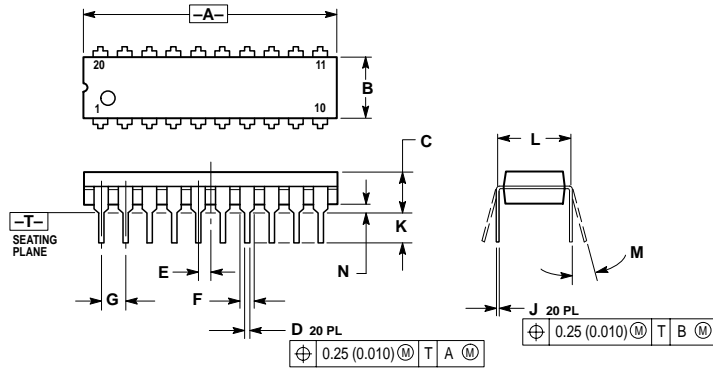
Figure 19-1. 20-Pin PDIP (Case #738)
