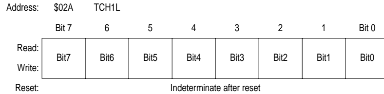
Figure 10-9. TIM Channel Registers (TCH0H/L:TCH1H/L)
