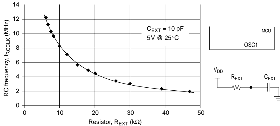
Figure 18-1. RC vs. Frequency (5V @ 25°C)
