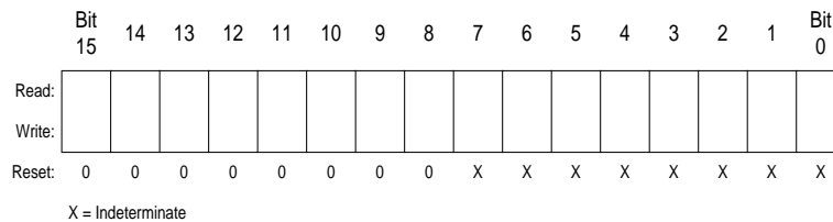
Figure 6-3. Index Register (H:X)
