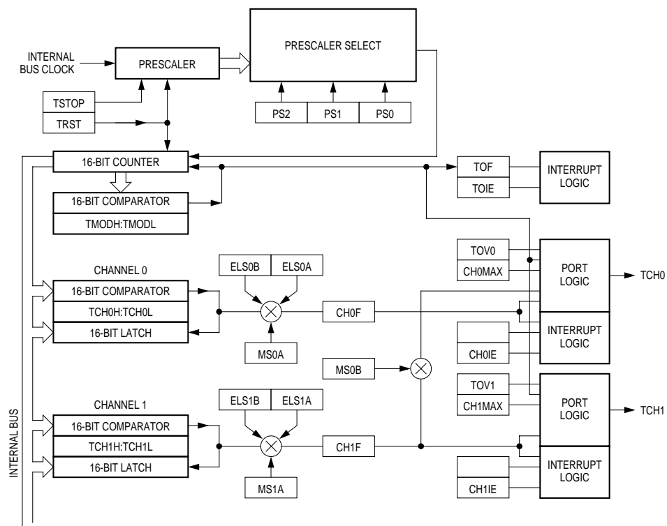
Figure 10-1. TIM Block Diagram
