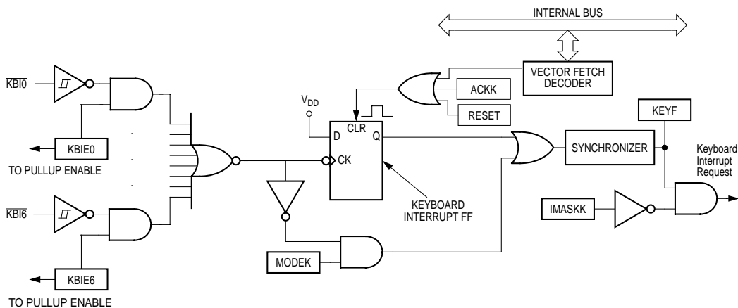
Figure 14-2. Keyboard Interrupt Block Diagram
