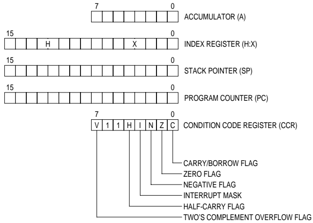
Figure 6-1. CPU Registers
