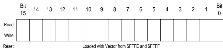
Figure 6-5. Program Counter (PC)
