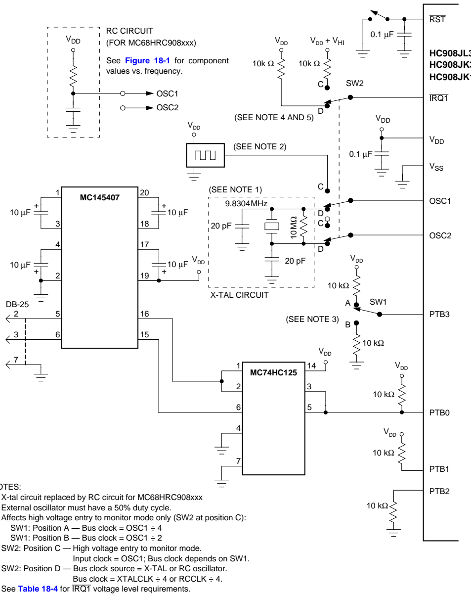
Figure 9-1. Monitor Mode Circuit
