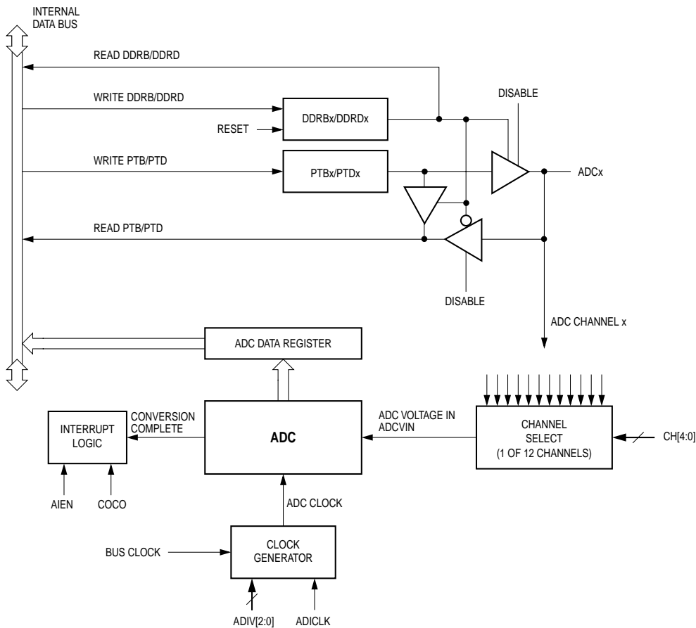
Figure 11-2. ADC Block Diagram
