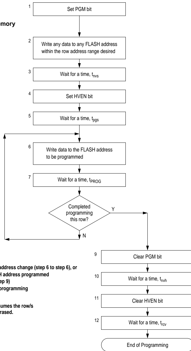
Figure 4-2. FLASH Programming Flowchart
