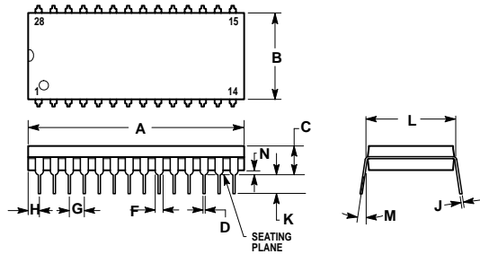
Figure 19-3. 28-Pin PDIP (Case #710)
