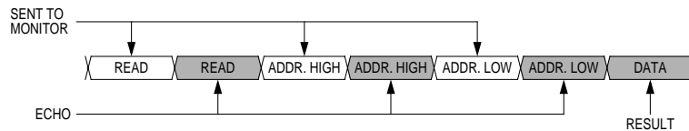
Figure 9-5. Read Transaction
