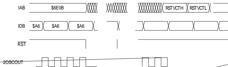
Figure 7-17. Wait Recovery from Internal Reset
