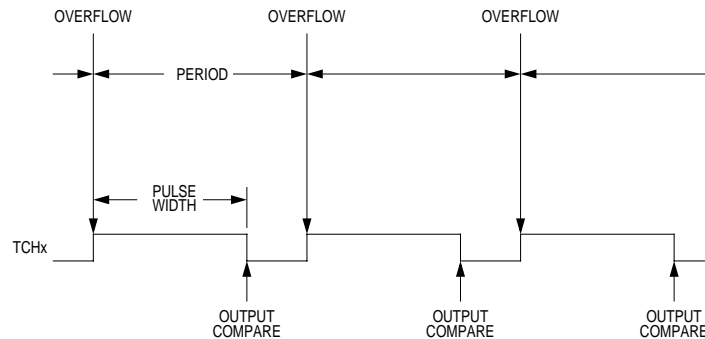
Figure 10-3. PWM Period and Pulse Width
