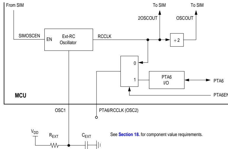
Figure 8-2. RC Oscillator External Connections
