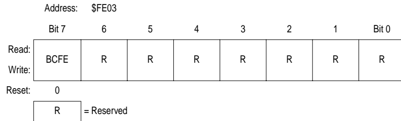
Figure 7-22. Break Flag Control Register (BFCR)
