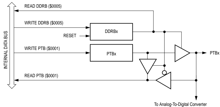
Figure 12-8. Port B I/O Circuit
