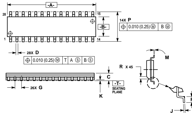
Figure 19-4. 28-Pin SOIC (Case #751F)
