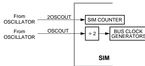
Figure 7-3. SIM Clock Signals
