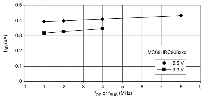
Figure 18-5. Typical Stop Mode I_{DD} , with all Modules Disabled (25 °C)
