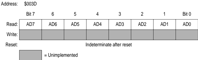
Figure 11-4. ADC Data Register (ADR)
