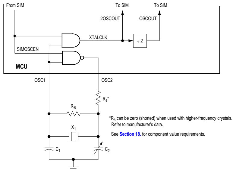
Figure 8-1. X-tal Oscillator External Connections
