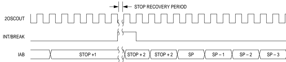
Figure 7-19. Stop Mode Recovery from Interrupt or Break
