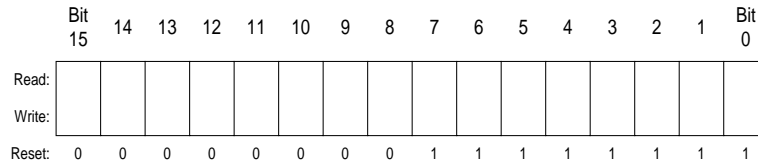
Figure 6-4. Stack Pointer (SP)
