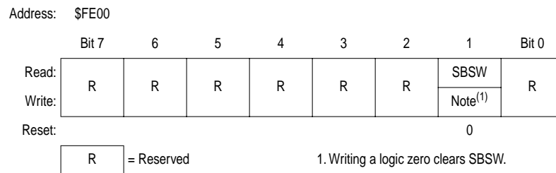
Figure 7-20. Break Status Register (BSR)
