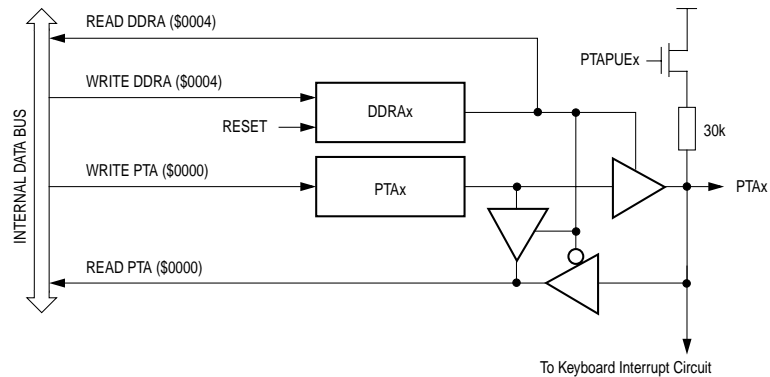
Figure 12-4. Port A I/O Circuit
