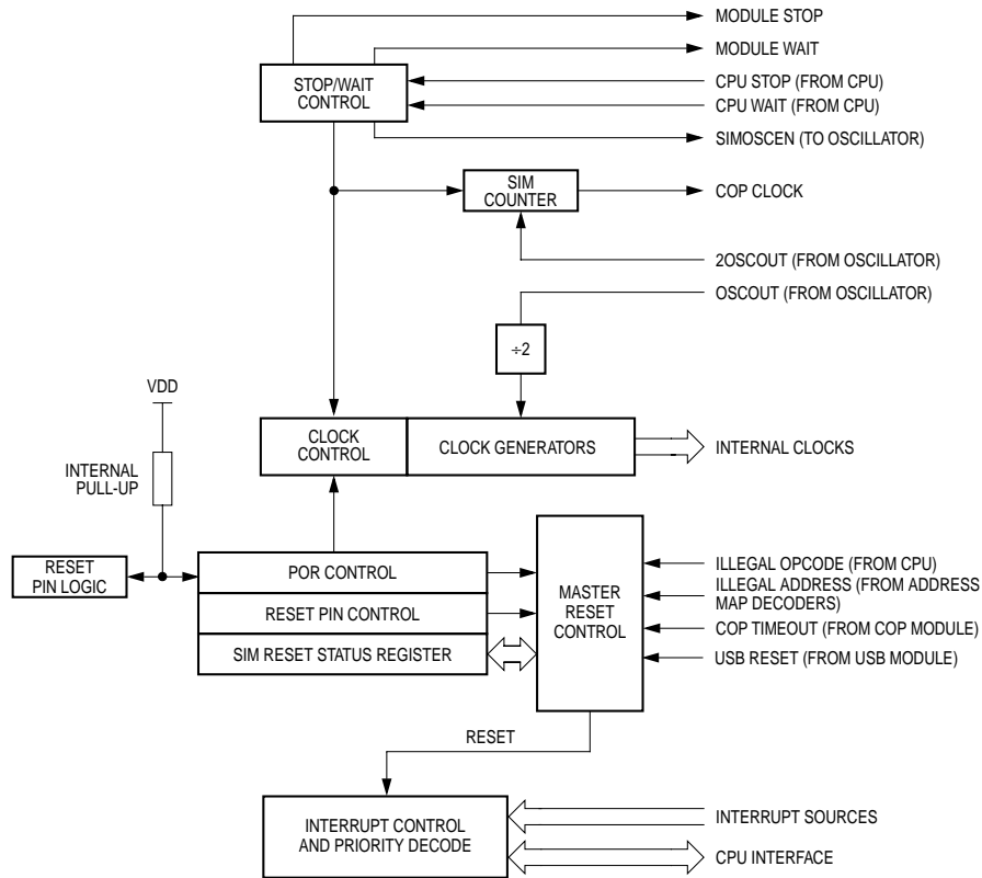
Figure 7-1. SIM Block Diagram
