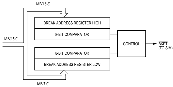
Figure 17-1. Break Module Block Diagram
