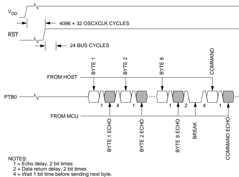
Figure 9-7. Monitor Mode Entry Timing
