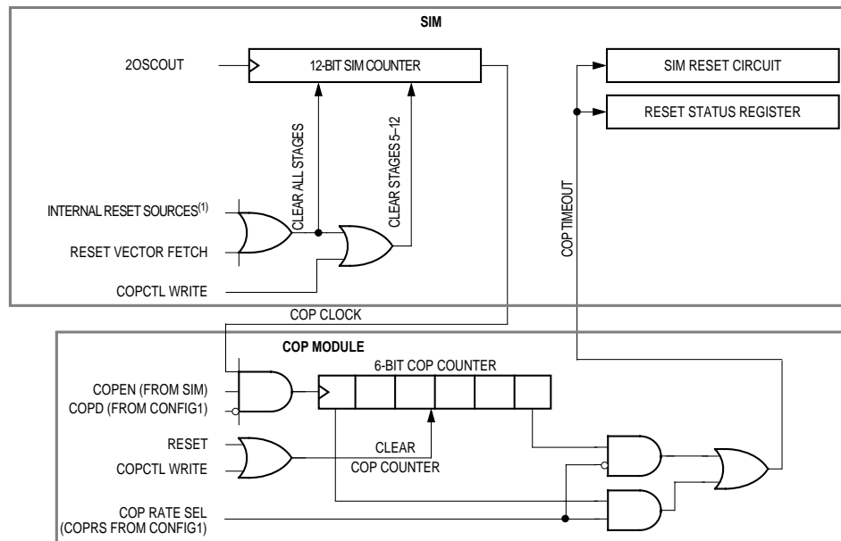
Figure 15-1. COP Block Diagram
