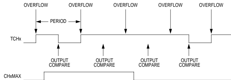
Figure 10-8. CHxMAX Latency
