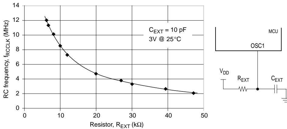
Figure 18-2. RC vs. Frequency (3V @ 25°C)
