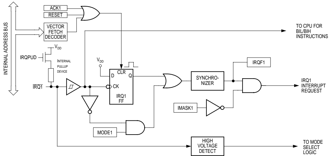
Figure 13-1. IRQ Module Block Diagram
