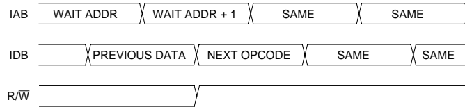
Figure 7-15. Wait Mode Entry Timing
