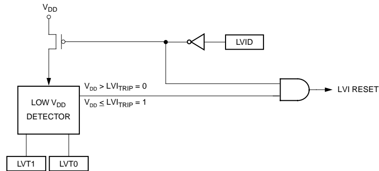
Figure 16-1. LVI Module Block Diagram
