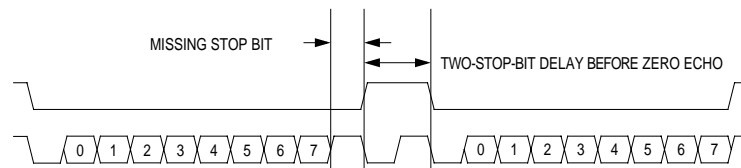
Figure 9-6. Break Transaction
