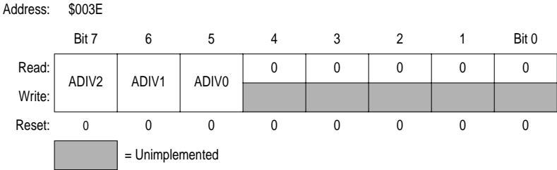
Figure 11-5. ADC Input Clock Register (ADICLK)
