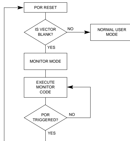
Figure 9-2. Low-Voltage Monitor Mode Entry Flowchart
