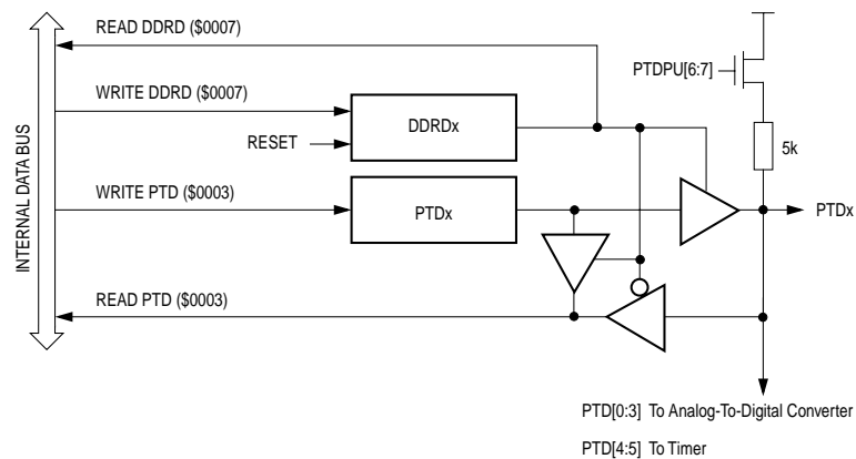
Figure 12-11. Port D I/O Circuit
