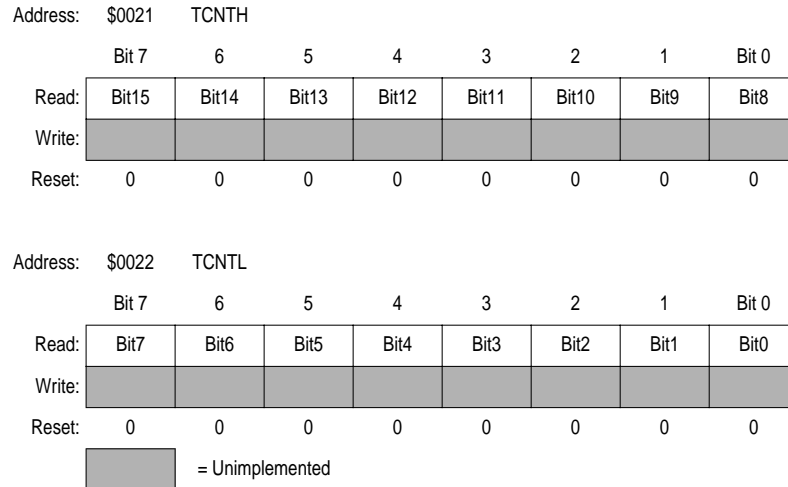
Figure 10-5. TIM Counter Registers (TCNTH:TCNTL)
