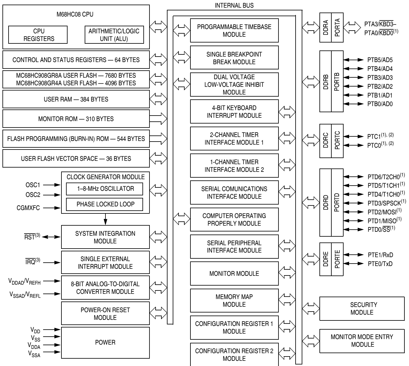
Figure 1-1 shows the structure of the MC68HC908GR8A.
