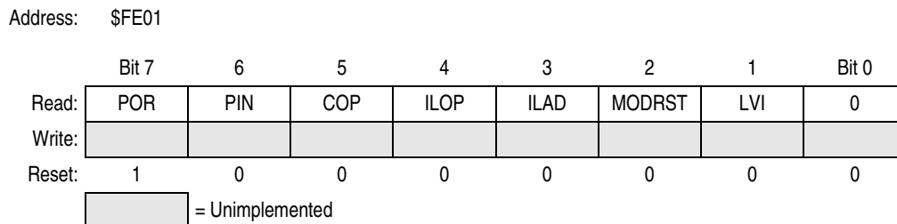
Figure 16-21. SIM Reset Status Register (SRSR)
