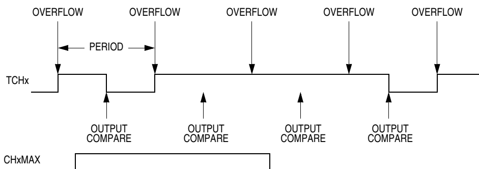
Figure 19-12. CHxMAX Latency
