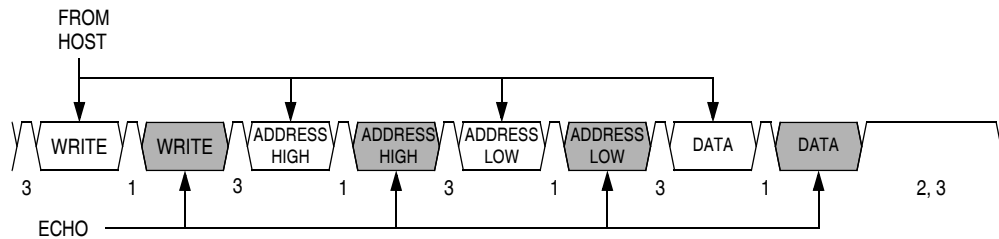
Figure 17-15. Read Transaction
