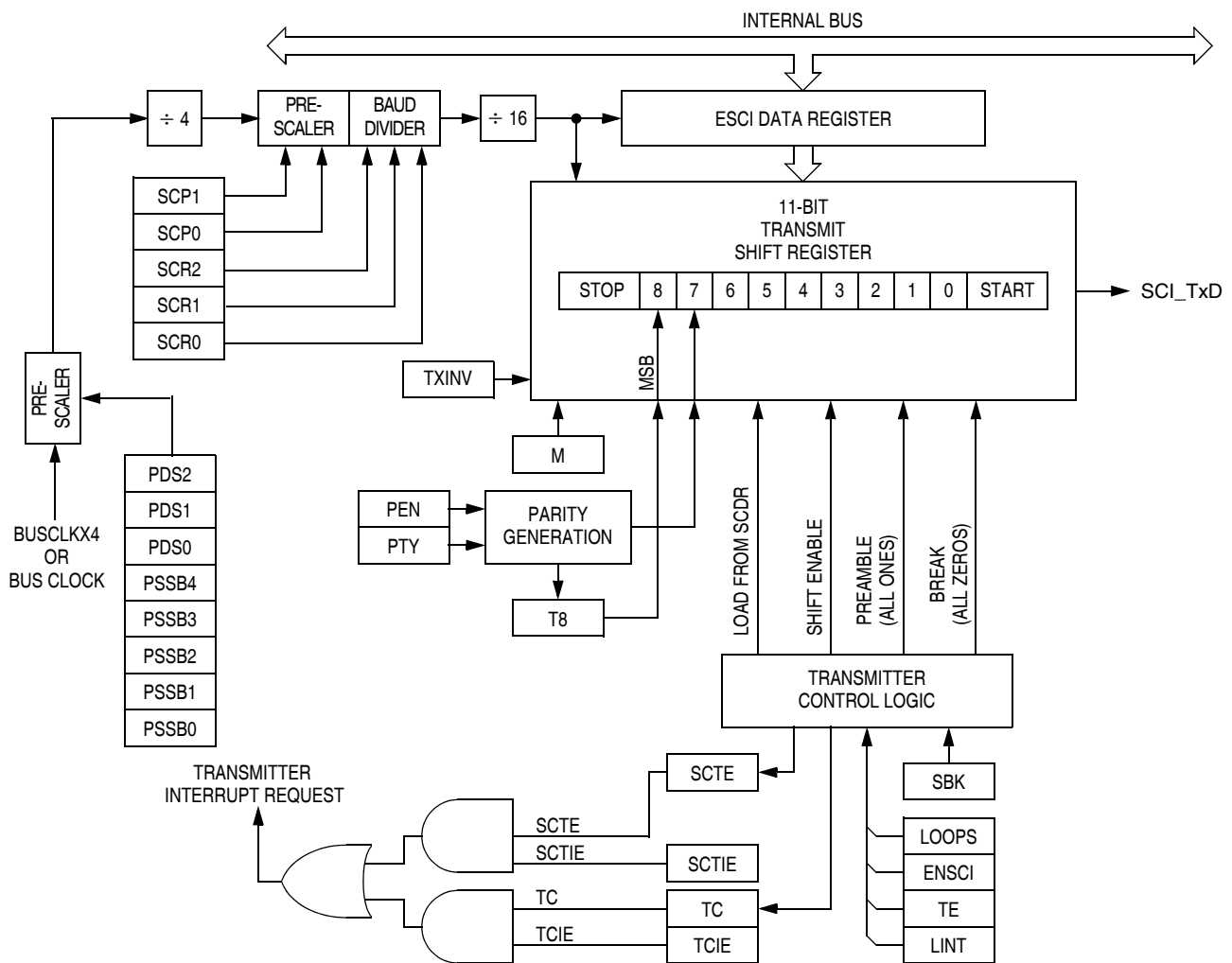
Figure 13-4. ESCI Transmitter
