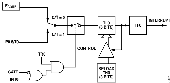
Figure 71. Timer/Counter 0, Mode 2
