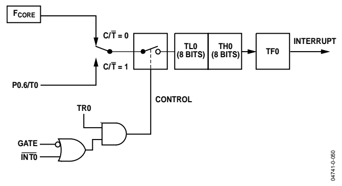
Figure 70. Timer/Counter 0, Mode 1
