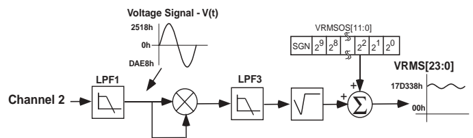
Figure 26 - Channel 2 RMS signal processing
