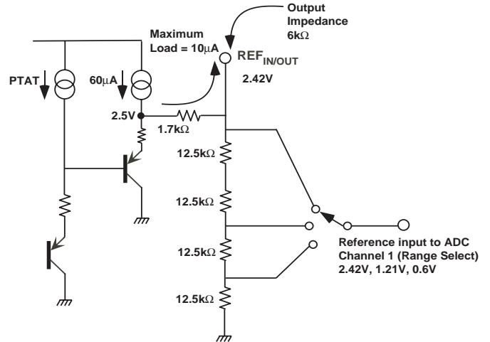
Figure 20—ADE7753 Reference Circuit Output
