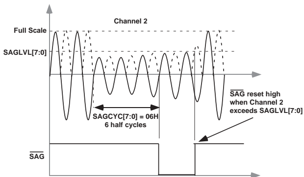
Figure 13 - ADE7753 Sag detection
