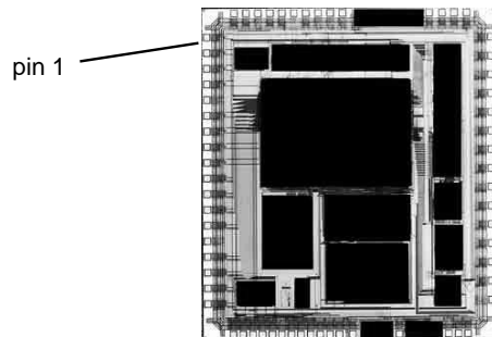
Figure 10.2: Die. Chip size is 4.2 x 4.7mm 2 for 0.3 mm thickness. Physical chip size and exact pad positioning can change without notification.
