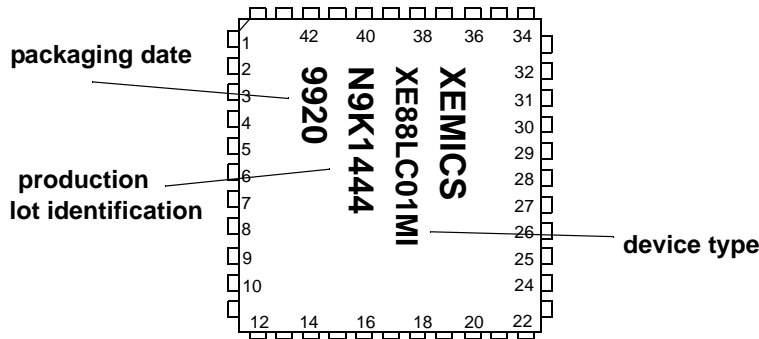
Figure 1.1: Pinout of the XE88LC01 in LQFP44 package
