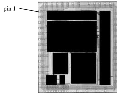
Figure 9.3: XE88LC01 in die: 4.1 x 4.6 mm 2
