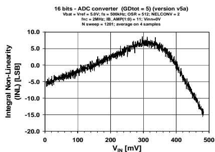
Figure 8.12: GAIN=5, 16 bit ADC setting
