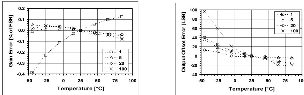
Figure 8.18: Gain and offset error vs temperature for several gains, normalized to 25°C, offset cancellation disabled. When the offset cancellation is enabled, the offset remains below the LSB in all temperature situations.
