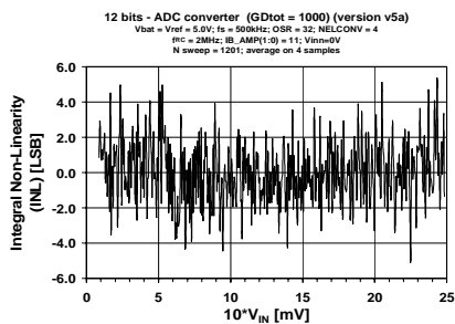
Figure 8.9: GAIN=1000, 12 bit ADC setting
