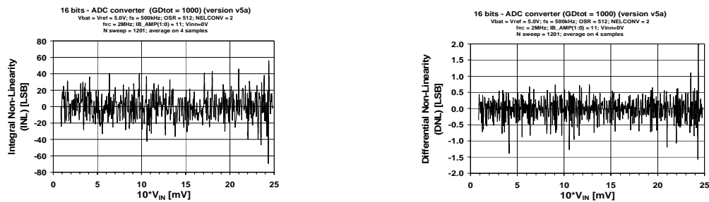
Figure 8.16: GAIN=1000, 16 bit ADC setting
