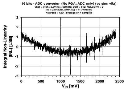
Figure 8.10: NO GAIN (ONLY ADC), 16 bit ADC setting
