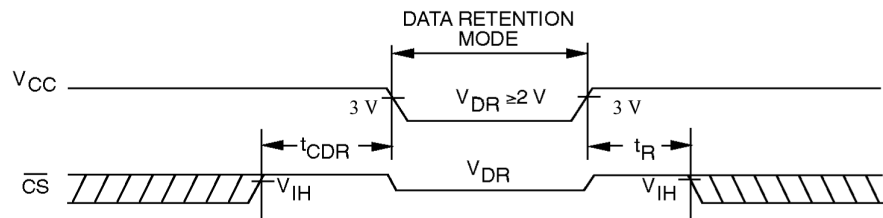
Figure 2. Data Retention Timing
