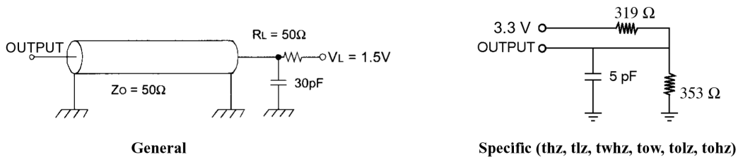
Figure 1. AC Test Loads Waveforms
