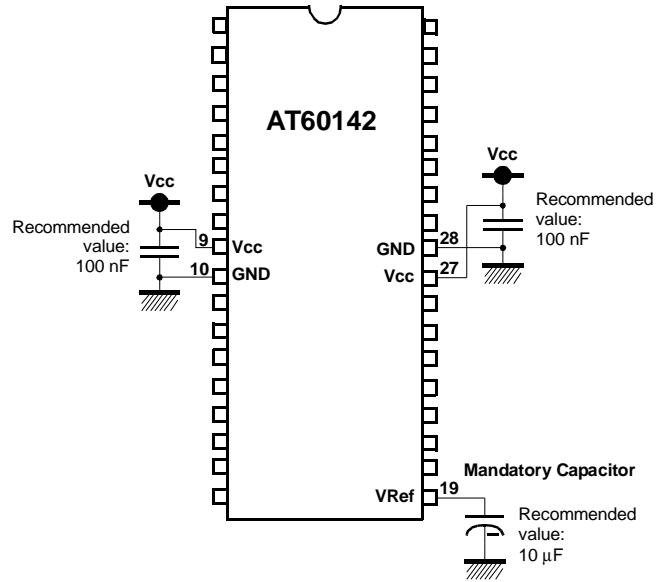
Decoupling capacitors closed to the device
