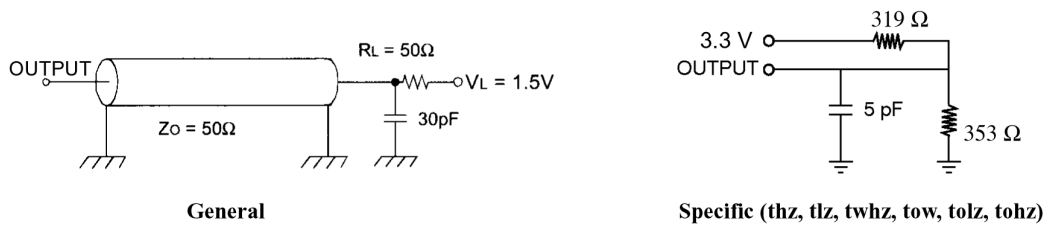
Figure 1. AC Test Loads Waveforms
