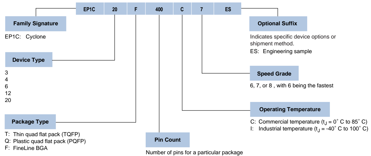
Figure 39. Cyclone Device Packaging Ordering Information
