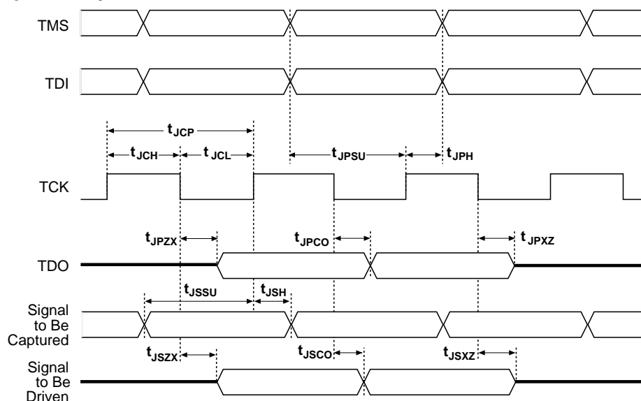
Figure 36. Cyclone JTAG Waveforms
