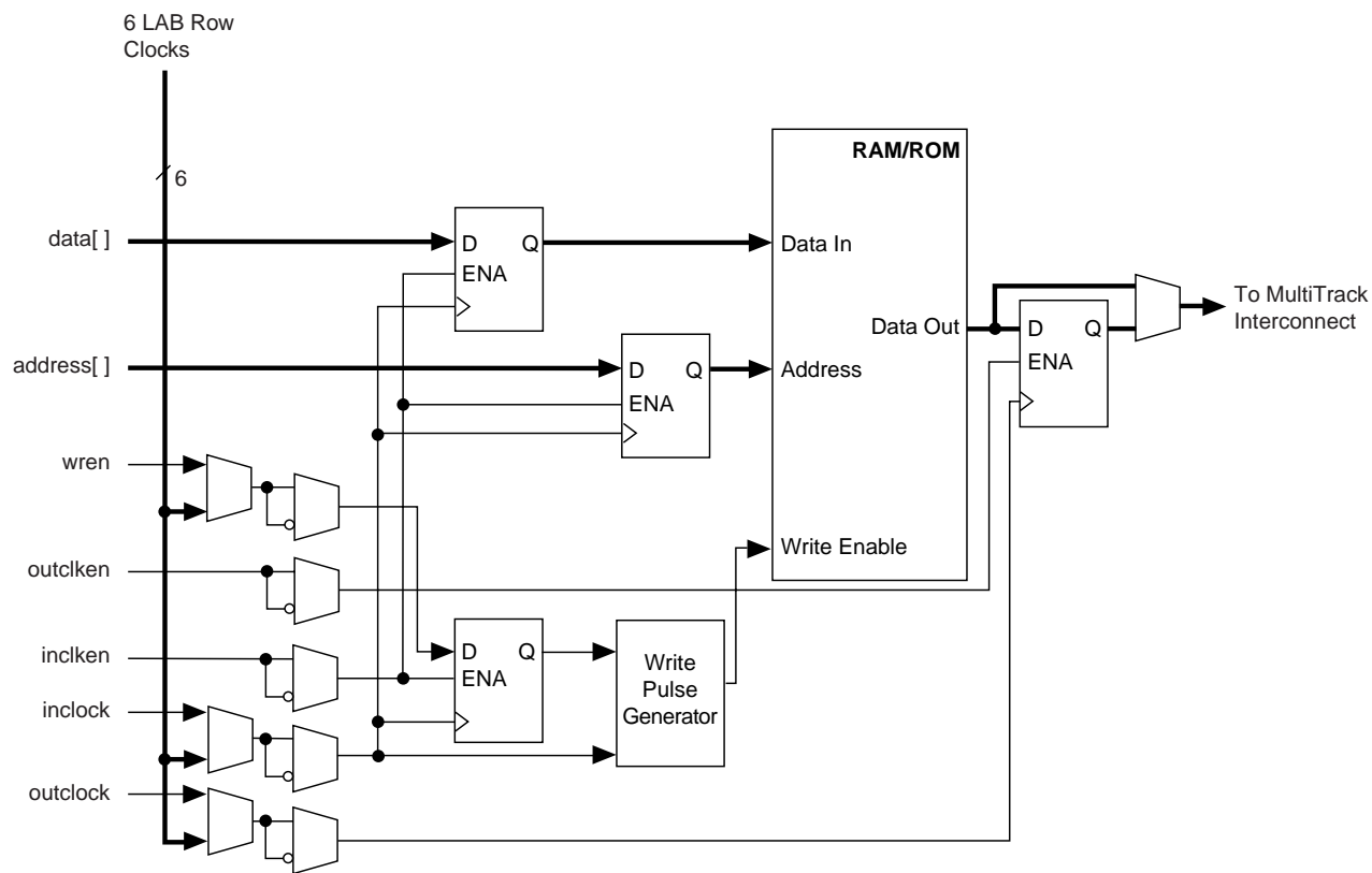
Figure 21. Single-Port Mode
