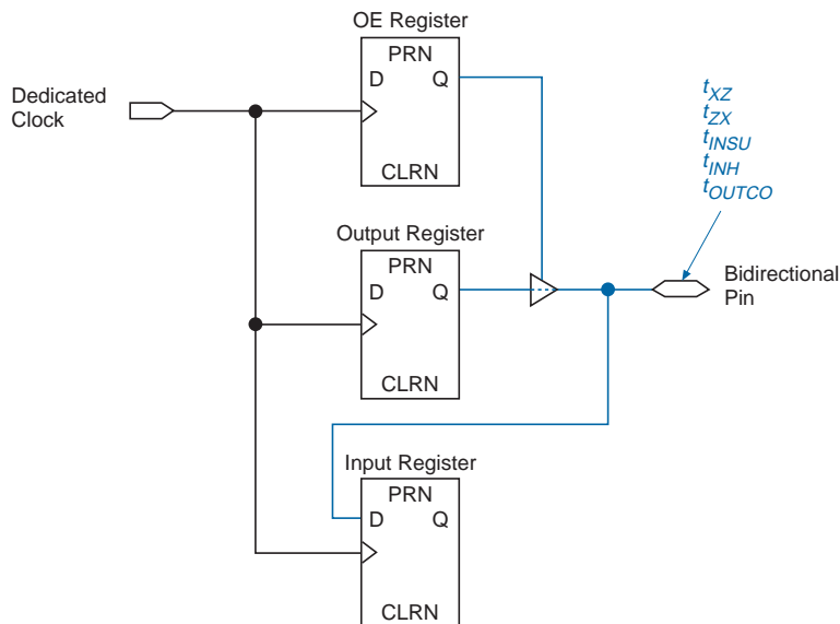
Figure 38. External Timing in Cyclone Devices
