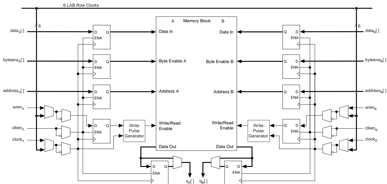
Figure 17. Independent Clock Mode Note (1)
