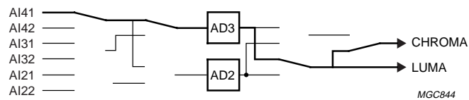
Fig.25 Mode 4; CVBS5.
