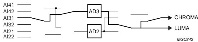
Fig.23 Mode 2; CVBS3.
