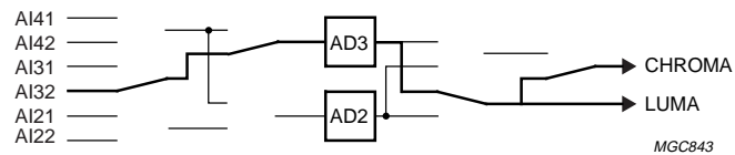
Fig.24 Mode 3; CVBS4.
