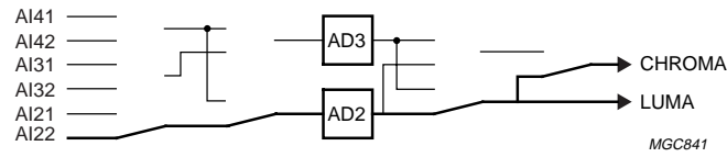
Fig.22 Mode 1; CVBS2.
