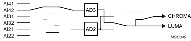
Fig.26 Mode 5; CVBS6.
