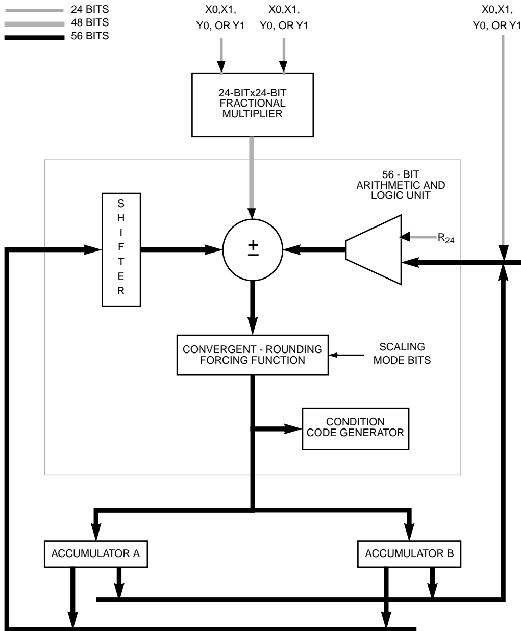
Figure 3-3 MAC Unit
