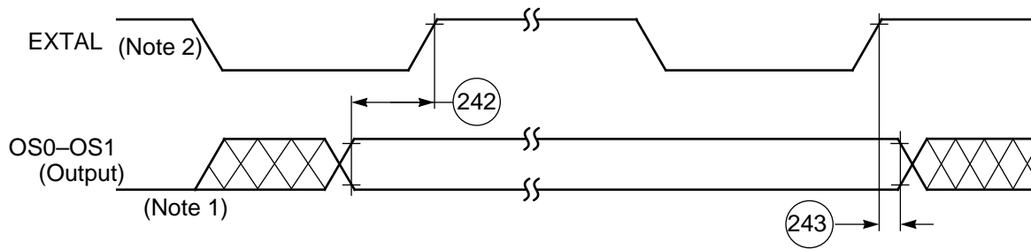
Figure 2-27 DSP56011 OnCE EXTAL to Status Timing
