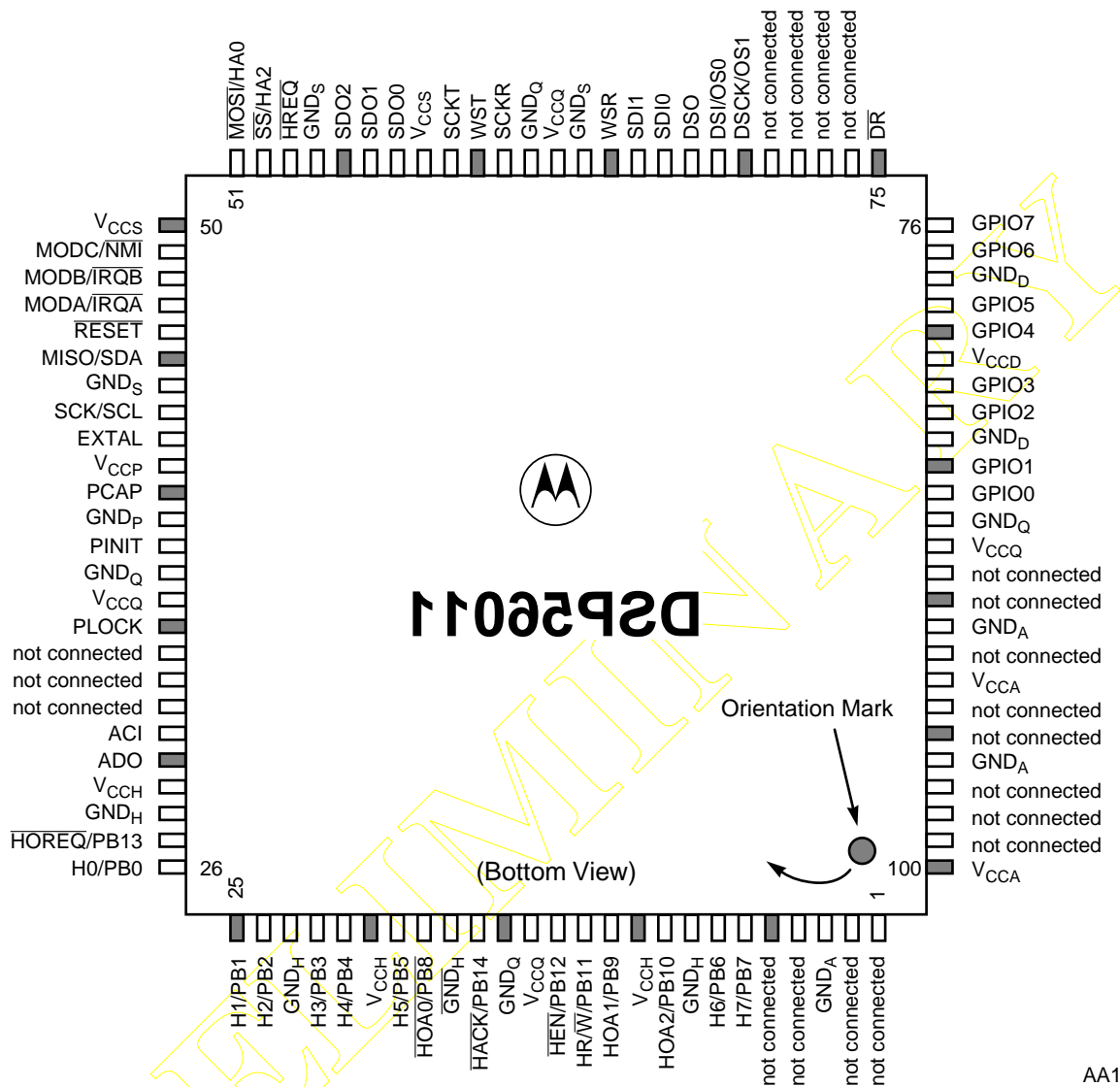
Figure 3-2 DSP56011 Thin Quad Flat Pack (TQFP), Bottom View
