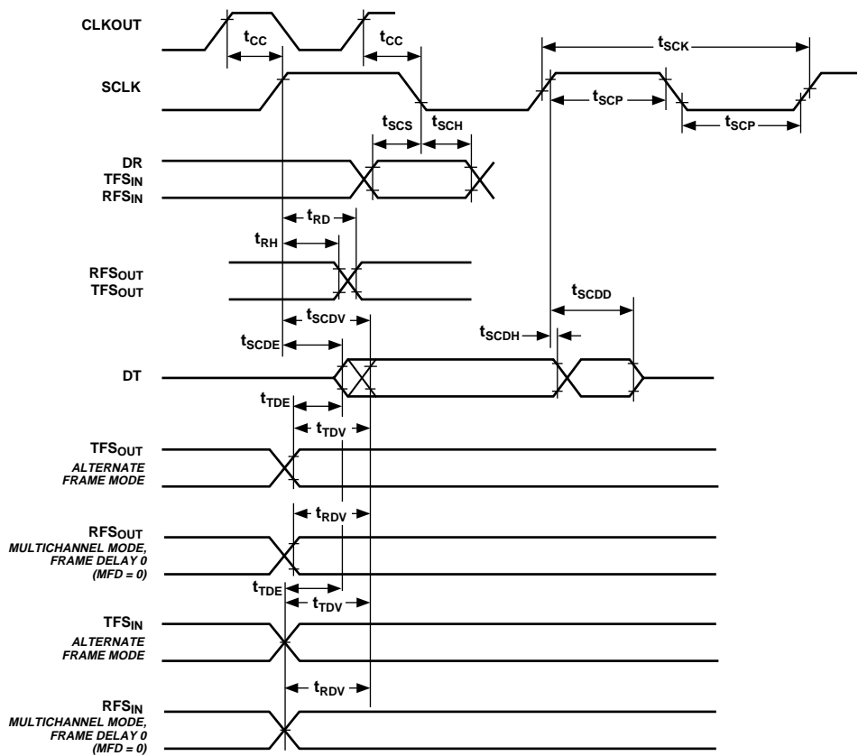
Figure 26. Serial Ports
