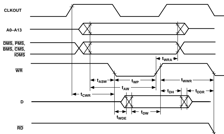
Figure 25. Memory Write
