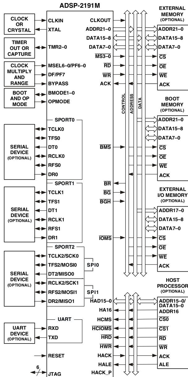
Figure 1. System Diagram
