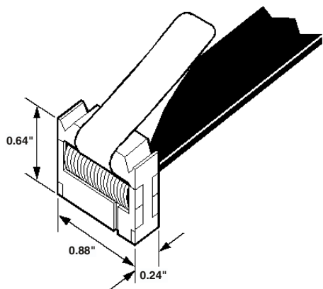
Figure 6. JTAG Pod Connector Dimensions
