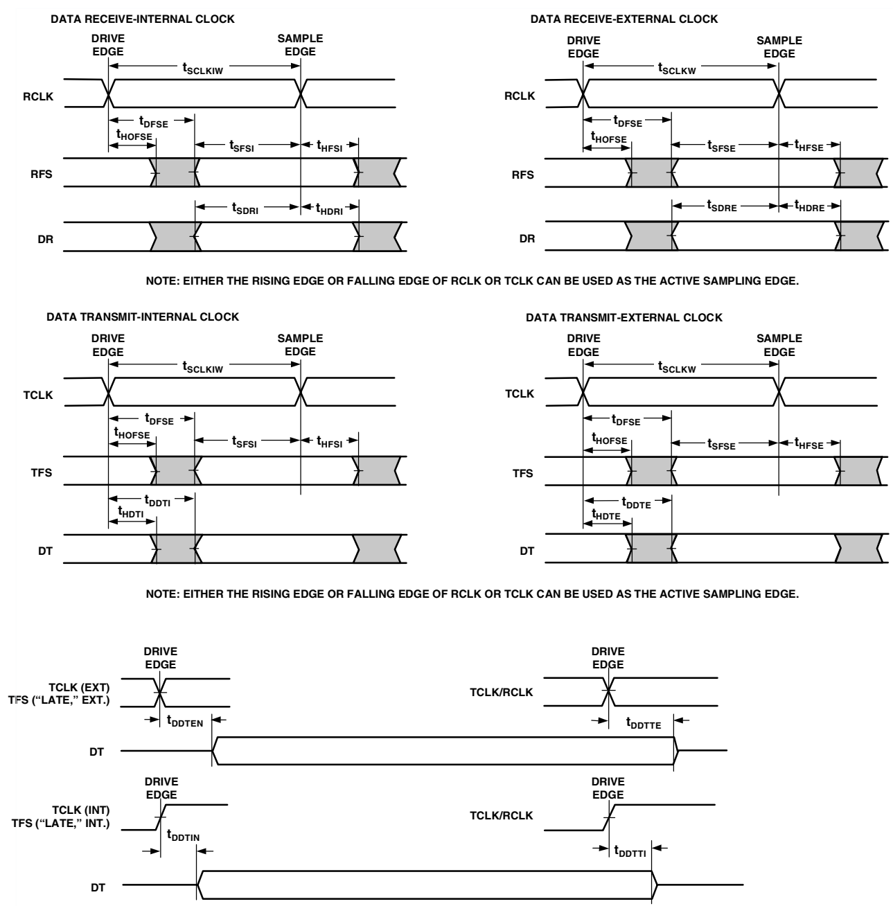
Figure 18. Serial Ports
