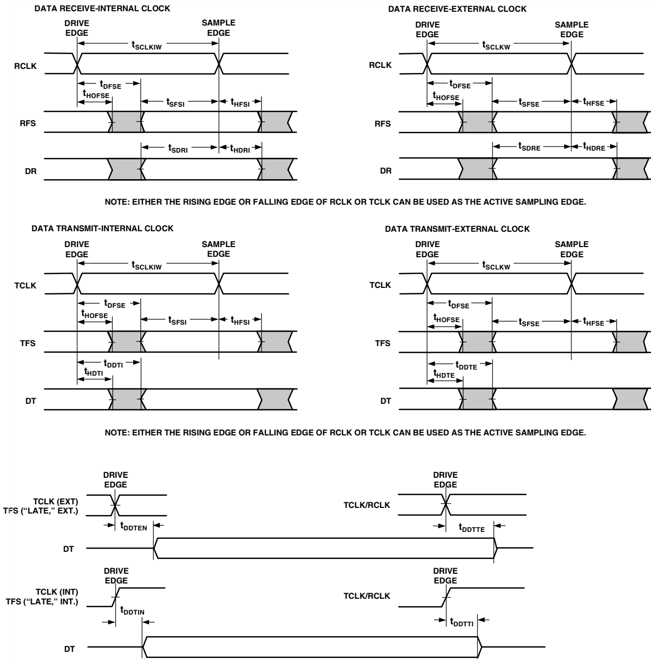
Figure 12. Serial Port
