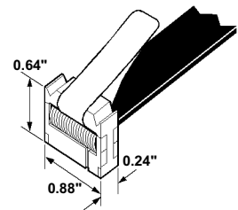
Figure 8. JTAG Pod Connector Dimensions
