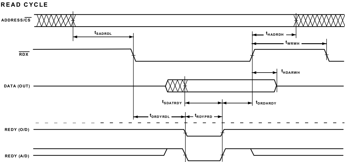
Figure 20. Read Cycle (Asynchronous Read—Host to ADSP-21160M)
