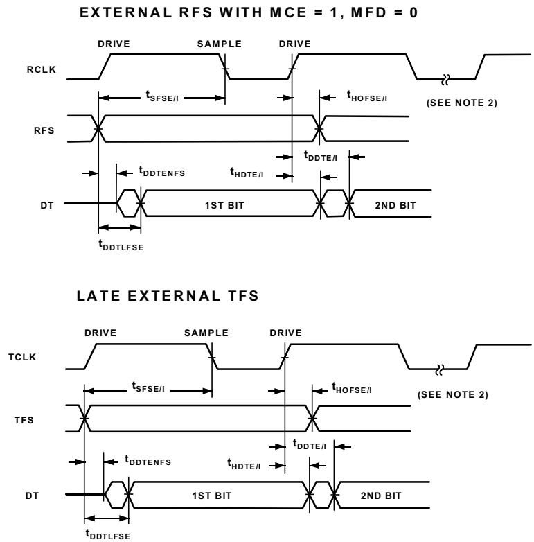
Figure 27. External Late Frame Sync
