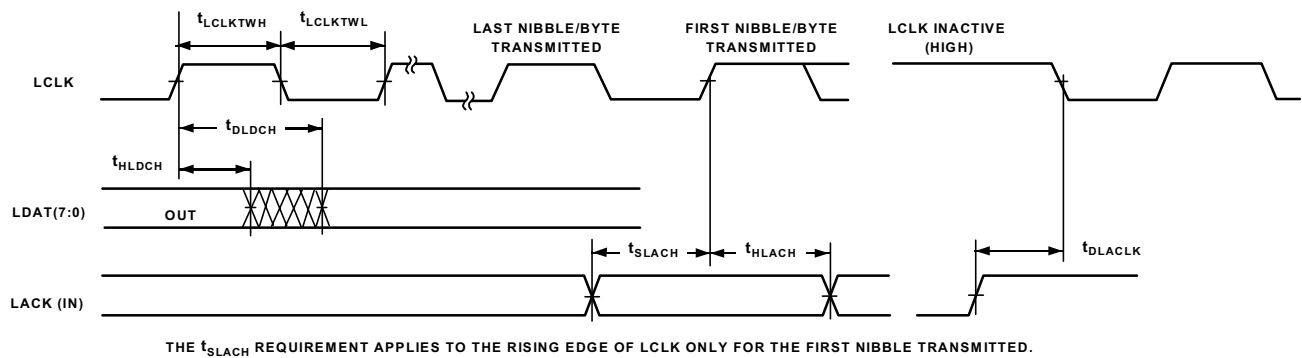
Figure 25. Link Ports—Transmit
