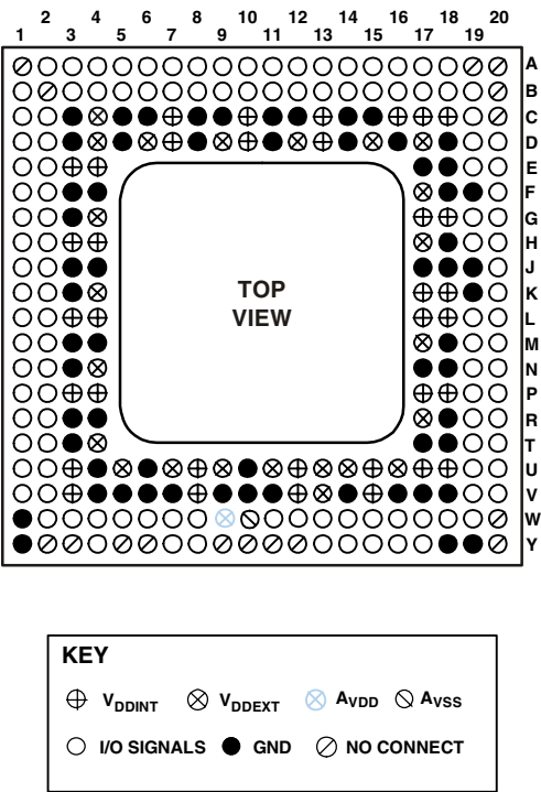
Figure 44. 256-Ball SBGA Ball Configuration (Top View)
