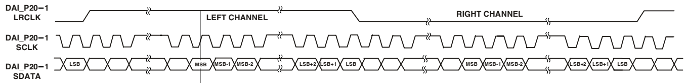
Figure 29. Right-Justified Mode
