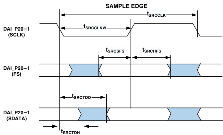
Figure 28. SRC Serial Output Port Timing
