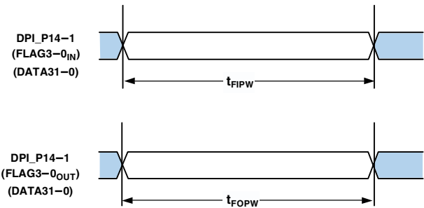
Figure 15. Flags
