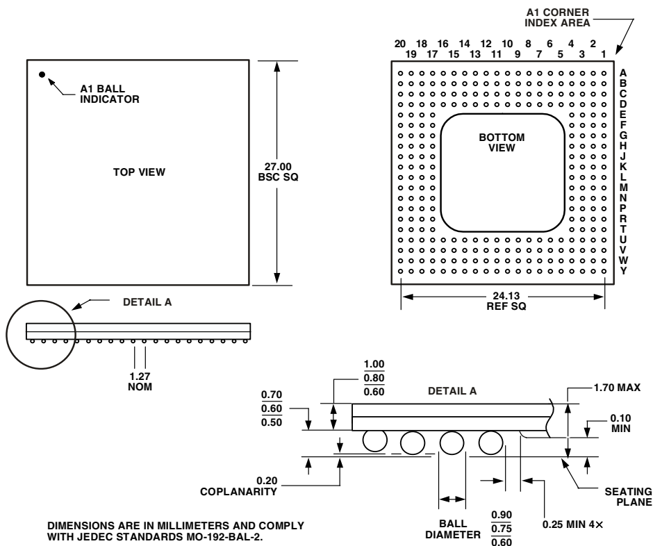
Figure 46. 256-Ball SBGA, Thermally Enhanced (BP-256)
