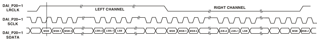
Figure 31. Left-Justified Mode
