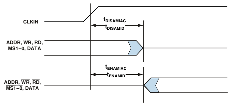
Figure 20. AMI Enable/Disable
