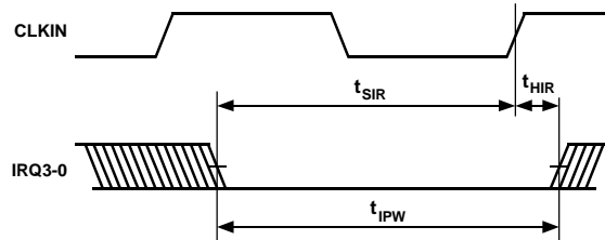
Figure 5. Interrupts
