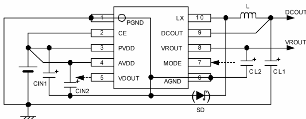
MSOP-10 (TOP VIEW)
