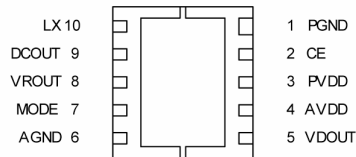
USP-10 (BOTTOM VIEW)
