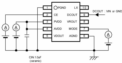
Circuit 1 Supply Current, Stand-by Current, CE Current, MODE Current
