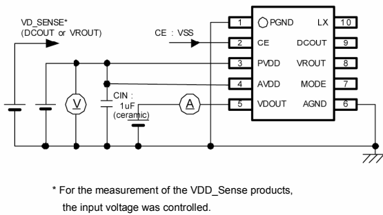
Circuit 9 VD Output Current
