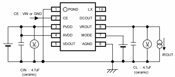
Circuit 2 Output Voltage (VR), Load Regulation, Dropout Voltage, Maximum Output Current, (MODE Voltage)
