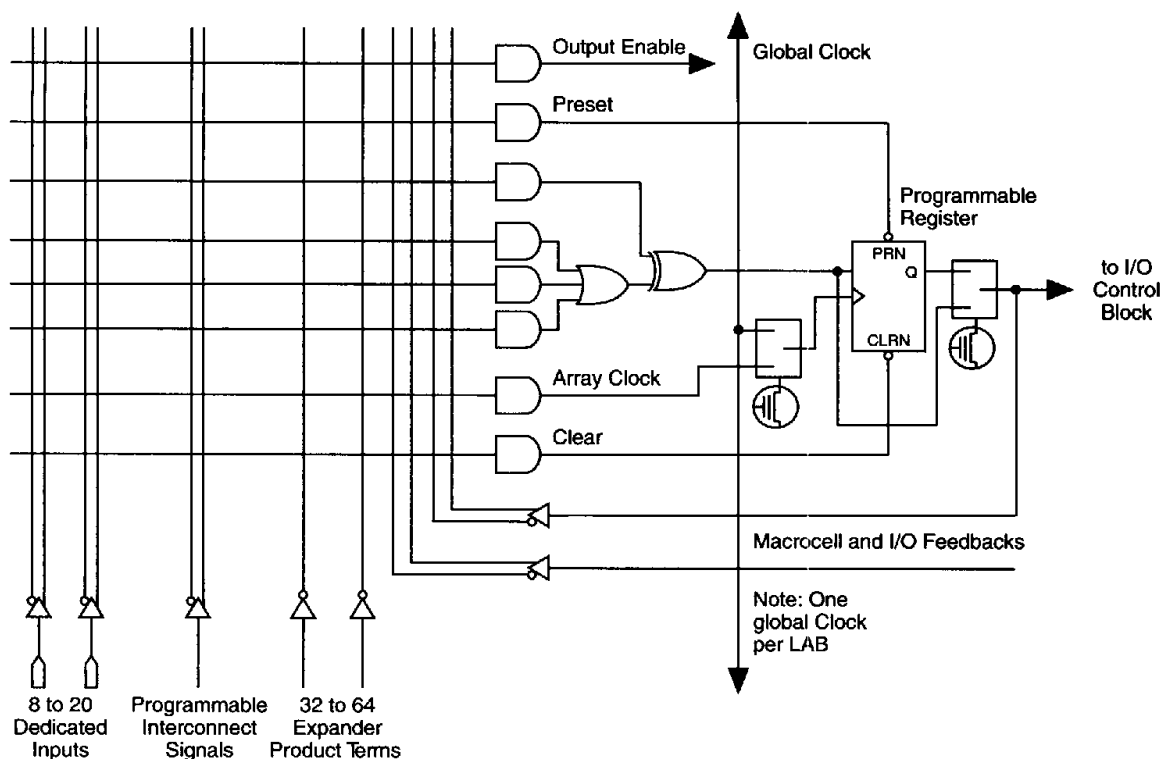
Figure 3. MAX 5000 Macrocell
