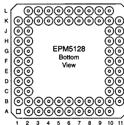
PGA
