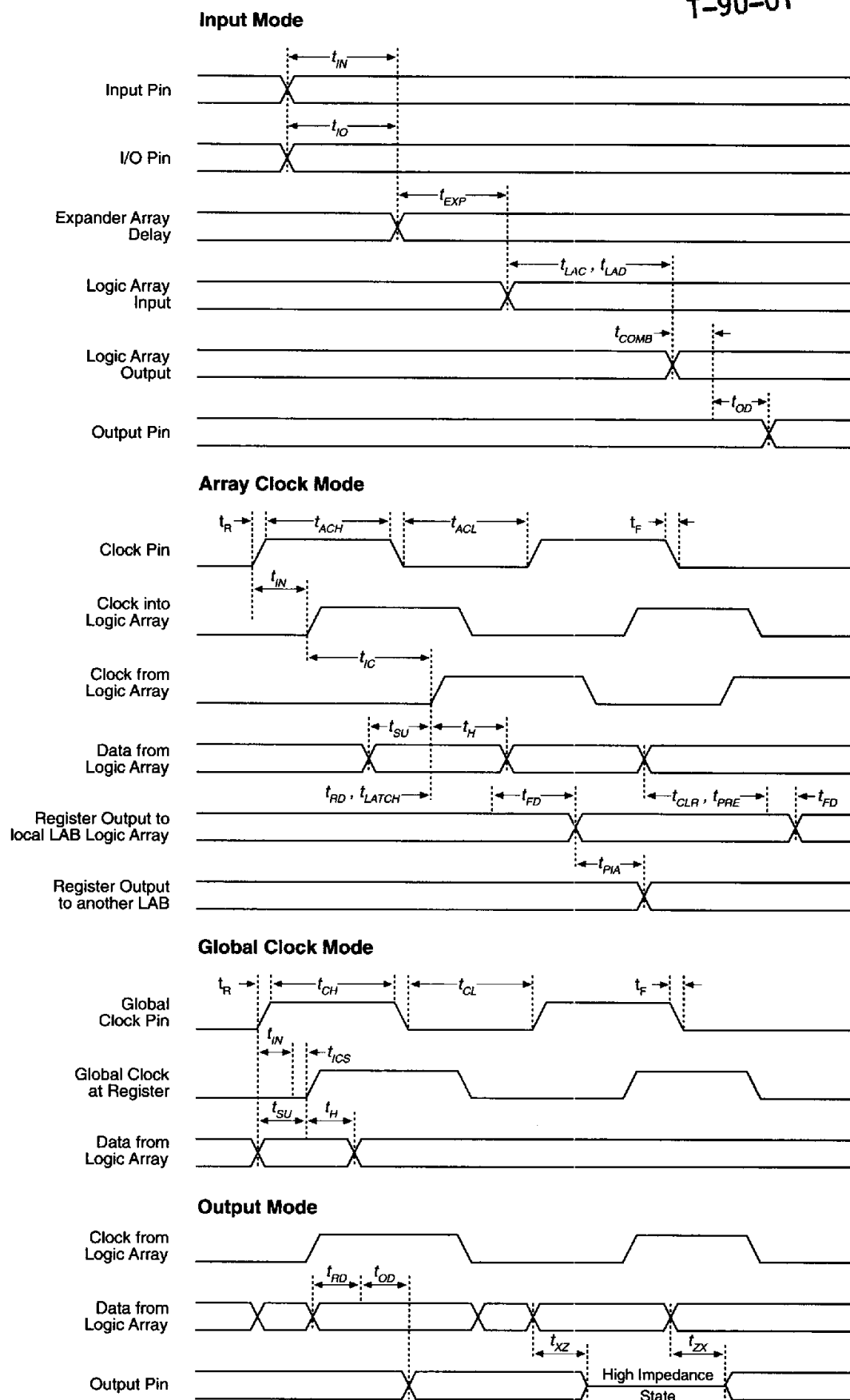
Figure 7. Switching Waveforms
