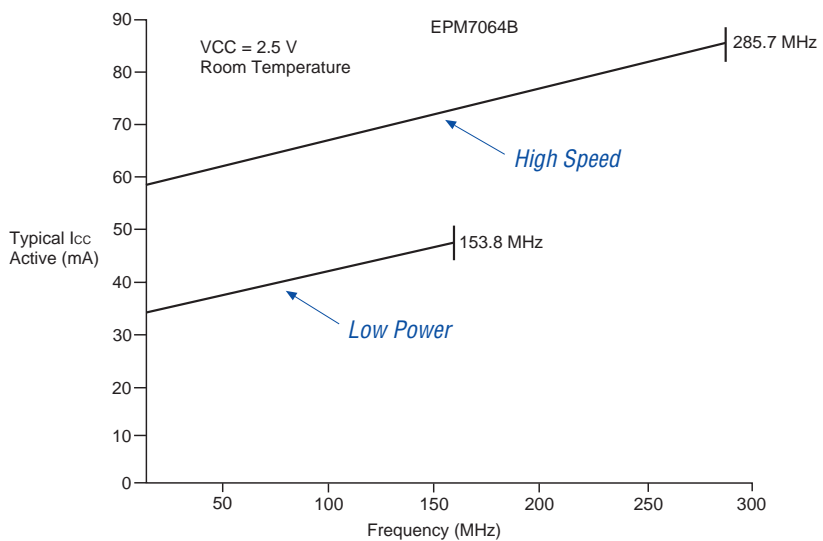
Figure 16. I_{CC} vs. Frequency for EPM7064B Devices
