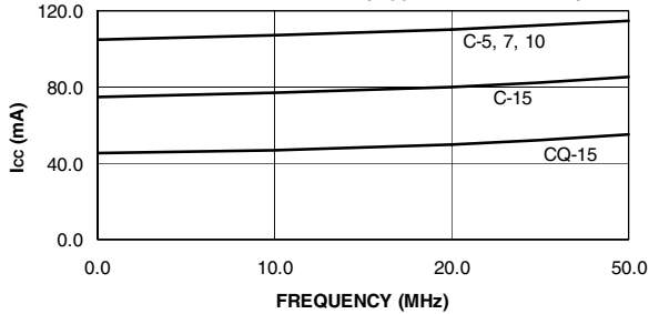
ATF22V10C/CQ SUPPLY CURRENT VS. INPUT FREQUENCY ( V_{CC} = 5\text{V} , T_A = 25^\circ\text{C} )
