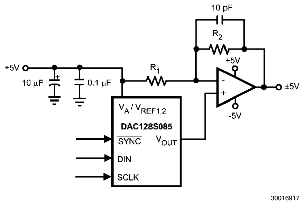
FIGURE 12. Bipolar Operation
