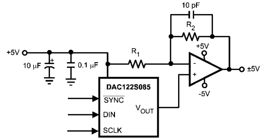
FIGURE 9. Bipolar Operation
