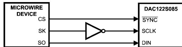
FIGURE 13. Microwire Interface
