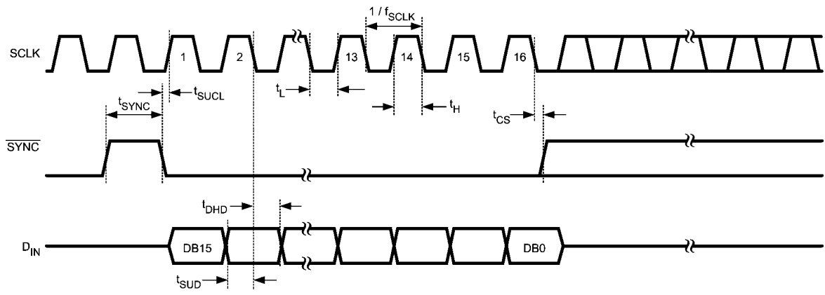
FIGURE 2. DAC121S101 Timing
