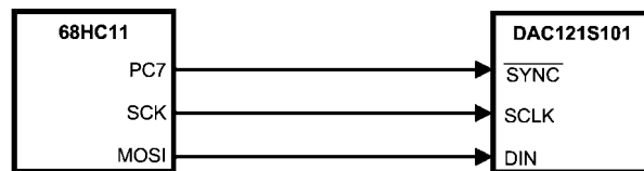
FIGURE 7. 68HC11 Interface
