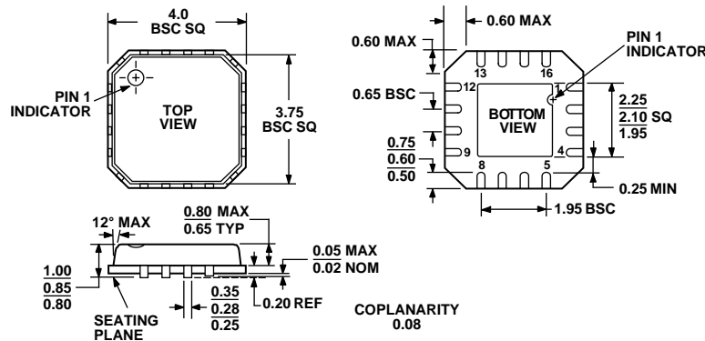
Figure 64. 16-Lead Lead Frame Chip Scale Package [LFCS] 4 mm x 4 mm Body (CP-16)
