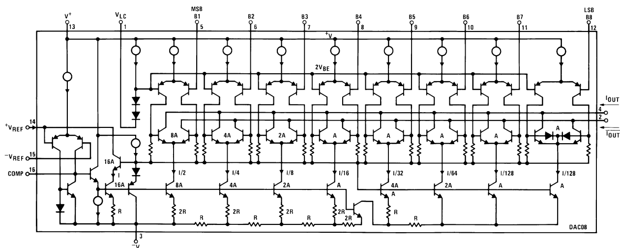
FIGURE 2. Equivalent Circuit
