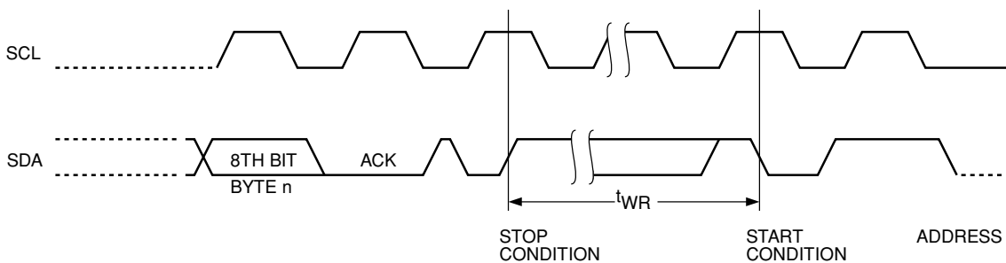
Figure 2. Write Cycle Timing
