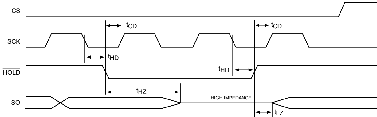
Figure 2. HOLD Timing
