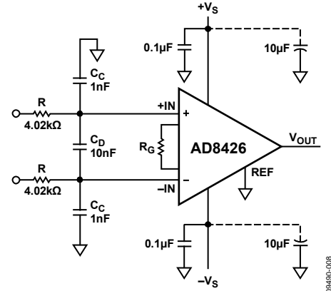
Figure 13. RFI Suppression
