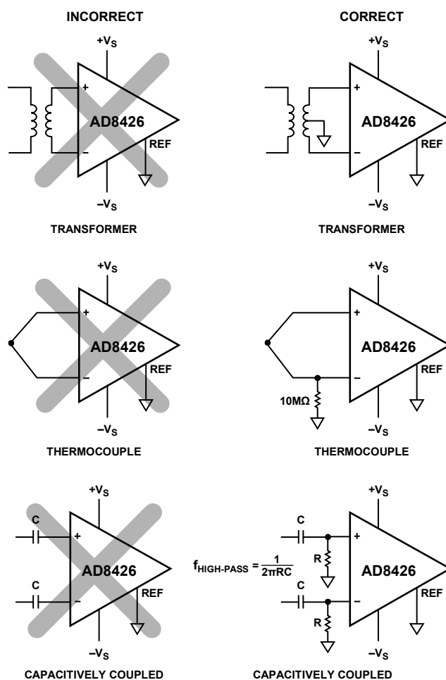
Figure 12. Creating an Input Bias Current Return Path
