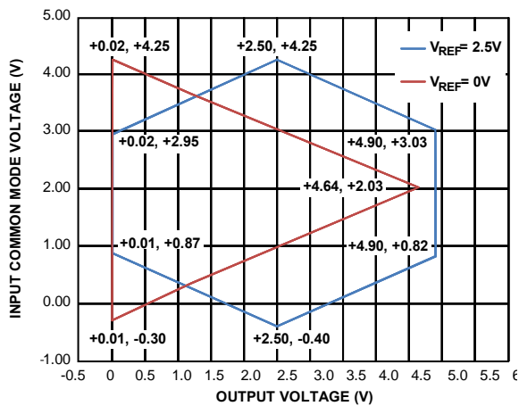
Figure 4. Input Common-Mode Voltage vs. Output Voltage, Single Supply, V_S = 5\text{ V} , G = 1
