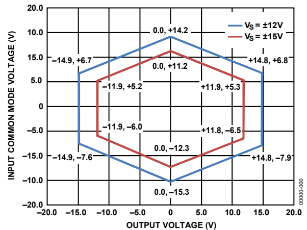
Figure 6. Input Common-Mode Voltage vs. Output Voltage, Dual Supply, V_S = \pm 15\text{ V} , G = 1
