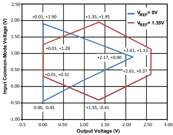
Figure 3. Input Common-Mode Voltage vs. Output Voltage, Single Supply, V_S = 2.7\text{ V} , G = 1
