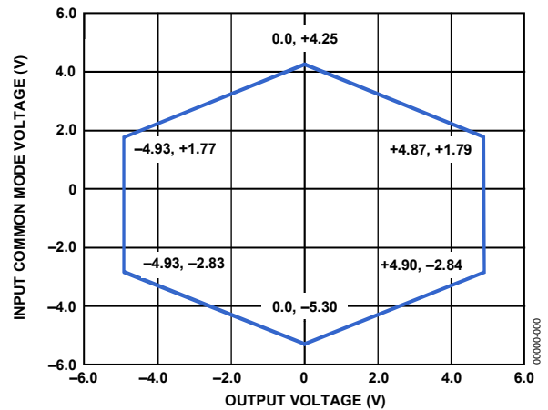
Figure 5. Input Common-Mode Voltage vs. Output Voltage, Dual Supply, V_S = \pm 5\text{ V} , G = 1
